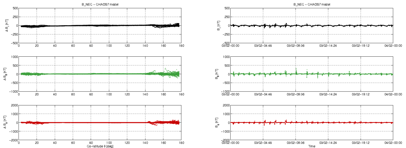
Figure 3-12: S/C C day 03/02: time series of B_{NEC} - B_{Chaos} residuals (right) and B_{NEC} - B_{Chaos} vs colatitude (left)
