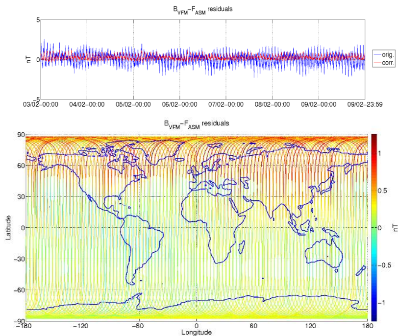
Figure 3-6: ASM-VFM residuals for S/C B, during monitoring period 03/02-09/02. In top figure are plotted: difference between |B_{VFM}| and F_{ASM} (without dB_{Sun} correction) (blue colour), and the residuals with dB_{Sun} corrections (red colour). In bottom figure residuals are presented on the world map.
