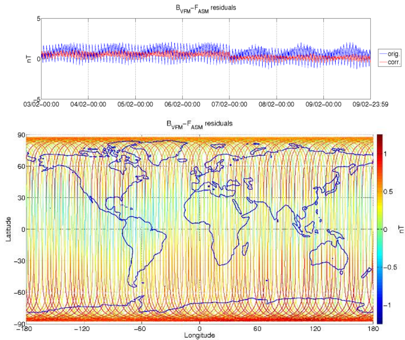
Figure 3-5: ASM-VFM residuals for S/C A, during monitoring period 03/02-09/02. In top figure are plotted: difference between |B_{VFM}| and F_{ASM} (without dB_{Sun} correction) (blue colour), and the residuals with dB_{Sun} corrections (red colour). In bottom figure residuals are presented on the world map.
