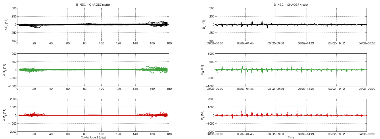
Figure 3-11: S/C B day 03/02: time series of B_{NEC} - B_{Chaos} residuals (right) and B_{NEC} - B_{Chaos} vs colatitude (left).
