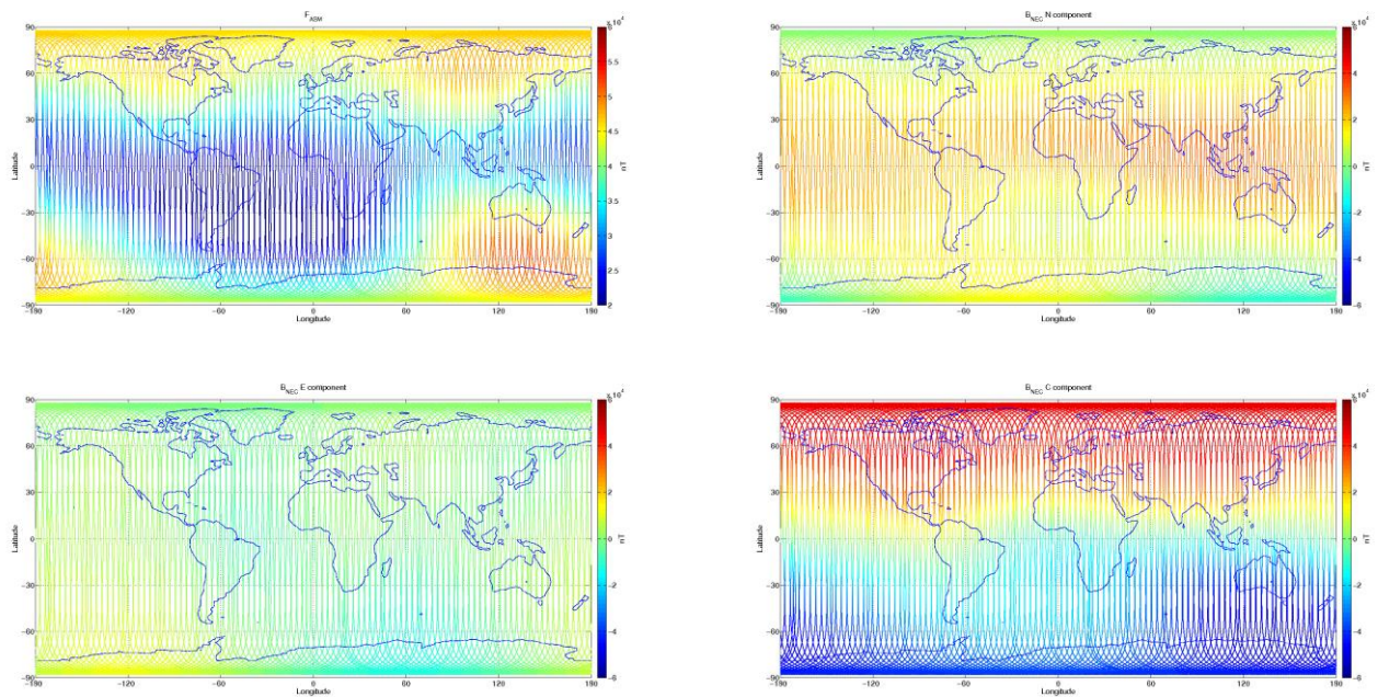
Figure 3-8: S/C B, world map plots of the geomagnetic field and components measured during monitoring period 27/01-02/02. From top to bottom: F-magnetic field from ASM measurement, B_{NEC} components (North, East, and Centre) of magnetic field from VFM measurement.
