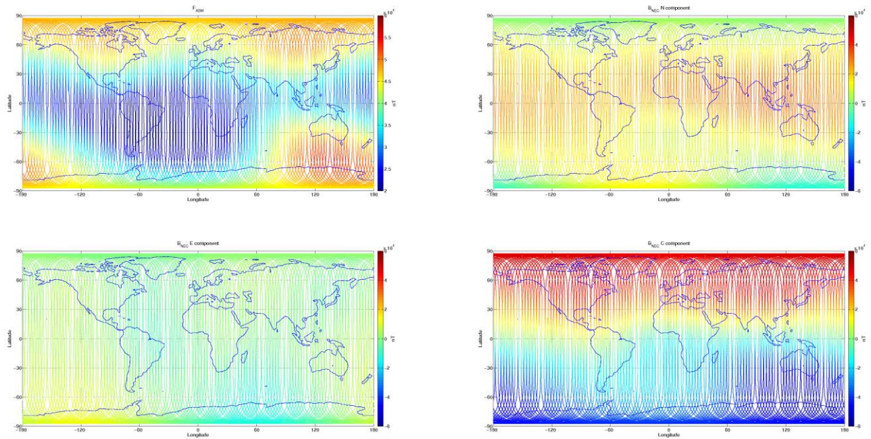
Figure 3-7: S/C A, world map plots of the geomagnetic field and components measured during monitoring period 27/01-02/02. From top to bottom: F-magnetic field from ASM measurement, B_{NEC} components (North, East, and Centre) of magnetic field from VFM measurement.
