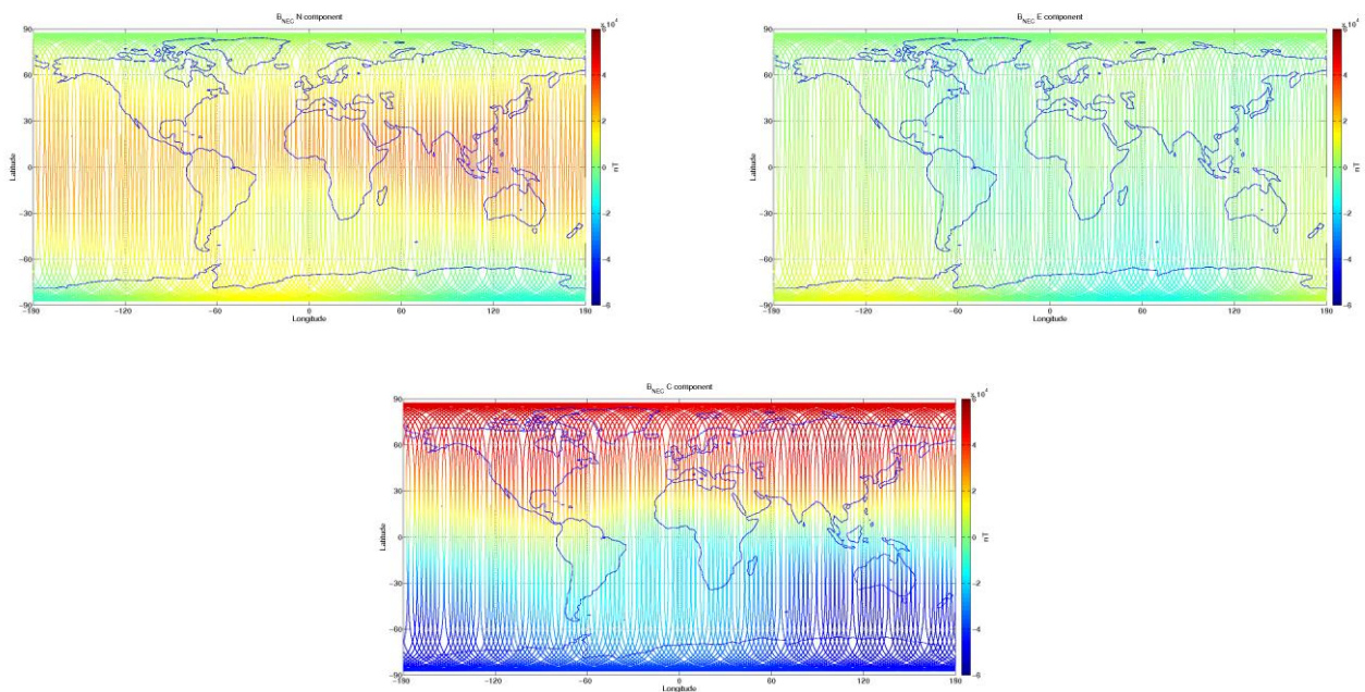
Figure 3-9: S/C C, world map plots of the geomagnetic field and components measured during monitoring period 27/01-02/02. From top to bottom: B_{NEC} components (North, East, and Centre) of magnetic field from VFM measurement.
