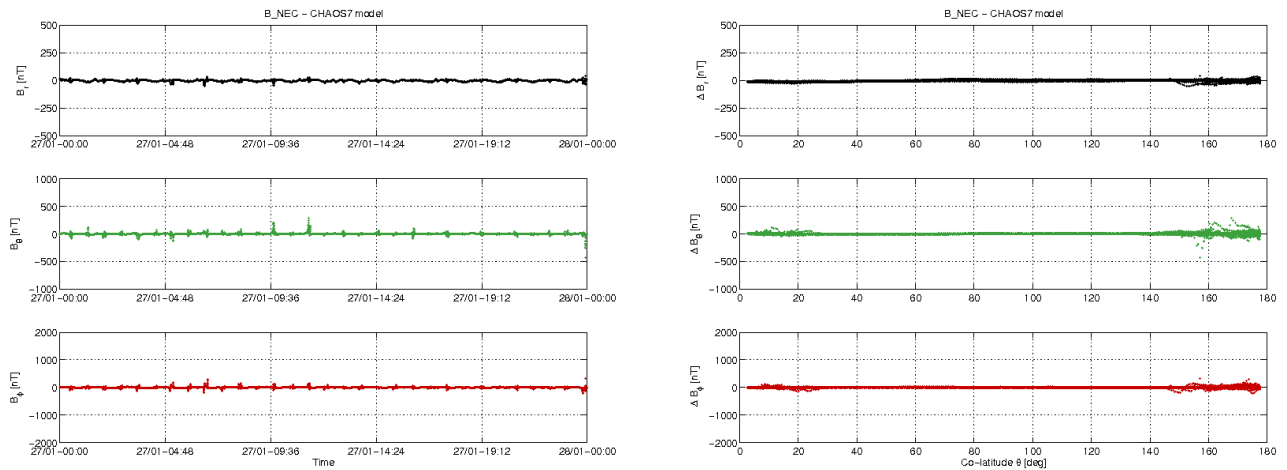
Figure 3-10: S/C A day 27/01: time series of B_{NEC} - B_{Chaos} residuals (left) and B_{NEC} - B_{Chaos} vs colatitude (right).
