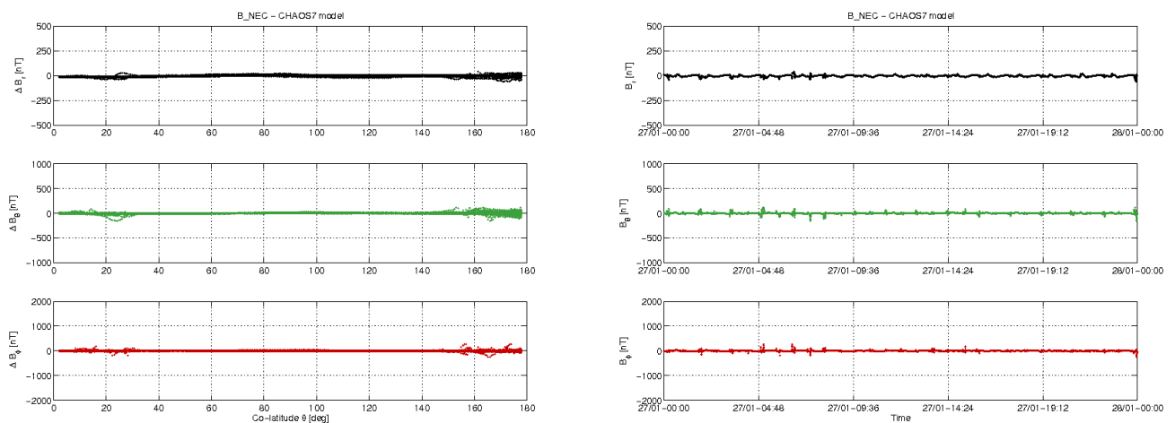
Figure 3-11: S/C B day 27/01: time series of B_{NEC} - B_{Chaos} residuals (left) and B_{NEC} - B_{Chaos} vs colatitude (right).
