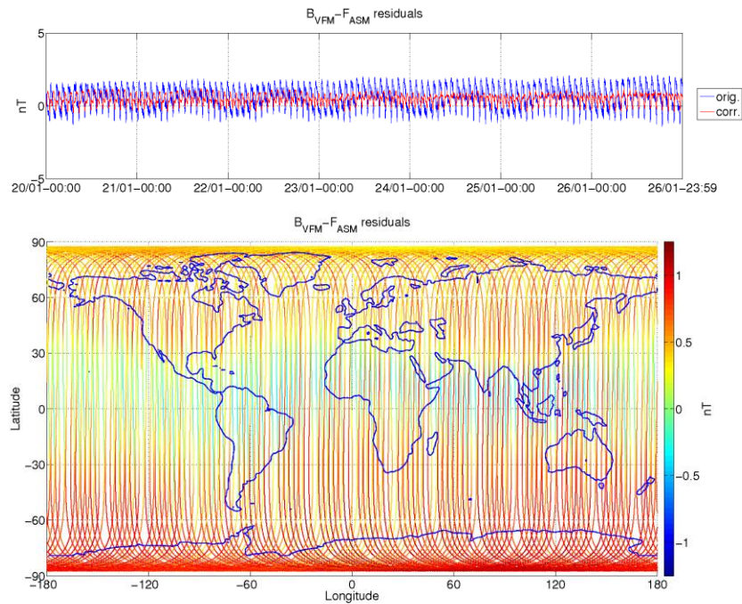
Figure 3-5: ASM-VFM residuals for S/C A, during monitoring period 20/01-26/01. In top figure are plotted: difference between |B_{VFM}| and F_{ASM} (without dB_{Sun} correction) (blue colour), and the residuals with dB_{Sun} corrections (red colour). In bottom figure residuals are presented on the world map.
