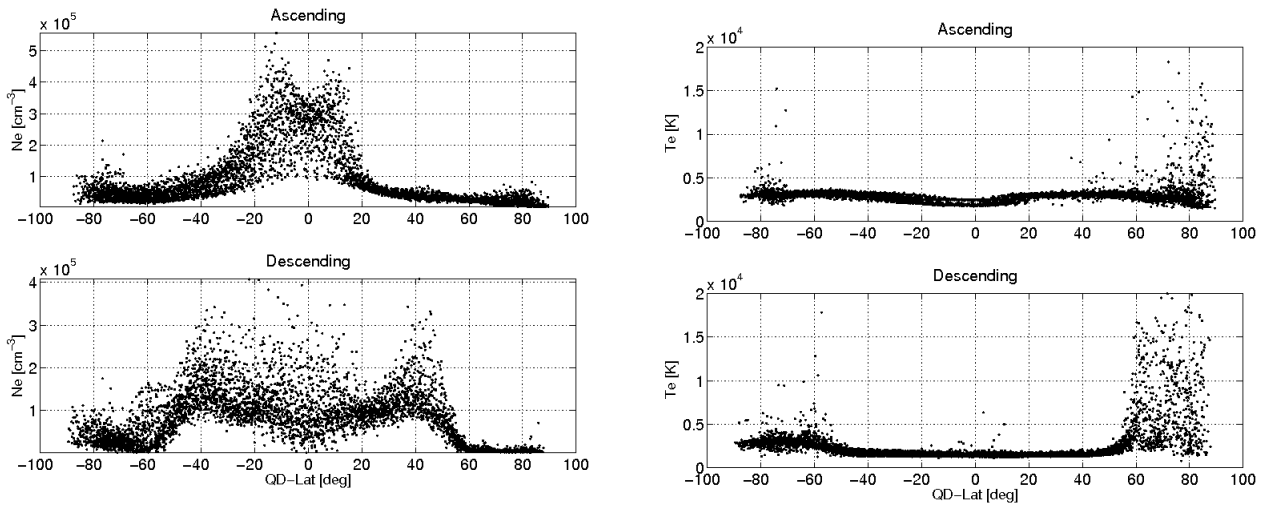
Figure 3-17: The panels show the electron density (left) and temperature (right) profile as a function of QD Latitudes for the last week of operation. The analysis is made separately for ascending (upper panels) and descending (bottom panels) orbits.
