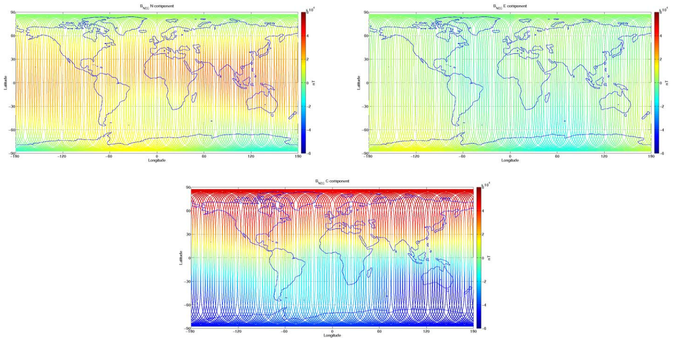
Figure 3-9: S/C C, world map plots of the geomagnetic field and components measured during monitoring period 20/01-26/01. From top to bottom: B_{NEC} components (North, East, and Centre) of magnetic field from VFM measurement
