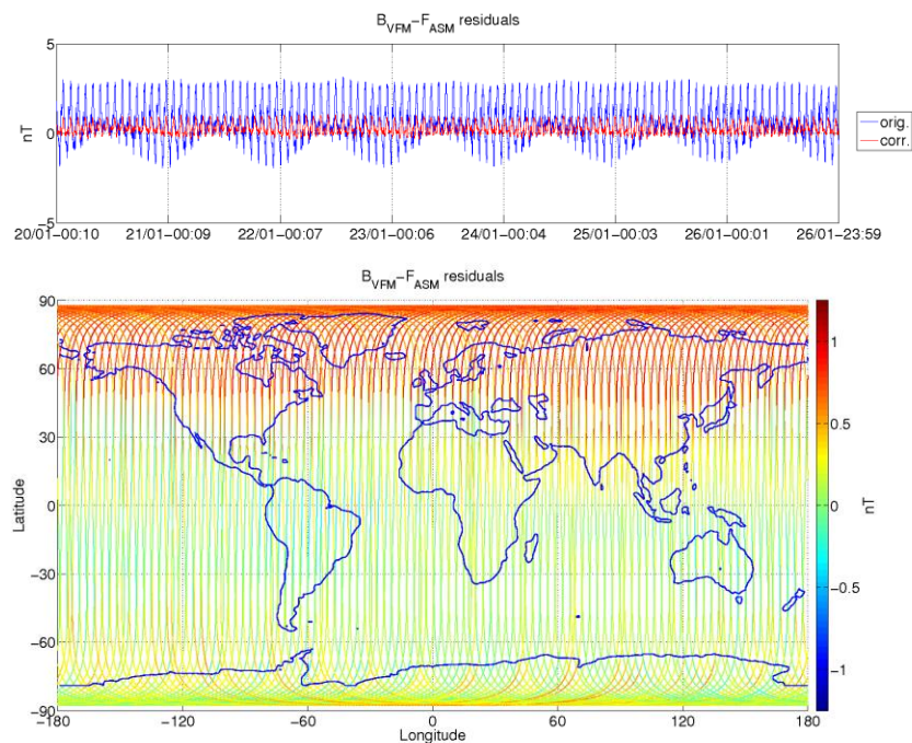
Figure 3-6: ASM-VFM residuals for S/C B, during monitoring period 20/01-26/01. In top figure are plotted: difference between |B_{VFM}| and F_{ASM} (without dB_Sun correction) (blue colour), and the residuals with dB_Sun corrections (red colour). In bottom figure residuals are presented on the world map.
