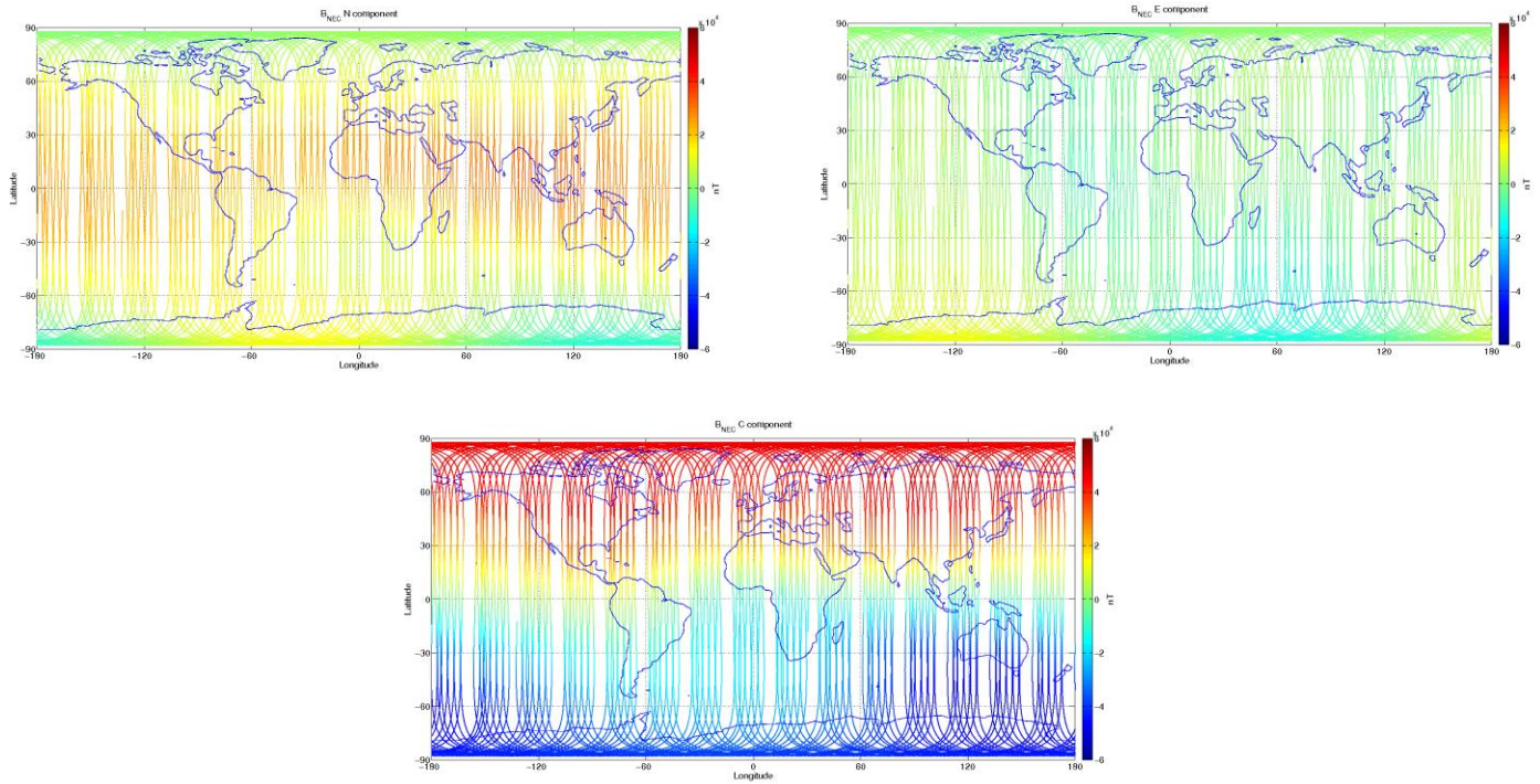
Figure 3-7: S/C B, world map plots of the geomagnetic field and components measured during monitoring period 13/01-19/01. From top to bottom: B_{NEC} components (North, East, and Centre) of magnetic field from VFM measurement.
