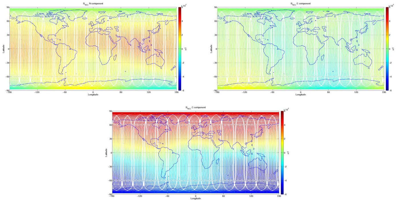
Figure 3-8: S/C C, world map plots of the geomagnetic field and components measured during monitoring period 13/01-19/01. From top to bottom: B_{NEC} components (North, East, and Centre) of magnetic field from VFM measurement.
