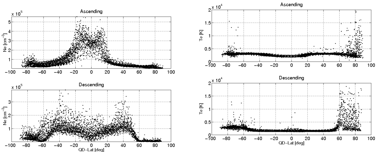
Figure 3-16: The panels shown the electron density (left) and temperature (right) profile as a function of QD Latitudes for the last week of operation. The analysis is made separately for ascending (upper panels) and descending (bottom panels) orbits.
