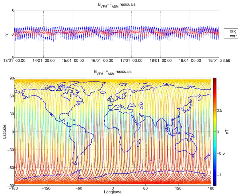
Figure 3-5 : ASM-VFM residuals for S/C A, during monitoring period 13/01-19/01. In top figure are plotted: difference between |B_{VFM}| and F_{ASM} (without dB Sun correction) (blue colour), and the residuals with dB Sun corrections (red colour). In bottom figure residuals are presented on the world map.
