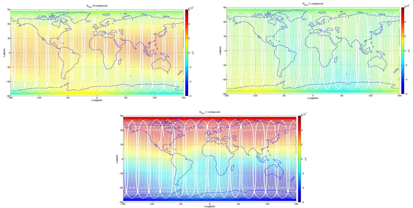
Figure 3-9: S/C C, world map plots of the geomagnetic field and components measured during monitoring period 06/01-12/01. From top to bottom: B_{NEC} components (North, East, and Centre) of magnetic field from VFM measurement
