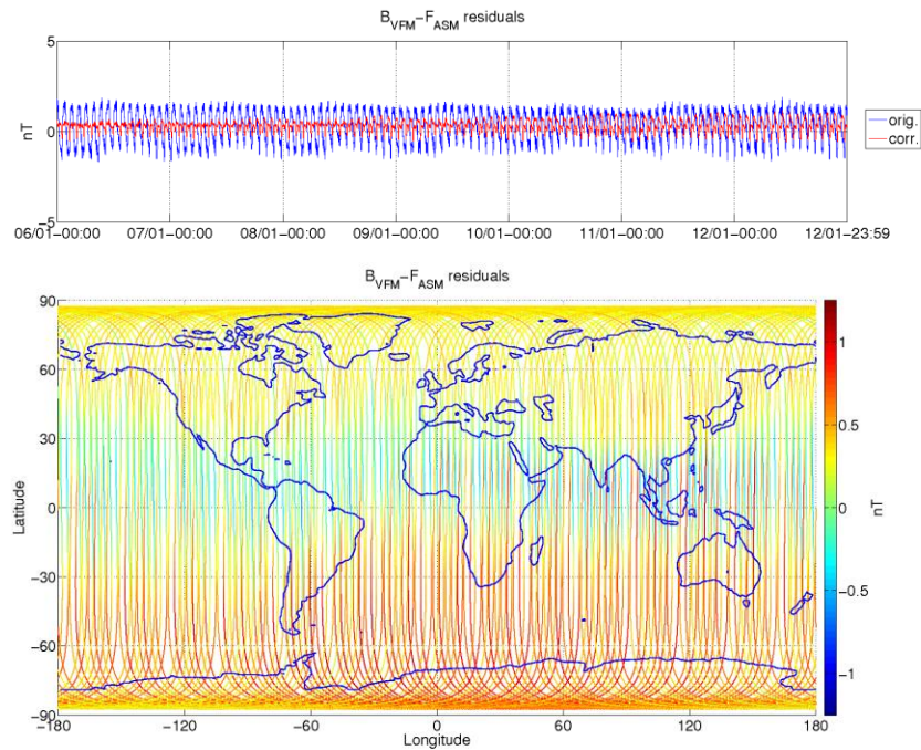
Figure 3-5: ASM-VFM residuals for S/C A, during monitoring period 06/01-12/01. In top figure are plotted: difference between |B_{VFM}| and F_{ASM} (without dB_{Sun} correction) (blue colour), and the residuals with dB_{Sun} corrections (red colour). In bottom figure residuals are presented on the world map.
