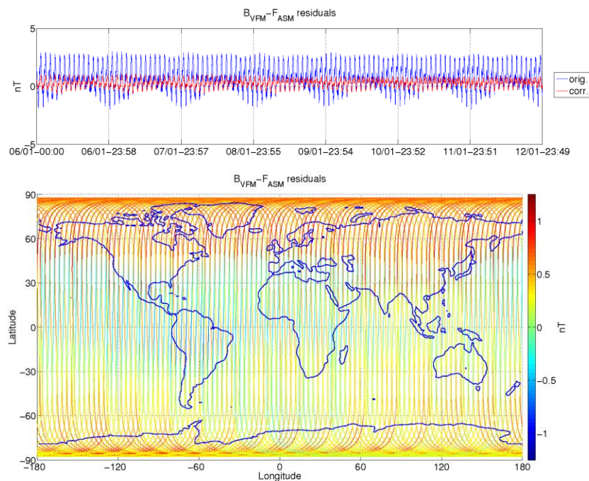
Figure 3-6: ASM-VFM residuals for S/C B, during monitoring period 06/01-12/01. In top figure are plotted: difference between |B_{VFM}| and F_{ASM} (without dB_{Sun} correction) (blue colour), and the residuals with dB_{Sun} corrections (red colour). In bottom figure residuals are presented on the world map.
