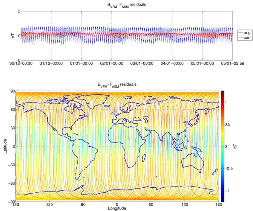
Figure 3-5: ASM-VFM residuals for S/C A, during monitoring period 30/12-05/01. In top figure are plotted: difference between |B_{VFM}| and F_{ASM} (without dB_{Sun} correction) (blue colour), and the residuals with dB_{Sun} corrections (red colour). In bottom figure residuals are presented on the world map.
