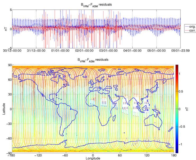
Figure 3-6: ASM-VFM residuals for S/C B, during monitoring period 30/12-05/01. In top figure are plotted: difference between |B_{VFM}| and F_{ASM} (without dB_Sun correction) (blue colour), and the residuals with dB_Sun corrections (red colour). In bottom figure residuals are presented on the world map.
