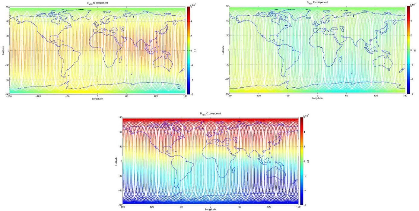
Figure 3-9: S/C C, world map plots of the geomagnetic field and components measured during monitoring period 23/12-29/12. From top to bottom: B_{NEC} components (North, East, and Centre) of magnetic field from VFM measurement
