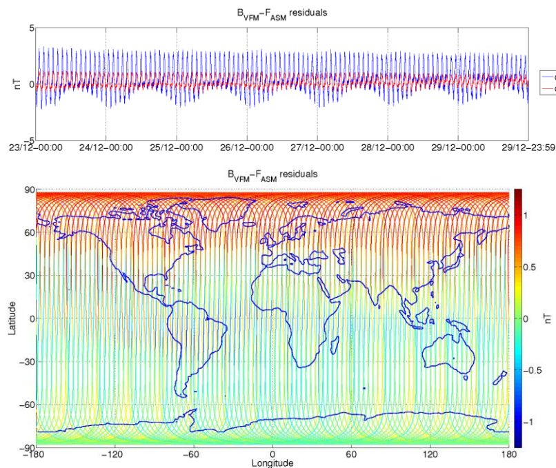
Figure 3-6: ASM-VFM residuals for S/C B, during monitoring period 23/12-29/12. In top figure are plotted: difference between |B_{VFM}| and F_{ASM} (without dB_Sun correction) (blue colour), and the residuals with dB_Sun corrections (red colour). In bottom figure residuals are presented on the world map.
