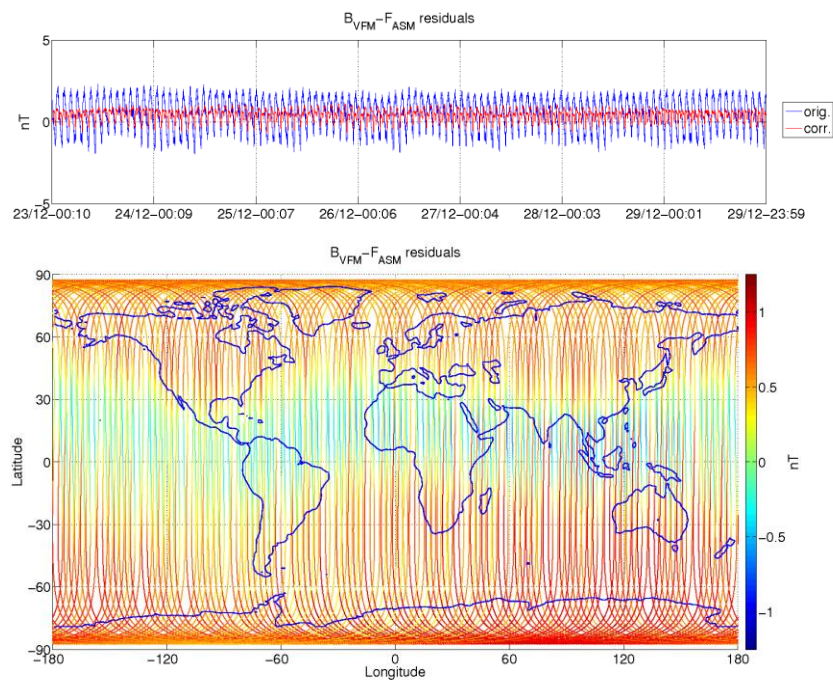
Figure 3-5: ASM-VFM residuals for S/C A, during monitoring period 23/12-29/12. In top figure are plotted: difference between |B_{VFM}| and F_{ASM} (without dB_{Sun} correction) (blue colour), and the residuals with dB_{Sun} corrections (red colour). In bottom figure residuals are presented on the world map.
