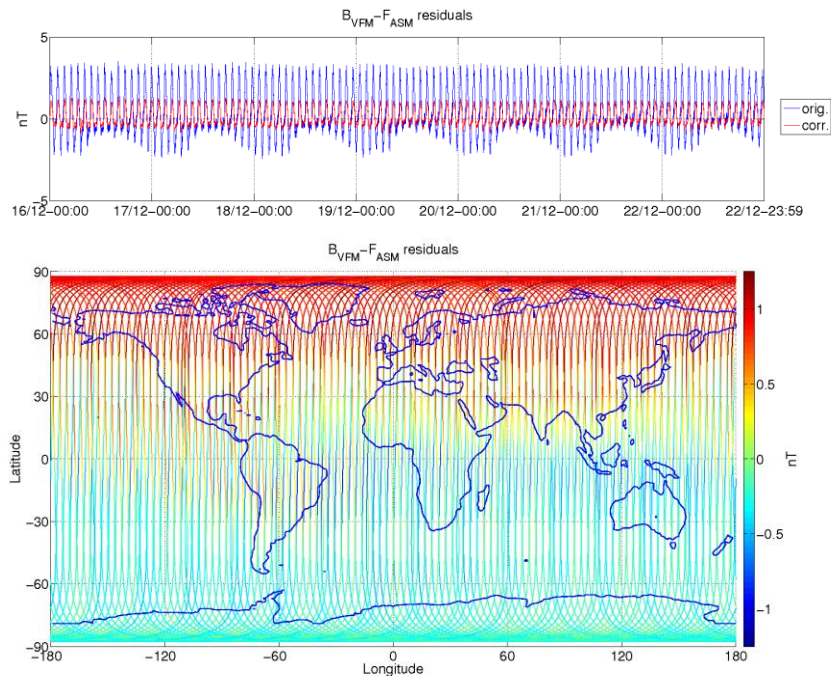
Figure 3-5: ASM-VFM residuals for S/C B, during monitoring period 16/12-22/12. In top figure are plotted: difference between |B_{VFM}| and F_{ASM} (without dB_{Sun} correction) (blue colour), and the residuals with dB_{Sun} corrections (red colour). In bottom figure residuals are presented on the world map.
