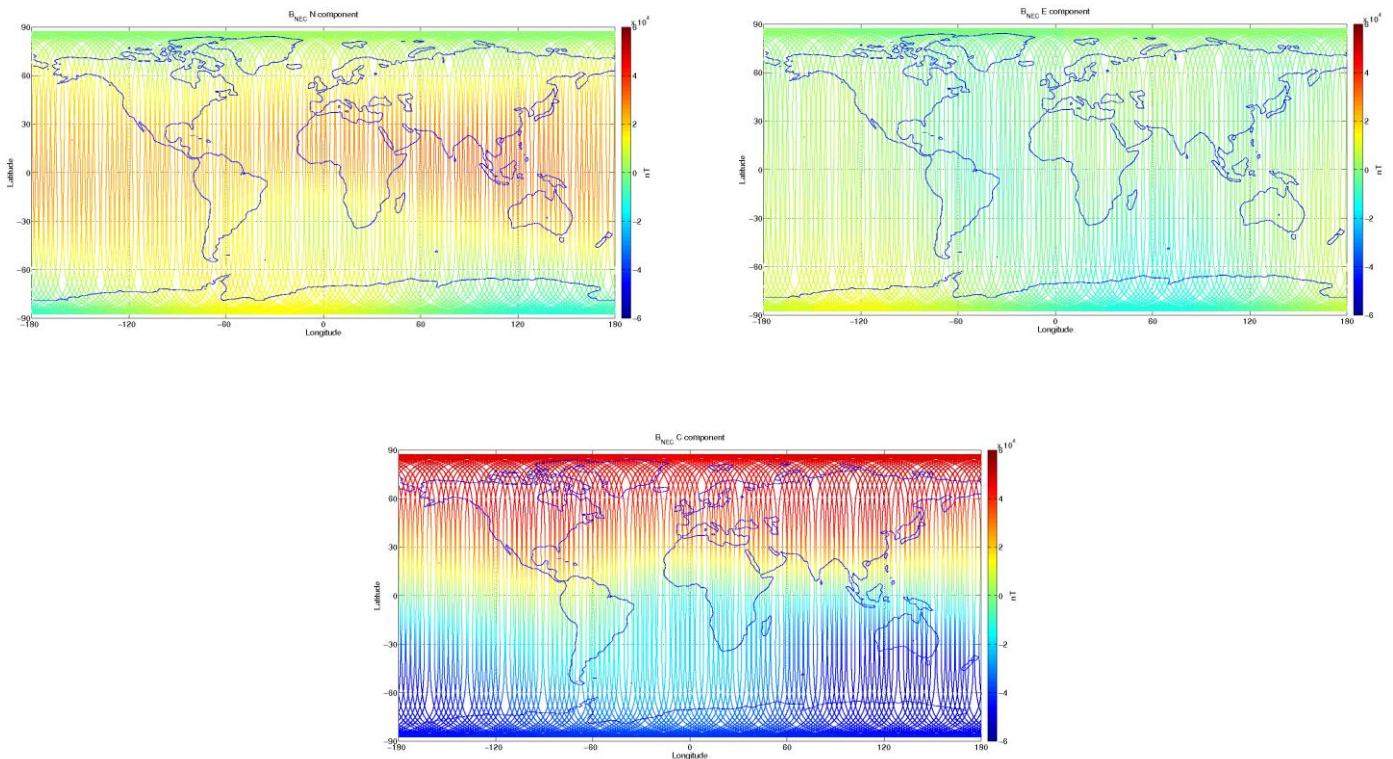
Figure 3-9: S/C C, world map plots of the geomagnetic field and components measured during monitoring period 09/12-15/12. From top to bottom: B_{NEC} components (North, East, and Centre) of magnetic field from VFM measurement
