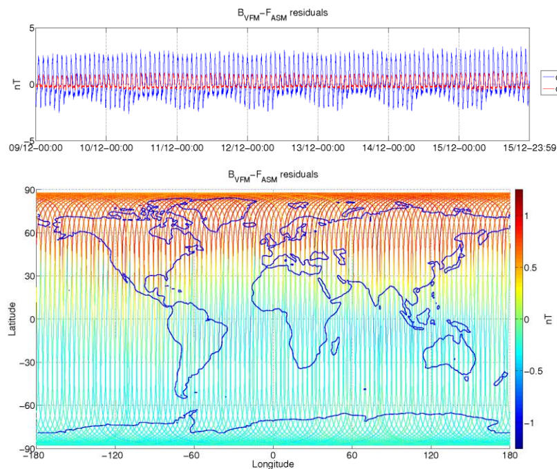
Figure 3-6: ASM-VFM residuals for S/C B, during monitoring period 09/12-15/12. In top figure are plotted: difference between |B_{VFM}| and F_{ASM} (without dB_{Sun} correction) (blue colour), and the residuals with dB_{Sun} corrections (red colour). In bottom figure residuals are presented on the world map.
