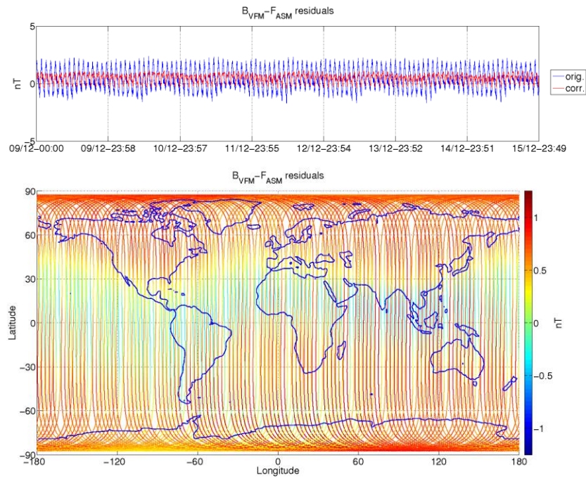
Figure 3-5: ASM-VFM residuals for S/C A, during monitoring period 09/12-15/12. In top figure are plotted: difference between |B_{VFM}| and F_{ASM} (without dB_{Sun} correction) (blue colour), and the residuals with dB_{Sun} corrections (red colour). In bottom figure residuals are presented on the world map.
