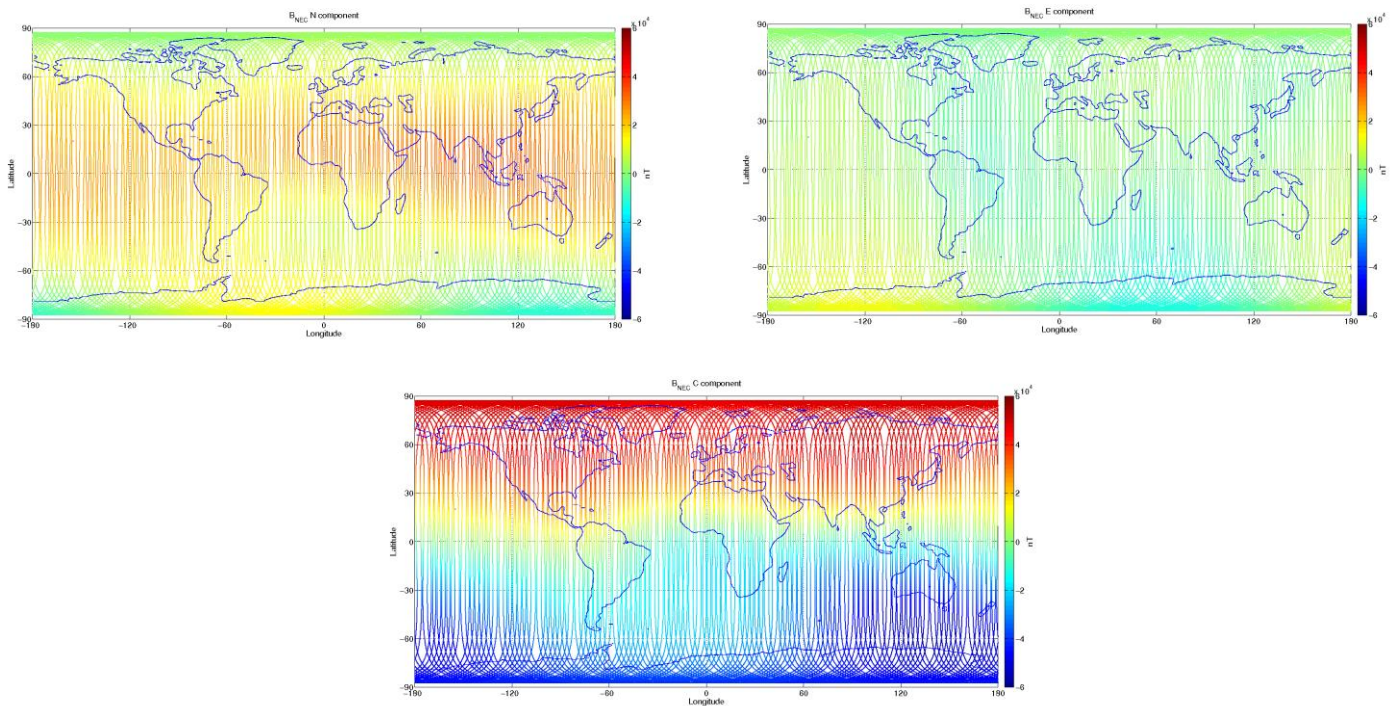
Figure 3-9: S/C C, world map plots of the geomagnetic field and components measured during monitoring period 02/12-08/12. From top to bottom: B_{NEC} components (North, East, and Centre) of magnetic field from VFM measurement
