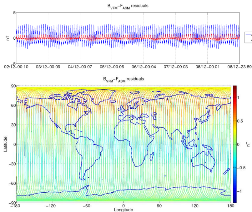
Figure 3-6: ASM-VFM residuals for S/C B, during monitoring period 02/12-08/12. In top figure are plotted: difference between |B_{VFM}| and F_{ASM} (without dB Sun correction) (blue colour), and the residuals with dB Sun corrections (red colour). In bottom figure residuals are presented on the world map.
