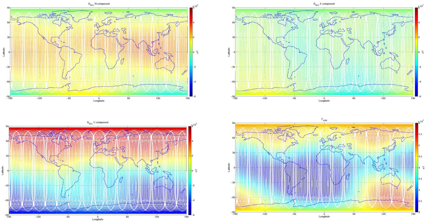
Figure 3-7: S/C A, world map plots of the geomagnetic field and components measured during monitoring period 02/12-08/12. From top to bottom: B_{NEC} components (North, East, and Centre) of magnetic field from VFM measurement, F_{ASM} magnetic field from ASM measurement.
