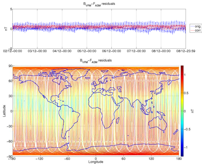
Figure 3-5: ASM-VFM residuals for S/C A, during monitoring period 02/12-08/12. In top figure are plotted: difference between |B VFM | and F ASM (without dB Sun correction) (blue colour), and the residuals with dB Sun corrections (red colour). In bottom figure residuals are presented on the world map.
