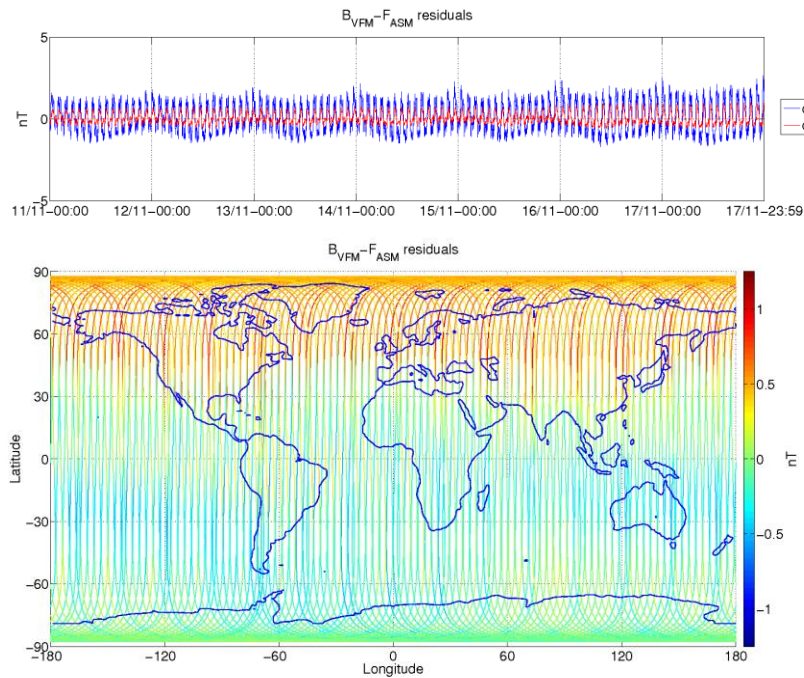
Figure 3-6: ASM-VFM residuals for S/C B, during monitoring period 11/11-17/11. In top figure are plotted: difference between |B_{VFM}| and F_{ASM} (without dB Sun correction) (blue colour), and the residuals with dB Sun corrections (red colour). In bottom figure residuals are presented on the world map.
