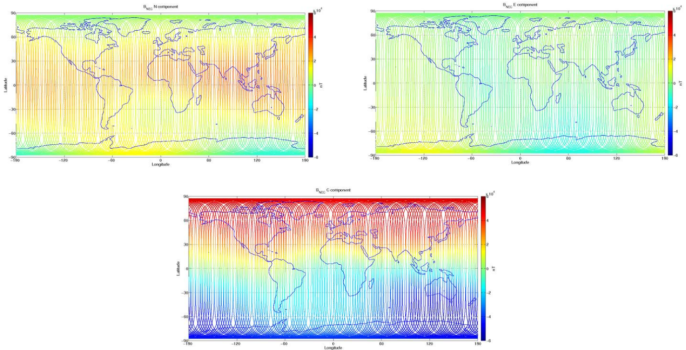
Figure 3-9: S/C C, world map plots of the geomagnetic field and components measured during monitoring period 11/11-17/11. From top to bottom: B_{NEC} components (North, East, and Centre) of magnetic field from VFM measurement
