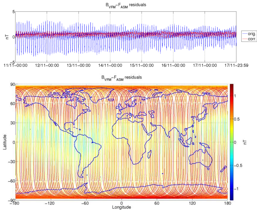
Figure 3-5: ASM-VFM residuals for S/C A, during monitoring period 11/11-17/11. In top figure are plotted: difference between |B_{VFM}| and F_{ASM} (without dB_{Sun} correction) (blue colour), and the residuals with dB_{Sun} corrections (red colour). In bottom figure residuals are presented on the world map.
