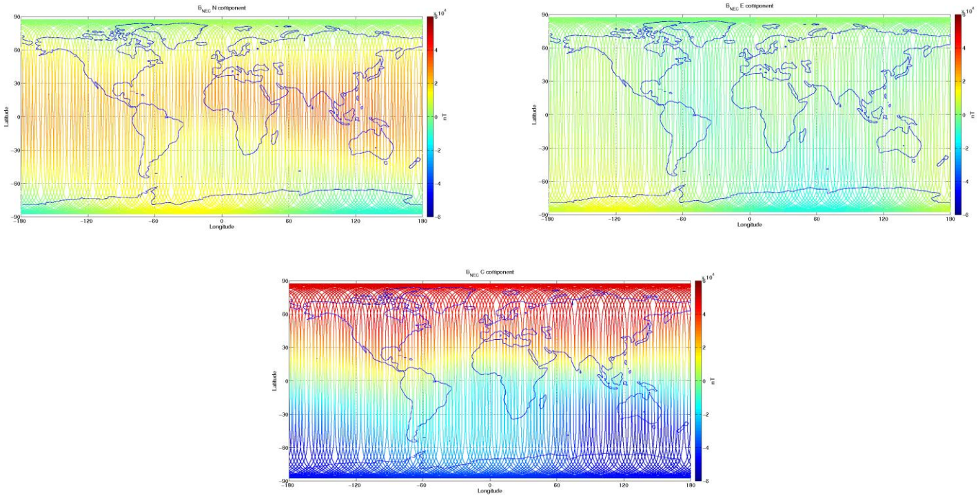
Figure 3-9: S/C C, world map plots of the geomagnetic field and components measured during monitoring period 04/11-10/11. From top to bottom: B_{NEC} components (North, East, and Centre) of magnetic field from VFM measurement
