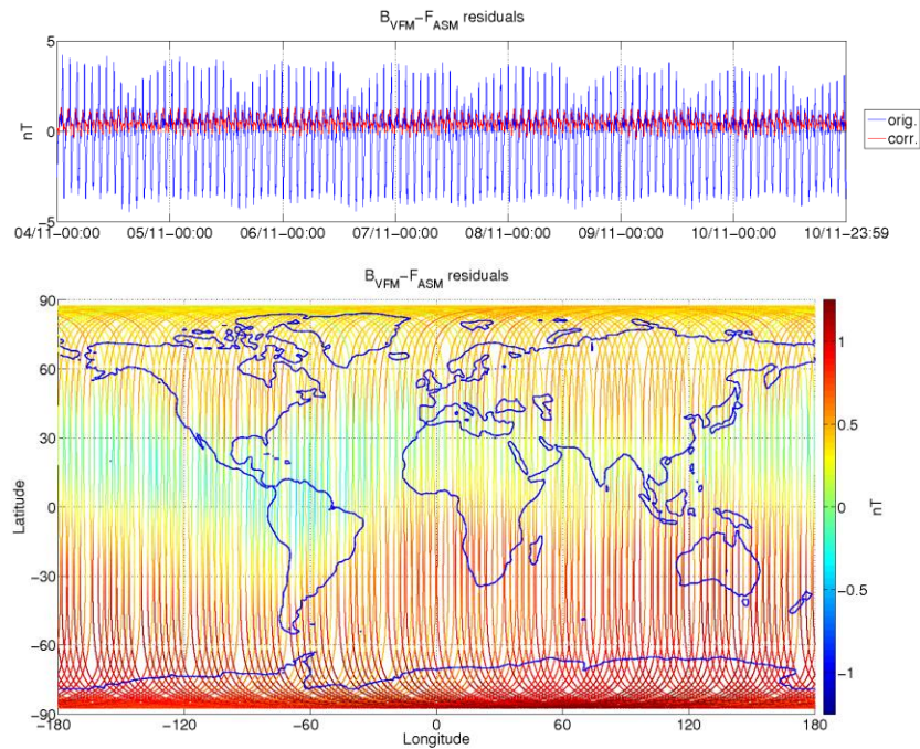
Figure 3-5: ASM-VFM residuals for S/C A, during monitoring period 04/11-10/11. In top figure are plotted: difference between |B_{VFM}| and F_{ASM} (without dB_{Sun} correction) (blue colour), and the residuals with dB_{Sun} corrections (red colour). In bottom figure residuals are presented on the world map.
