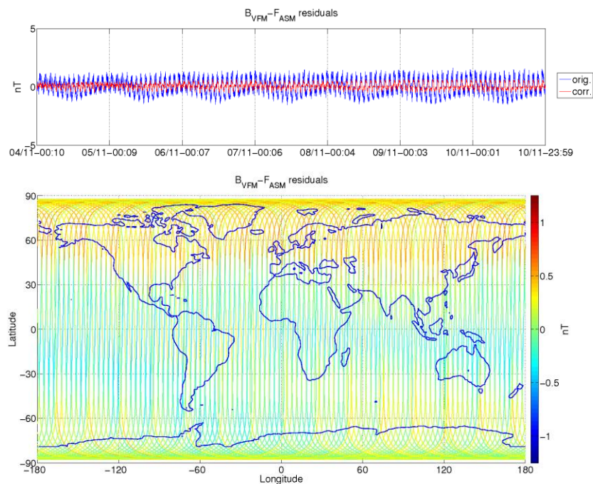
Figure 3-6: ASM-VFM residuals for S/C B, during monitoring period 04/11-10/11. In top figure are plotted: difference between |B_{VFM}| and F_{ASM} (without dB Sun correction) (blue colour), and the residuals with dB Sun corrections (red colour). In bottom figure residuals are presented on the world map.
