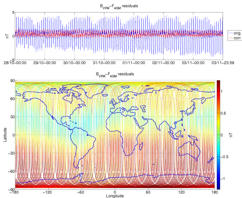
Figure 3-5: ASM-VFM residuals for S/C A, during monitoring period 28/10-03/11. In top figure are plotted: difference between |B_{VFM}| and F_{ASM} (without dB_{Sun} correction) (blue colour), and the residuals with dB_{Sun} corrections (red colour). In bottom figure residuals are presented on the world map.
