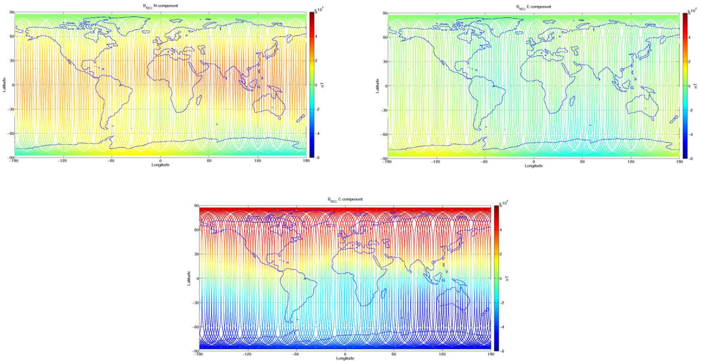
Figure 3-8: S/C C, world map plots of the geomagnetic field and components measured during monitoring period 28/10-03/11. From top to bottom: B_{NEC} components (North, East, and Centre) of magnetic field from VFM measurement
