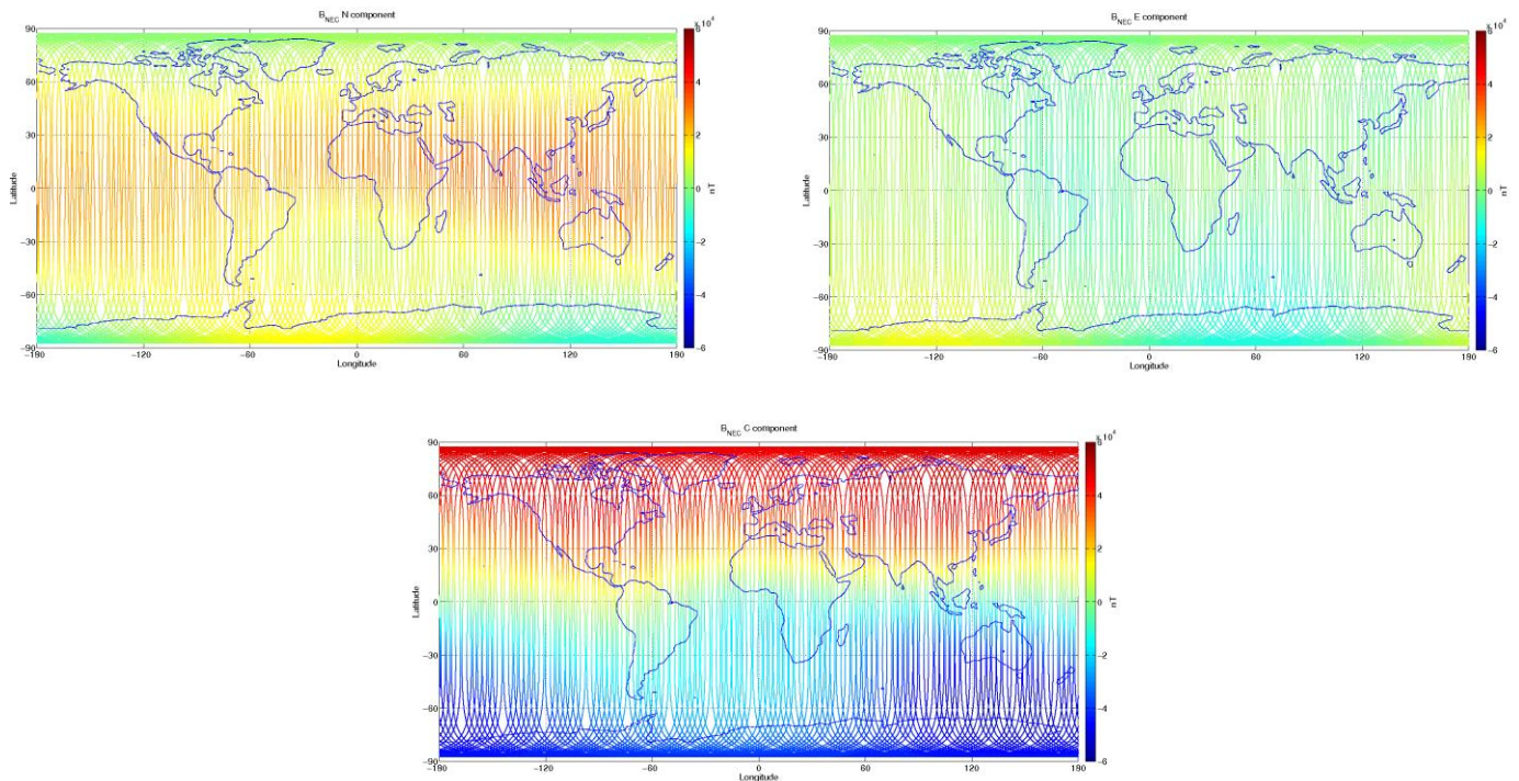
Figure 3-9: S/C C, world map plots of the geomagnetic field and components measured during monitoring period 21/10-27/10. From top to bottom: B_{NEC} components (North, East, and Centre) of magnetic field from VFM measurement
