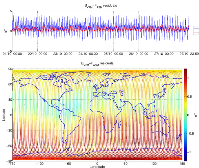
Figure 3-5: ASM-VFM residuals for S/C A, during monitoring period 21/10-27/10. In top figure are plotted: difference between |B_{VFM}| and F_{ASM} (without dB_Sun correction) (blue colour), and the residuals with dB_Sun corrections (red colour). In bottom figure residuals are presented on the world map.
