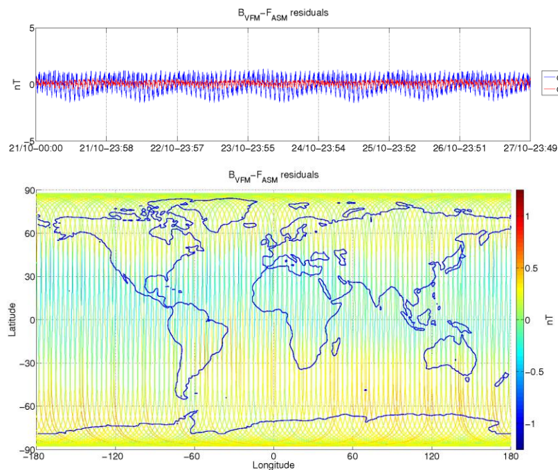
Figure 3-6: ASM-VFM residuals for S/C B, during monitoring period 21/10-27/10. In top figure are plotted: difference between |B_{VFM}| and F_{ASM} (without dB_Sun correction) (blue colour), and the residuals with dB_Sun corrections (red colour). In bottom figure residuals are presented on the world map.
