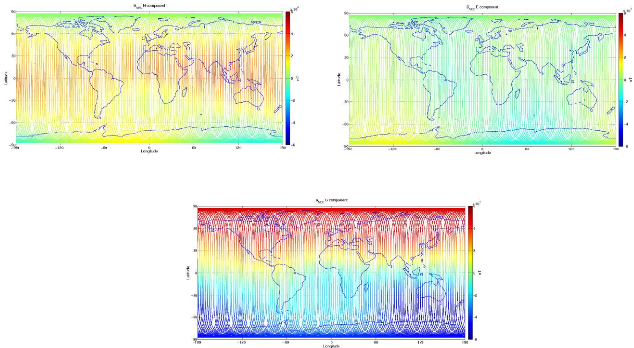
Figure 3-9: S/C C, world map plots of the geomagnetic field and components measured during monitoring period 14/10-20/10. From top to bottom: B_{NEC} components (North, East, and Centre) of magnetic field from VFM measurement
