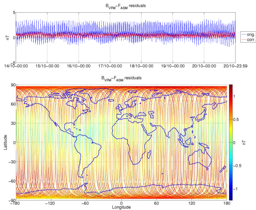
Figure 3-5: ASM-VFM residuals for S/C A, during monitoring period 14/10-20/10. In top figure are plotted: difference between |B_{VFM}| and F_{ASM} (without dB_{Sun} correction) (blue colour), and the residuals with dB_{Sun} corrections (red colour). In bottom figure residuals are presented on the world map.
