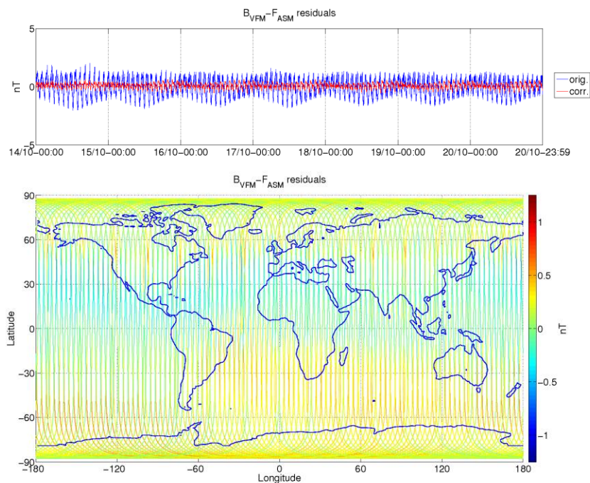
Figure 3-6: ASM-VFM residuals for S/C B, during monitoring period 14/10-20/10. In top figure are plotted: difference between |B_{VFM}| and F_{ASM} (without dB Sun correction) (blue colour), and the residuals with dB Sun corrections (red colour). In bottom figure residuals are presented on the world map.
