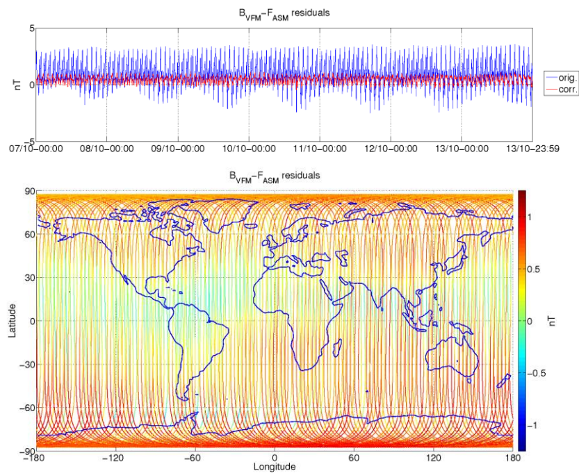
Figure 3-5: ASM-VFM residuals for S/C A, during monitoring period 07/10-13/10. In top figure are plotted: difference between |B_{VFM}| and F_{ASM} (without dB_{Sun} correction) (blue colour), and the residuals with dB_{Sun} corrections (red colour). In bottom figure residuals are presented on the world map.
