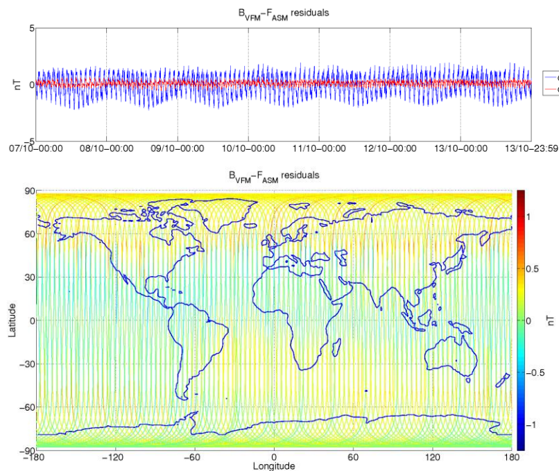
Figure 3-6: ASM-VFM residuals for S/C B, during monitoring period 07/10-13/10. In top figure are plotted: difference between |B_{VFM}| and F_{ASM} (without dB Sun correction) (blue colour), and the residuals with dB Sun corrections (red colour). In bottom figure residuals are presented on the world map.
