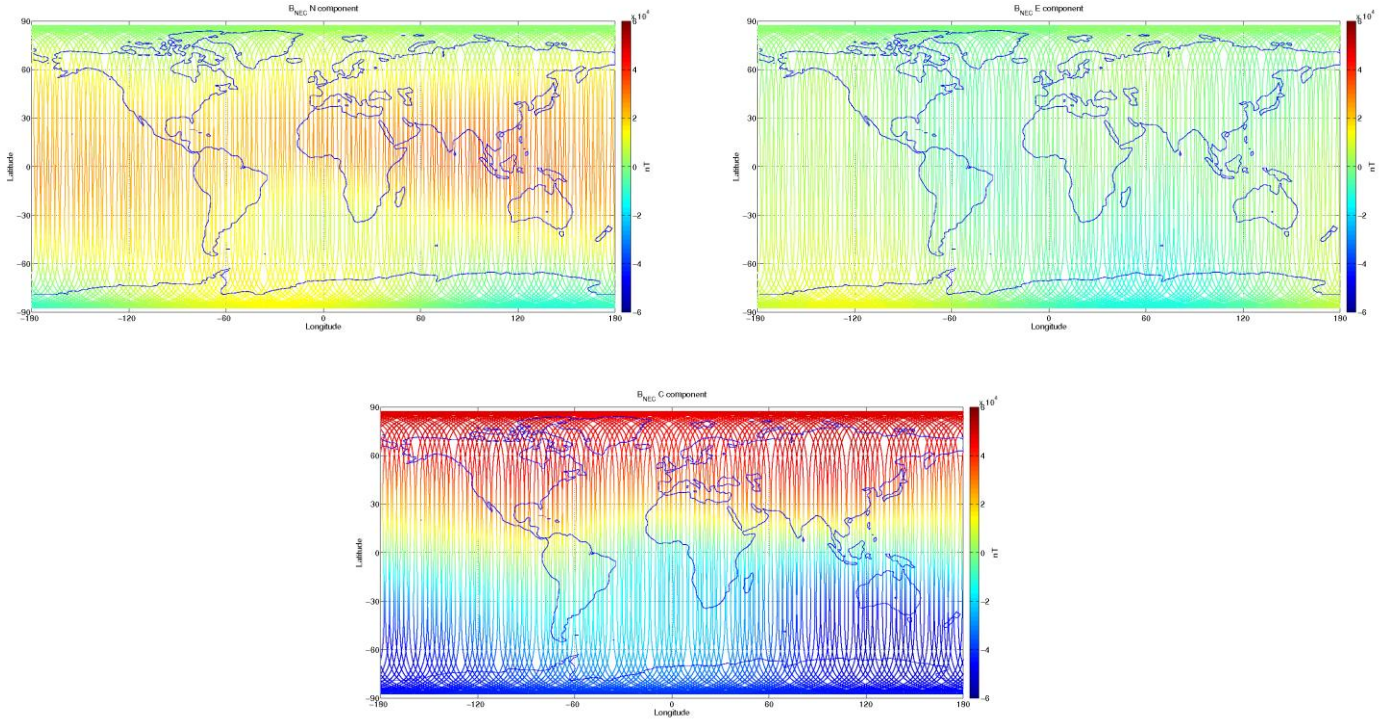
Figure 3-8: S/C C, world map plots of the geomagnetic field and components measured during monitoring period 23/09-29/09. From top to bottom: B_{NEC} components (North, East, and Centre) of magnetic field from VFM measurement
