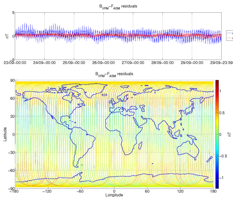
Figure 3-5: ASM-VFM residuals for S/C B, during monitoring period 23/09-29/09. In top figure are plotted: difference between |B_{VFM}| and F_{ASM} (without dB_{Sun} correction) (blue colour), and the residuals with dB_{Sun} corrections (red colour). In bottom figure residuals are presented on the world map.
