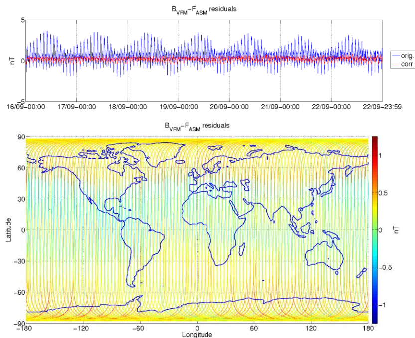
Figure 3-6: ASM-VFM residuals for S/C B, during monitoring period 16/09-22/09. In top figure are plotted: difference between |B_{VFM}| and F_{ASM} (without dB Sun correction) (blue colour), and the residuals with dB Sun corrections (red colour). In bottom figure residuals are presented on the world map.
