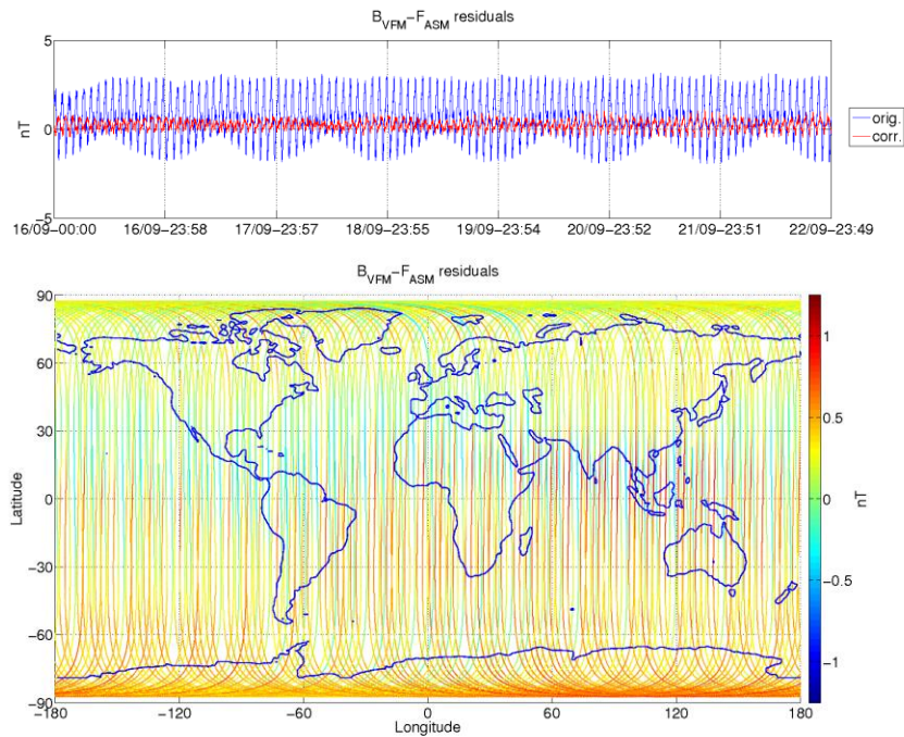
Figure 3-5: ASM-VFM residuals for S/C A, during monitoring period 16/09-22/09. In top figure are plotted: difference between |B_{VFM}| and F_{ASM} (without dB_{Sun} correction) (blue colour), and the residuals with dB_{Sun} corrections (red colour). In bottom figure residuals are presented on the world map.
