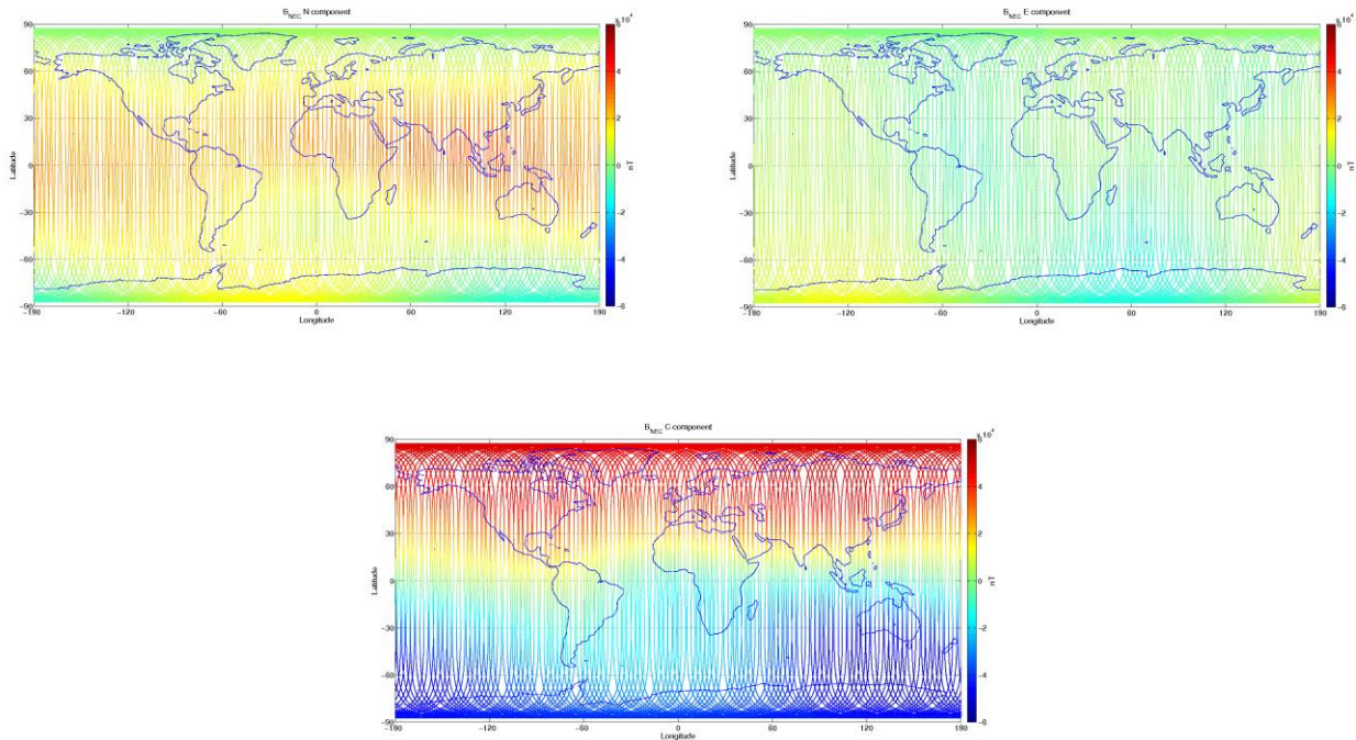
Figure 3-9: S/C C, world map plots of the geomagnetic field and components measured during monitoring period 09/09-15/09. From top to bottom: B_{NEC} components (North, East, and Centre) of magnetic field from VFM measurement.
