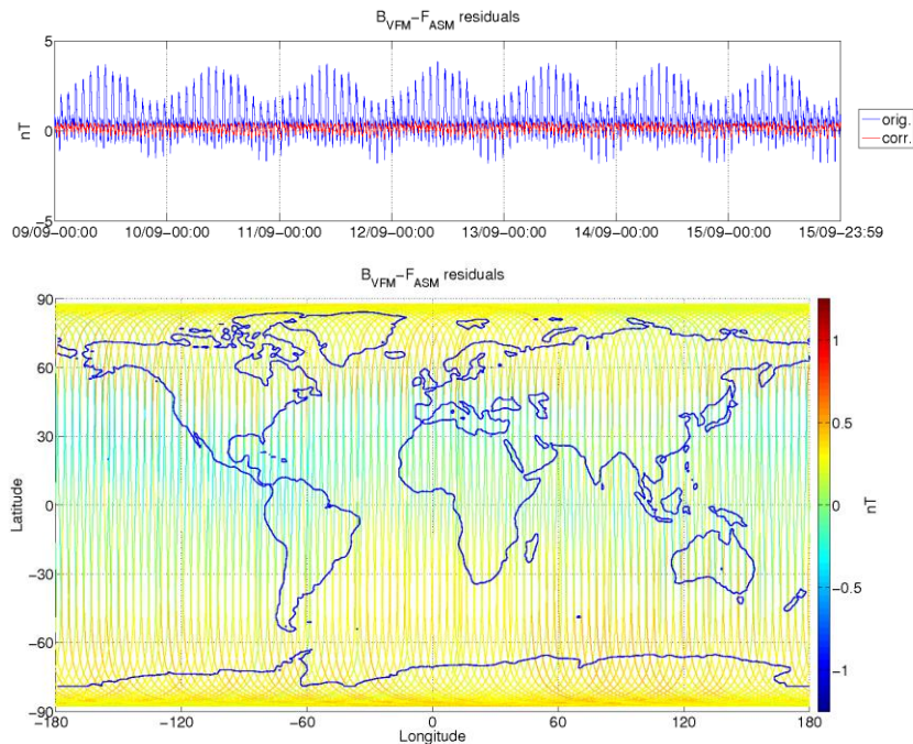
Figure 3-6: ASM-VFM residuals for S/C B, during monitoring period 09/09-15/09. In top figure are plotted: difference between |B_{VFM}| and F_{ASM} (without dB Sun correction) (blue colour), and the residuals with dB Sun corrections (red colour). In bottom figure residuals are presented on the world map.
