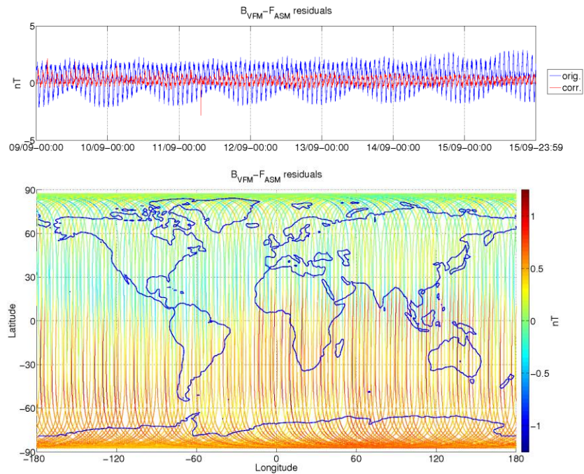
Figure 3-5: ASM-VFM residuals for S/C A, during monitoring period 09/09-15/09. In top figure are plotted: difference between |B_{VFM}| and F_{ASM} (without dB_{Sun} correction) (blue colour), and the residuals with dB_{Sun} corrections (red colour). In bottom figure residuals are presented on the world map.
