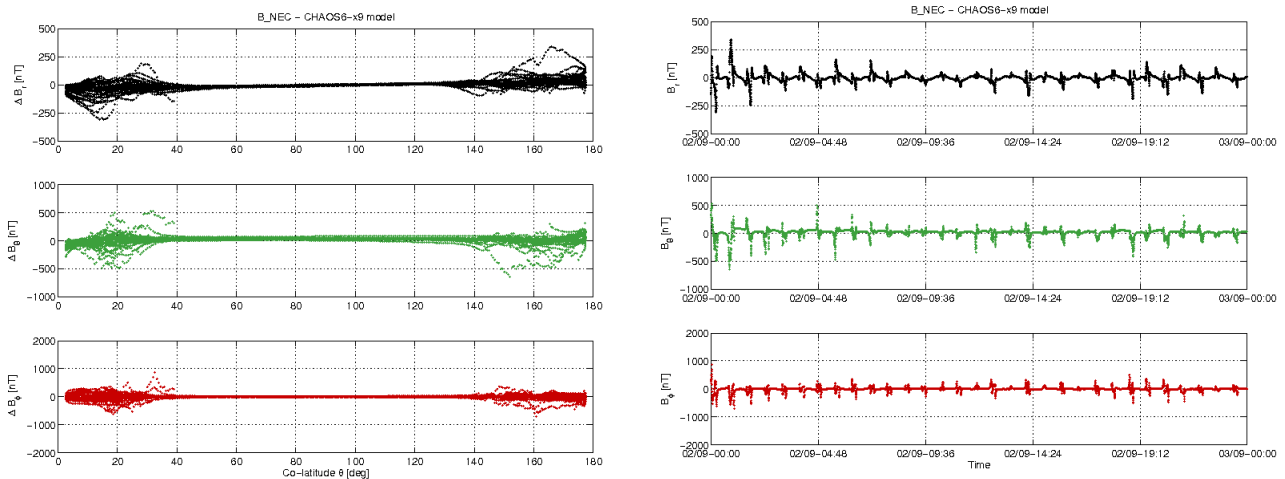
Figure 3-10: S/C A day 02.09: time series of B_{NEC} - B_{Chaos} residuals (right) and B_{NEC} - B_{Chaos} vs colatitude (left).
