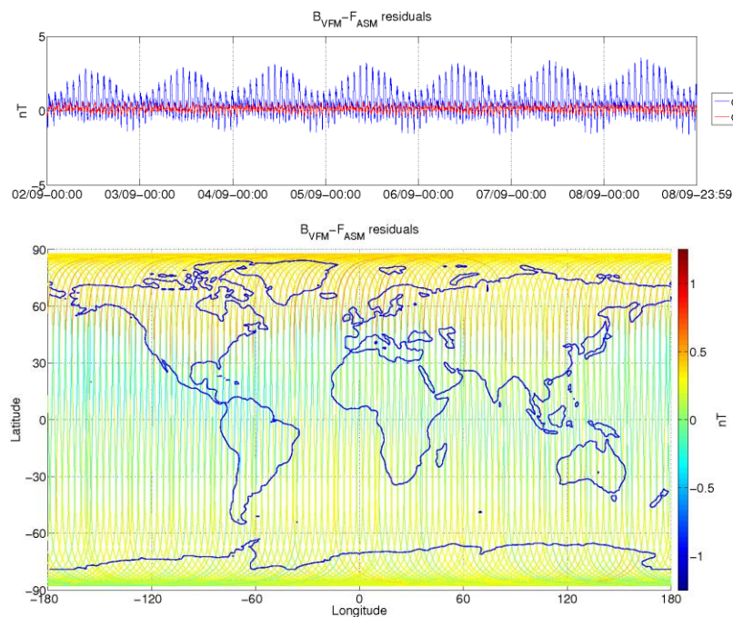
Figure 3-6: ASM-VFM residuals for S/C B, during monitoring period 02/09-08/09. In top figure are plotted: difference between |B_{VFM}| and F_{ASM} (without dB Sun correction) (blue colour), and the residuals with dB Sun corrections (red colour). In bottom figure residuals are presented on the world map.
