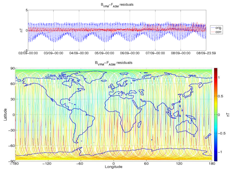
Figure 3-5: ASM-VFM residuals for S/C A, during monitoring period 02/09-08/09. In top figure are plotted: difference between |B_{VFM}| and F_{ASM} (without dB_{Sun} correction) (blue colour), and the residuals with dB_{Sun} corrections (red colour). In bottom figure residuals are presented on the world map.
