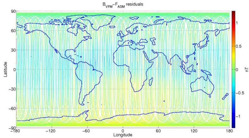
Figure 3-5: ASM-VFM residuals for S/C A, during monitoring period 19/08-25/08. In top figure are plotted: difference between |B_{VFM}| and F_{ASM} (without dB_{Sun} correction) (blue colour), and the residuals with dB_{Sun} corrections (red colour). In bottom figure residuals are presented on the world map.
