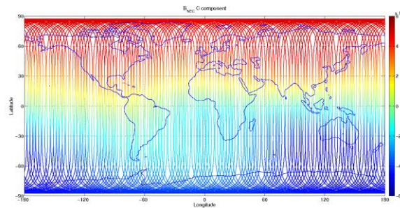
Figure 3-9: S/C C, world map plots of the geomagnetic field and components measured during monitoring period 19/08-25/08. From top to bottom: B_{NEC} components (North, East, and Centre) of magnetic field from VFM measurement
