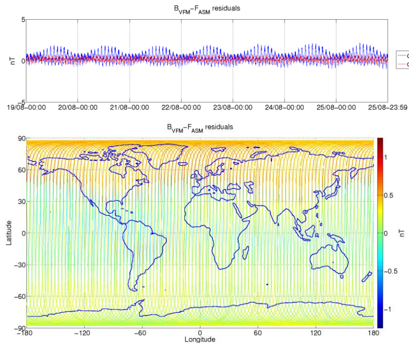
Figure 3-6: ASM-VFM residuals for S/C B, during monitoring period 19/08-25/08. In top figure are plotted: difference between |B_{VFM}| and F_{ASM} (without dB_{Sun} correction) (blue colour), and the residuals with dB_{Sun} corrections (red colour). In bottom figure residuals are presented on the world map.
