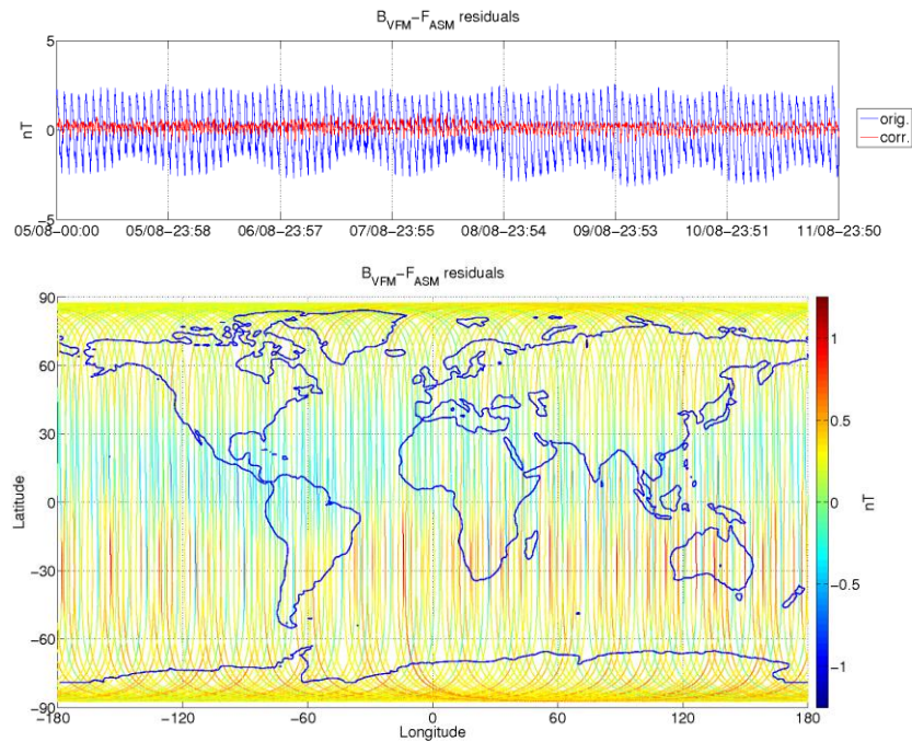
Figure 3-5: ASM-VFM residuals for S/C A, during monitoring period 05/08-11/08. In top figure are plotted: difference between |B_{VFM}| and F_{ASM} (without dB_{Sun} correction) (blue colour), and the residuals with dB_{Sun} corrections (red colour). In bottom figure residuals are presented on the world map.
