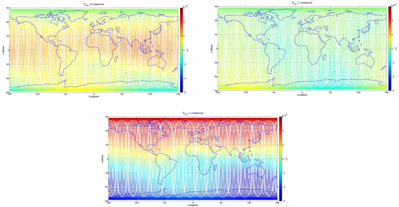
Figure 3-9: S/C C, world map plots of the geomagnetic field and components measured during monitoring period 05/08-11/08. From top to bottom: B_{NEC} components (North, East, and Centre) of magnetic field from VFM measurement
