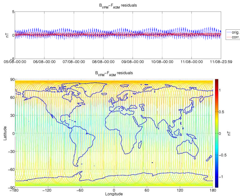
Figure 3-6: ASM-VFM residuals for S/C B, during monitoring period 05/08-11/08. In top figure are plotted: difference between |B_{VFM}| and F_{ASM} (without dB_Sun correction) (blue colour), and the residuals with dB_Sun corrections (red colour). In bottom figure residuals are presented on the world map.
