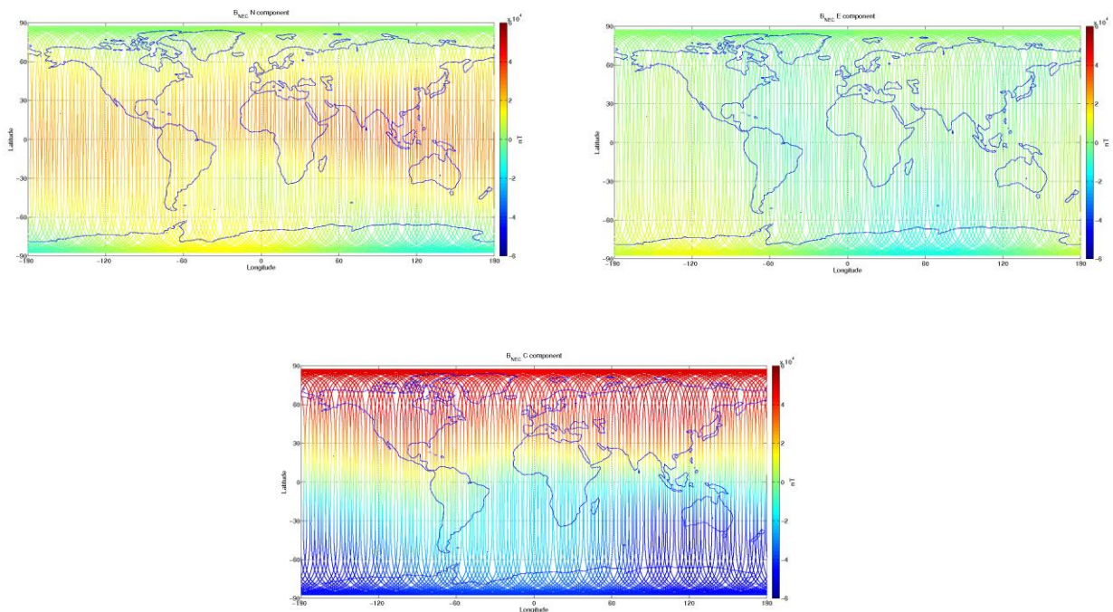
Figure 3-9: S/C C, world map plots of the geomagnetic field and components measured during monitoring period 29/07-04/08. From top to bottom: B_{NEC} components (North, East, and Centre) of magnetic field from VFM measurement
