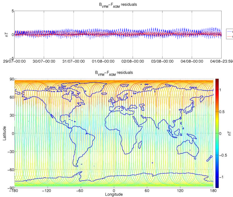
Figure 3-6: ASM-VFM residuals for S/C B, during monitoring period 29/07-04/08. In top figure are plotted: difference between |B_{VFM}| and F_{ASM} (without dB Sun correction) (blue colour), and the residuals with dB Sun corrections (red colour). In bottom figure residuals are presented on the world map.
