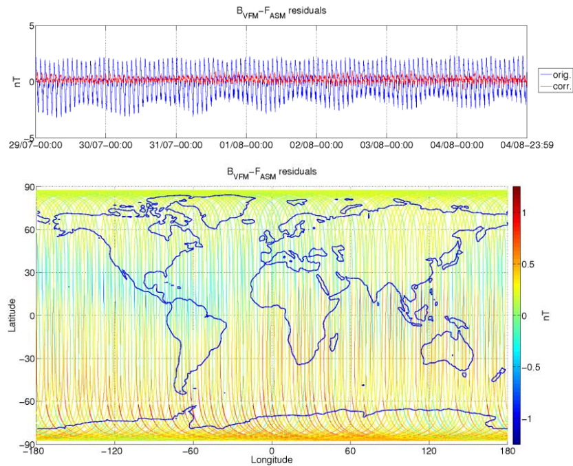
Figure 3-5: ASM-VFM residuals for S/C A, during monitoring period 29/07-04/08. In top figure are plotted: difference between |B_{VFM}| and F_{ASM} (without dB_{Sun} correction) (blue colour), and the residuals with dB_{Sun} corrections (red colour). In bottom figure residuals are presented on the world map.
