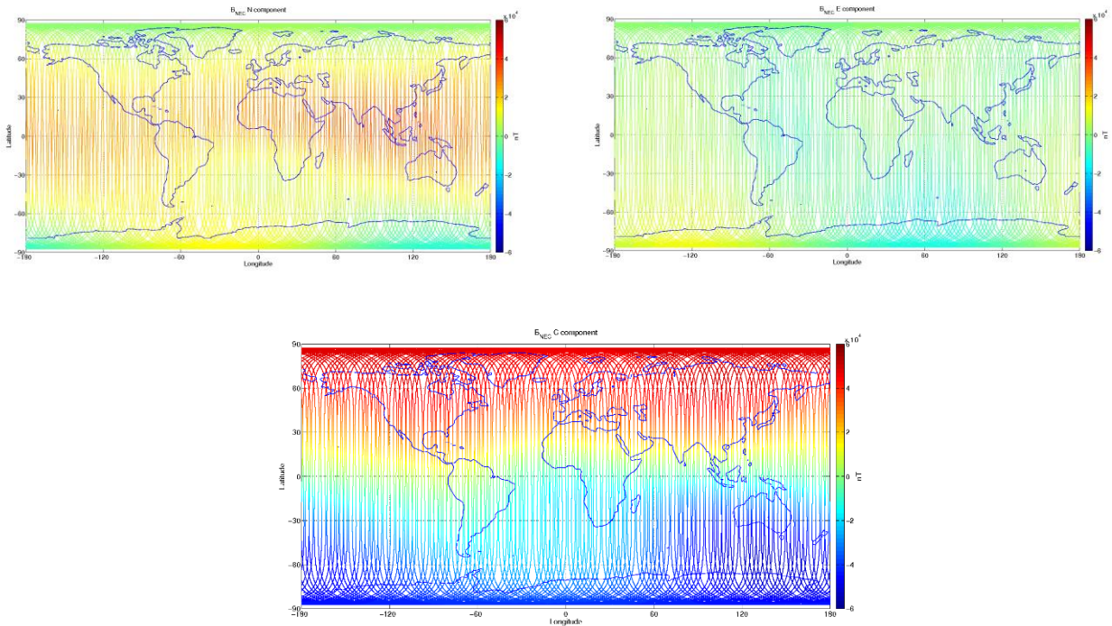
Figure 3-9: S/C C, world map plots of the geomagnetic field and components measured during monitoring period 22/07-28/07. From top to bottom: B_{NEC} components (North, East, and Centre) of magnetic field from VFM measurement
