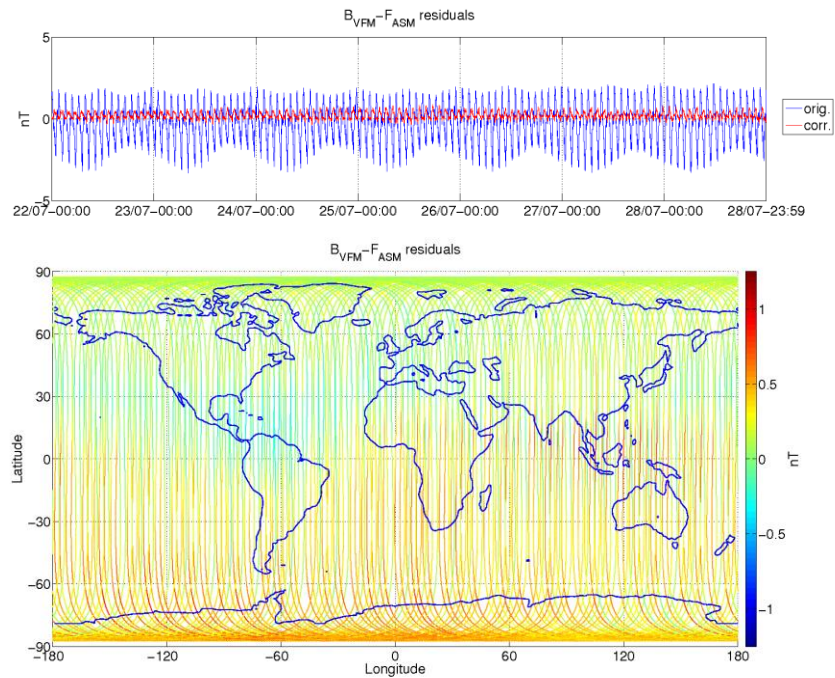
Figure 3-5: ASM-VFM residuals for S/C A, during monitoring period 22/07-28/07. In top figure are plotted: difference between |B_{VFM}| and F_{ASM} (without dB_{Sun} correction) (blue colour), and the residuals with dB_{Sun} corrections (red colour). In bottom figure residuals are presented on the world map.
