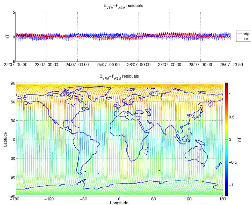
Figure 3-6: ASM-VFM residuals for S/C B, during monitoring period 22/07-28/07. In top figure are plotted: difference between |B_{VFM}| and F_{ASM} (without dB_{Sun} correction) (blue colour), and the residuals with dB_{Sun} corrections (red colour). In bottom figure residuals are presented on the world map.
