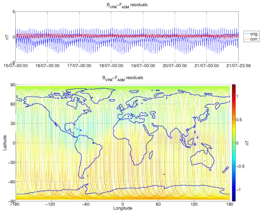
Figure 3-5: ASM-VFM residuals for S/C A, during monitoring period 15/07-21/07. In top figure are plotted: difference between |B_{VFM}| and F_{ASM} (without dB_{Sun} correction) (blue colour), and the residuals with dB_{Sun} corrections (red colour). In bottom figure residuals are presented on the world map.
