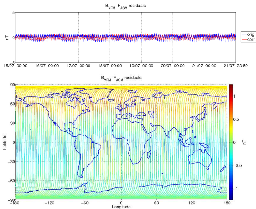
Figure 3-6: ASM-VFM residuals for S/C B, during monitoring period 15/07-21/07. In top figure are plotted: difference between |B_{VFM}| and F_{ASM} (without dB Sun correction) (blue colour), and the residuals with dB Sun corrections (red colour). In bottom figure residuals are presented on the world map.
