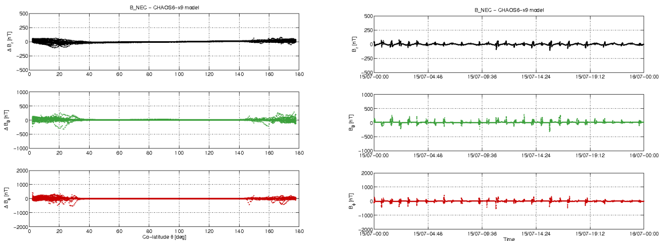
Figure 3-11: S/C B day 15.07 S/C B day 08/04: time series of B_{NEC} - B_{Chaos} residuals (right) and B_{NEC} - B_{Chaos} vs colatitude (left).
