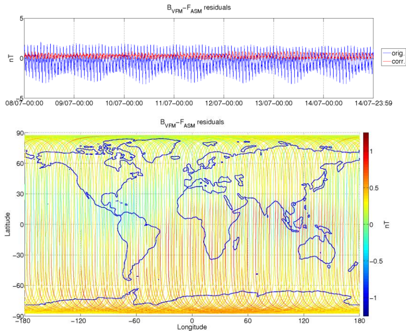
Figure 3-5: ASM-VFM residuals for S/C A, during monitoring period 08/07-14/07. In top figure are plotted: difference between |B_{VFM}| and F_{ASM} (without dB_{Sun} correction) (blue colour), and the residuals with dB_{Sun} corrections (red colour). In bottom figure residuals are presented on the world map.
