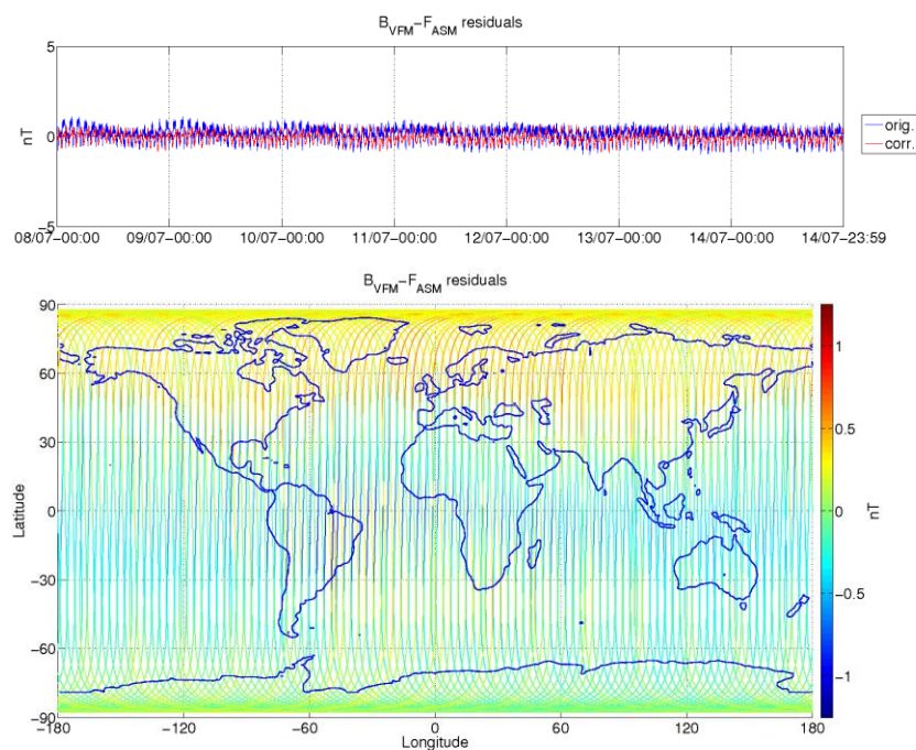
Figure 3-6: ASM-VFM residuals for S/C B, during monitoring period 08/07-14/07. In top figure are plotted: difference between |B_{VFM}| and F_{ASM} (without dB_{Sun} correction) (blue colour), and the residuals with dB_{Sun} corrections (red colour). In bottom figure residuals are presented on the world map.
