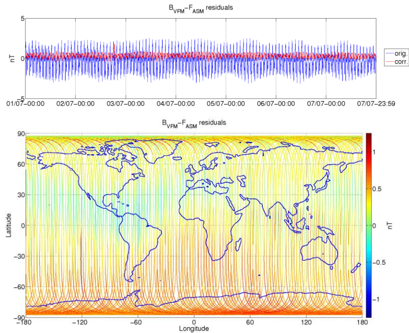
Figure 3-5: ASM-VFM residuals for S/C A, during monitoring period 01/07-07/07. In top figure are plotted: difference between |B_{VFM}| and F_{ASM} (without dB_{Sun} correction) (blue colour), and the residuals with dB_{Sun} corrections (red colour). In bottom figure residuals are presented on the world map.
