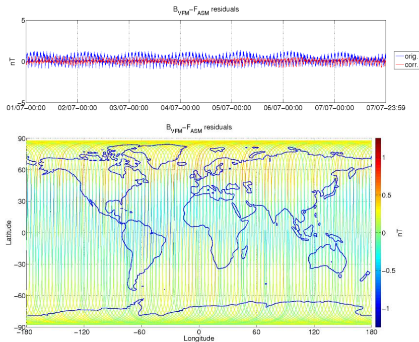
Figure 3-6: ASM-VFM residuals for S/C B, during monitoring period 01/07-07/07. In top figure are plotted: difference between |B_{VFM}| and F_{ASM} (without dB_{Sun} correction) (blue colour), and the residuals with dB_{Sun} corrections (red colour). In bottom figure residuals are presented on the world map.
