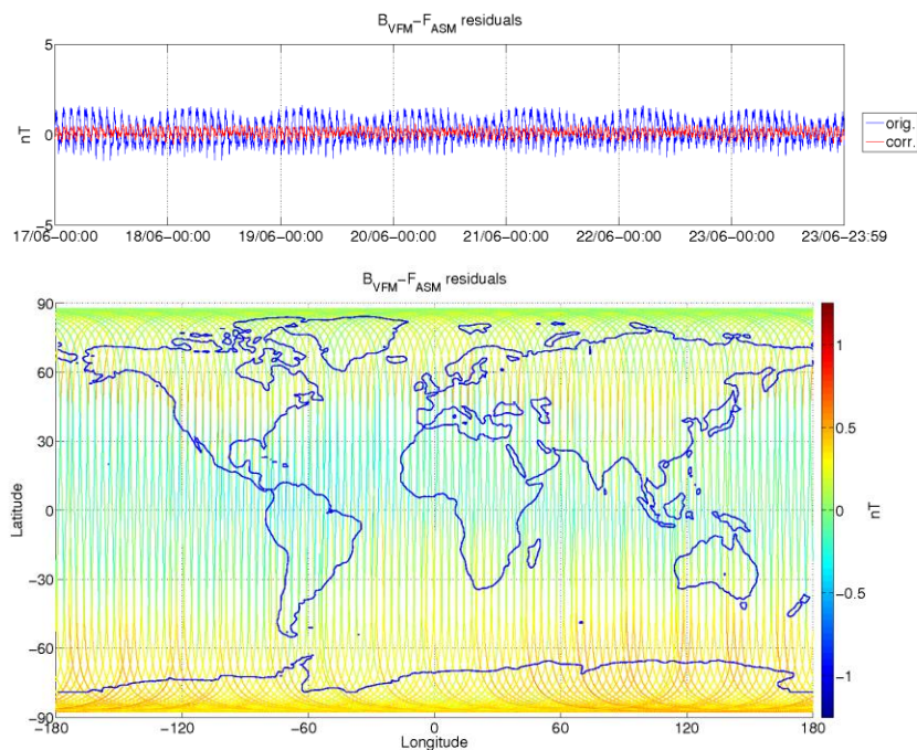
Figure 3-6: ASM-VFM residuals for S/C B, during monitoring period 17/06-23/06. In top figure are plotted: difference between |B_{VFM}| and F_{ASM} (without dB_Sun correction) (blue colour), and the residuals with dB_Sun corrections (red colour). In bottom figure residuals are presented on the world map.
