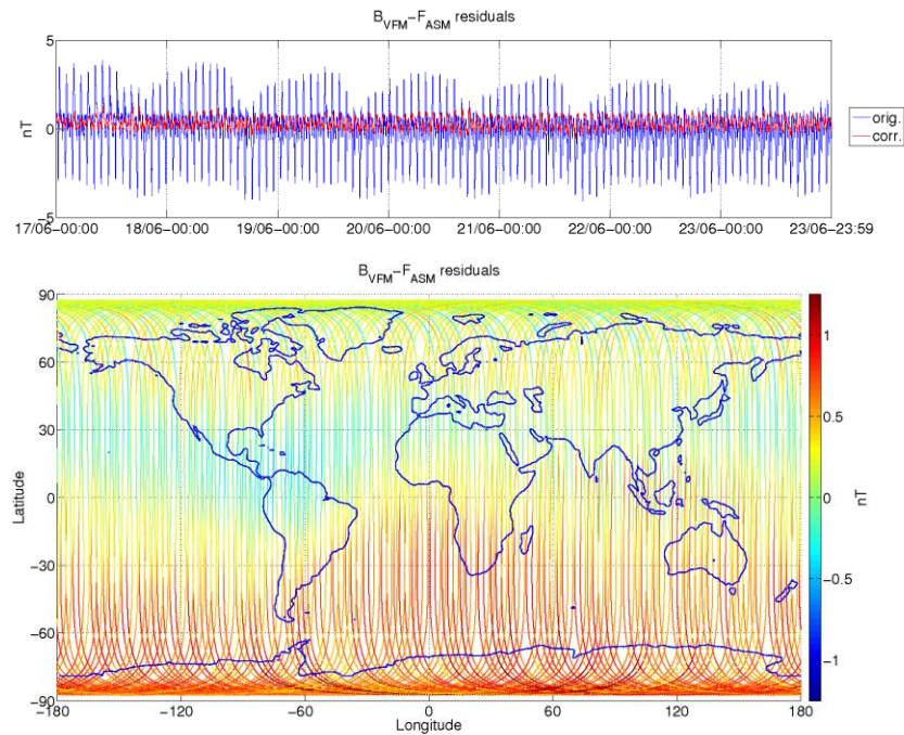
Figure 3-5: ASM-VFM residuals for S/C A, during monitoring period 17/06-23/06. In top figure are plotted: difference between |B_{VFM}| and F_{ASM} (without dB_{Sun} correction) (blue colour), and the residuals with dB_{Sun} corrections (red colour). In bottom figure residuals are presented on the world map.
