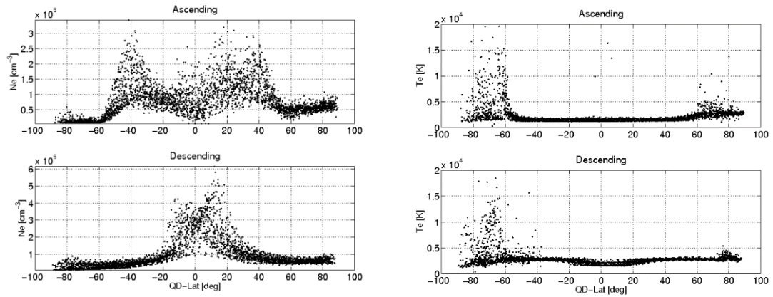
Figure 3-14: The panels show the electron density (left) and temperature (right) profile as a function of QD Latitudes for the last week of operation. The analysis is made separately for ascending (upper panels) and descending (bottom panels) orbits.
