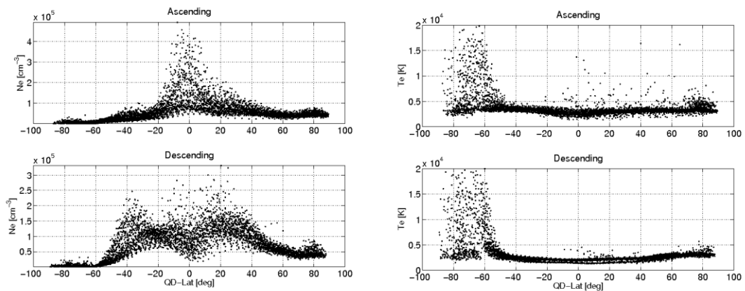
Figure 3-15: The panels show the electron density (left) and temperature (right) profile as a function of QD Latitudes for the last week of operation. The analysis is made separately for ascending (upper panels) and descending (bottom panels) orbits.
