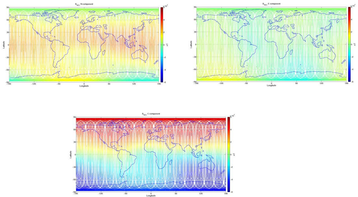
Figure 3-8: S/C C, world map plots of the geomagnetic field and components measured during monitoring period 10/06-16/06. From top to bottom: B_{NEC} components (North, East, and Centre) of magnetic field from VFM measurement
