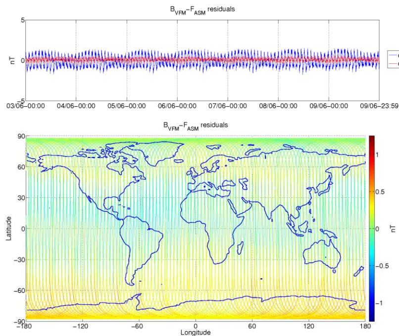
Figure 3-6: ASM-VFM residuals for S/C B, during monitoring period 03/06-09/06. In top figure are plotted: difference between |B_{VFM}| and F_{ASM} (without dB_{Sun} correction) (blue colour), and the residuals with dB_{Sun} corrections (red colour). In bottom figure residuals are presented on the world map.
