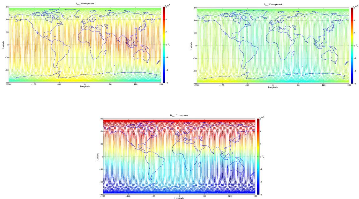
Figure 3-9: S/C C, world map plots of the geomagnetic field and components measured during monitoring period 03/06–09/06. From top to bottom: B_{NEC} components (North, East, and Centre) of magnetic field from VFM measurement.
