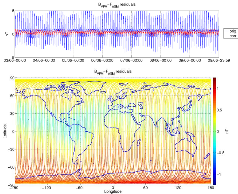
Figure 3-5: ASM-VFM residuals for S/C A, during monitoring period 03/06-09/06. In top figure are plotted: difference between |B_{VFM}| and F_{ASM} (without dB_{Sun} correction) (blue colour), and the residuals with dB_{Sun} corrections (red colour). In bottom figure residuals are presented on the world map.
