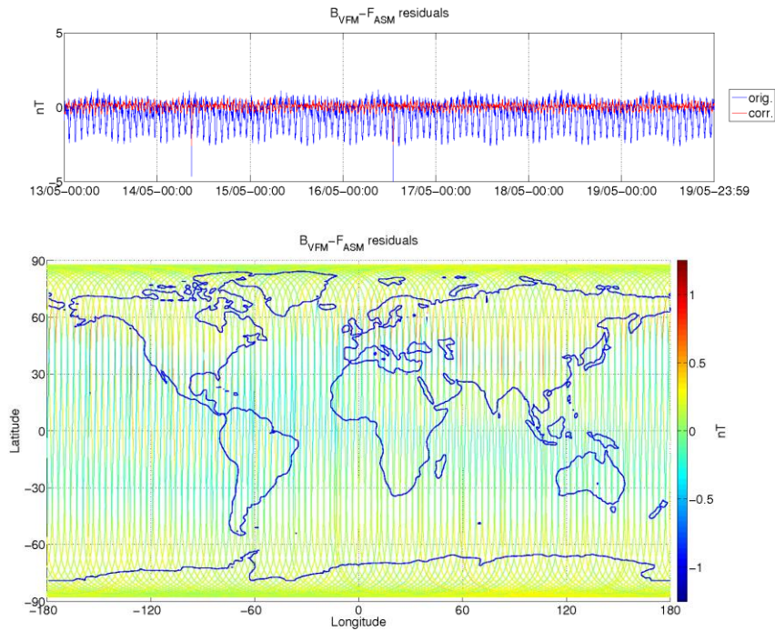
Figure 3-6: ASM-VFM residuals for S/C B, during monitoring period. In top figure are plotted: difference between |B_{VFM}| and F_{ASM} (without dB_{Sun} correction) (blue colour), and the residuals with dB_{Sun} corrections (red colour). In bottom figure residuals are presented on the world map.
