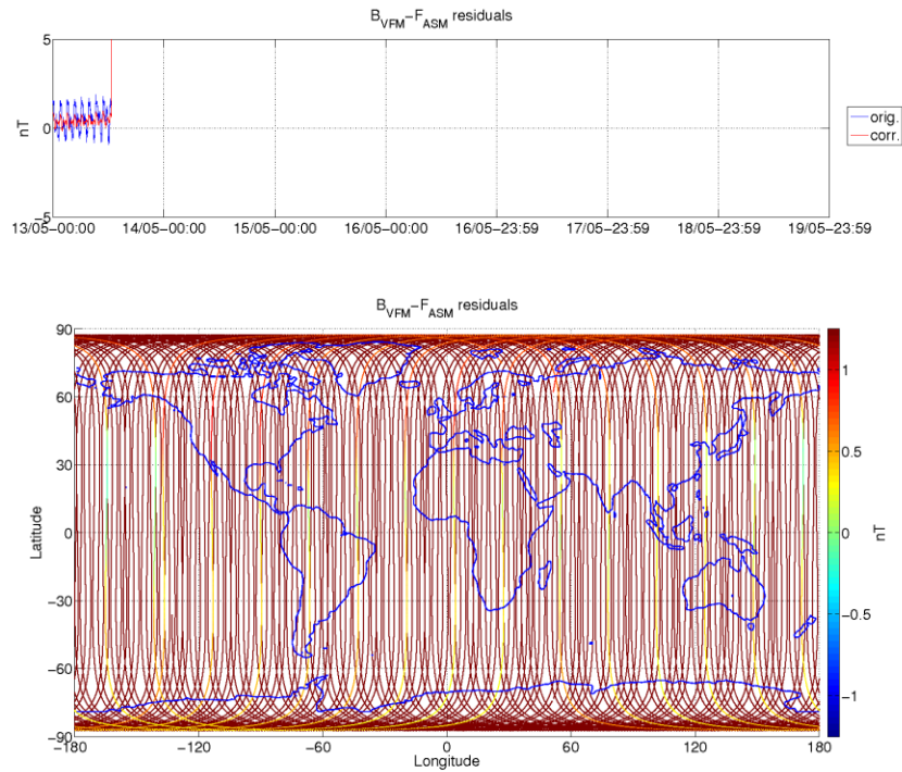
Figure 3-5: ASM-VFM residuals for S/C A, during monitoring period. In top figure are plotted: difference between |B_{VFM}| and F_{ASM} (without dB_{Sun} correction) (blue colour), and the residuals with dB_{Sun} corrections (red colour). In bottom figure residuals are presented on the world map.
