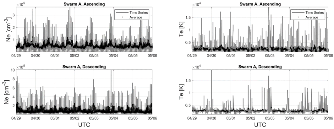
Figure 3-12: The panels show the electron density (left) and temperature (right) weekly time series (grey lines) together with the 20 min moving windows average (black lines). The analysis is made separately for ascending (upper panels) and descending (bottom panels) orbits. The average magnetic local time during the week is 4 a.m. for ascending phase and 4 p.m. for descending phase.
