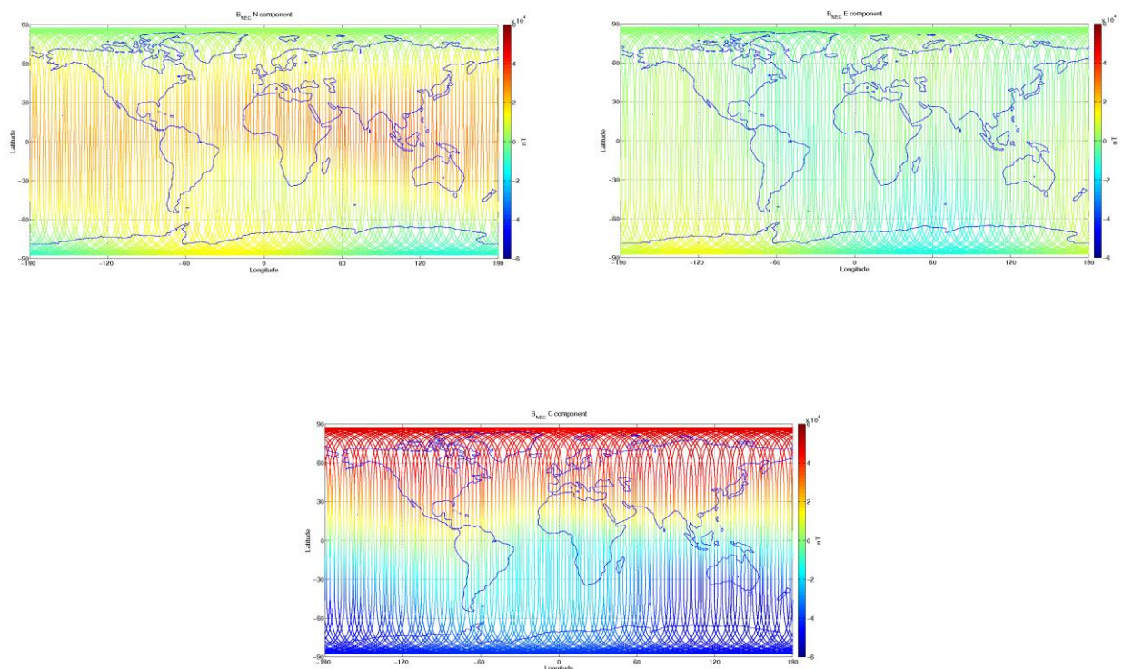
Figure 3-9: S/C C, world map plots of the geomagnetic field and components measured during monitoring period. From top left to bottom right: B_{NEC} components (North, East, and Centre) of magnetic field from VFM measurement, F-magnetic field from ASM measurement.
