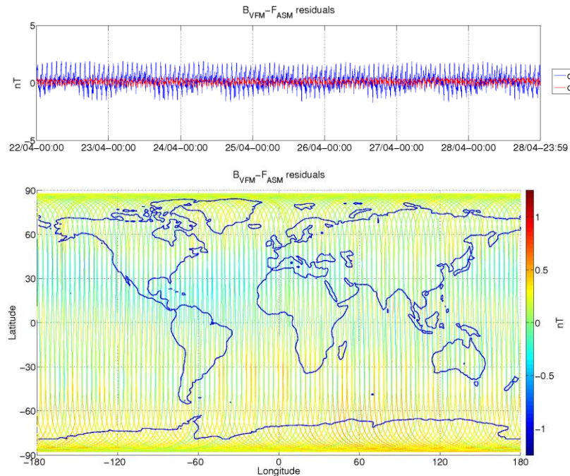
Figure 3-6: ASM-VFM residuals for S/C B, during monitoring period. In top figure are plotted: difference between |B_{VFM}| and F_{ASM} (without dB Sun correction) (blue colour), and the residuals with dB Sun corrections (red colour). In bottom figure residuals are presented on the world map.
