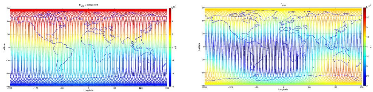
Figure 3-8: S/C B, world map plots of the geomagnetic field and components measured during monitoring period. From top left to bottom right: F-magnetic field from ASM measurement, B_{NEC} components (North, East, and Centre) of magnetic field from VFM measurement, F-magnetic field from ASM measurement.
