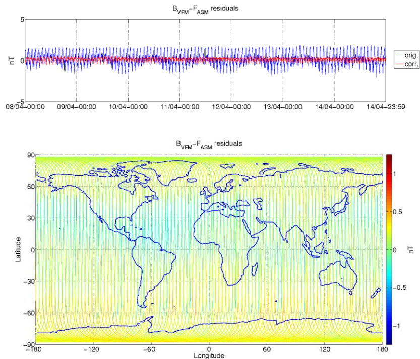
Figure 3-6: ASM-VFM residuals for S/C B, during monitoring period. In top figure are plotted: difference between |B_{VFM}| and F_{ASM} (without dB_{Sun} correction) (blue colour), and the residuals with dB_{Sun} corrections (red colour). In bottom figure residuals are presented on the world map.
