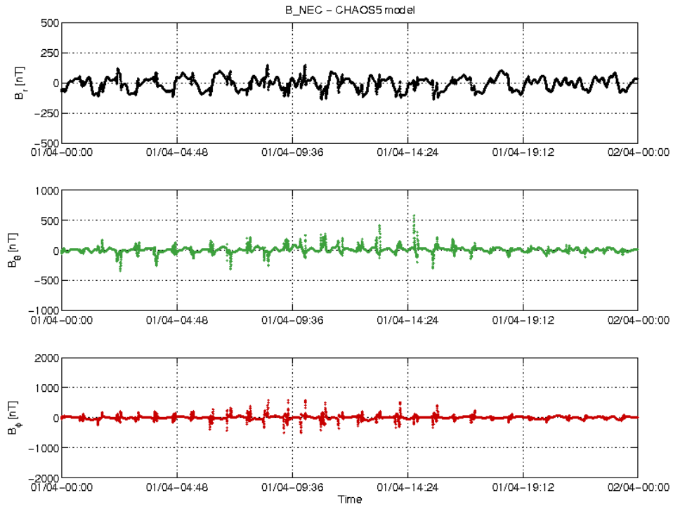
Figure 3-18: S/C A day 01.04: time series of B_{NEC} - B_{Chaos} residuals.
