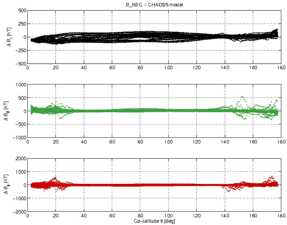
Figure 3-21: S/C C day 01.04 B_{NEC} - B_{Chaos} difference vs colatitude.
