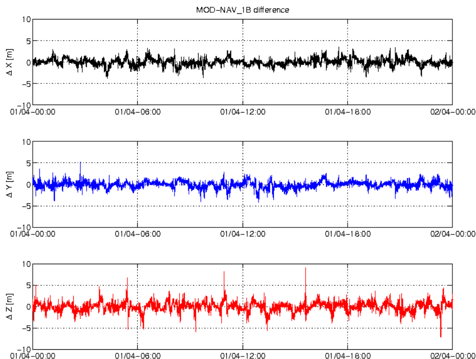
Figure 3-5: Difference MOD-GPSNAV, S/C C, 01.04. From top to bottom: X, Y and Z-axis
