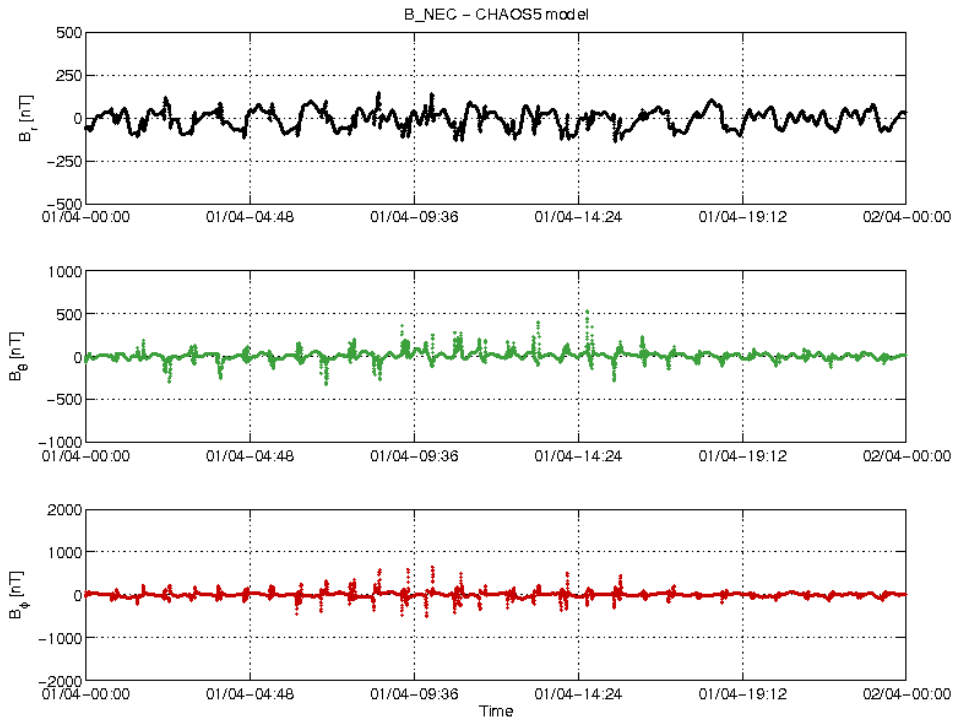
Figure 3-22: S/C C day 01.04 time series of B_{NEC} - B_{Chaos} residuals.
