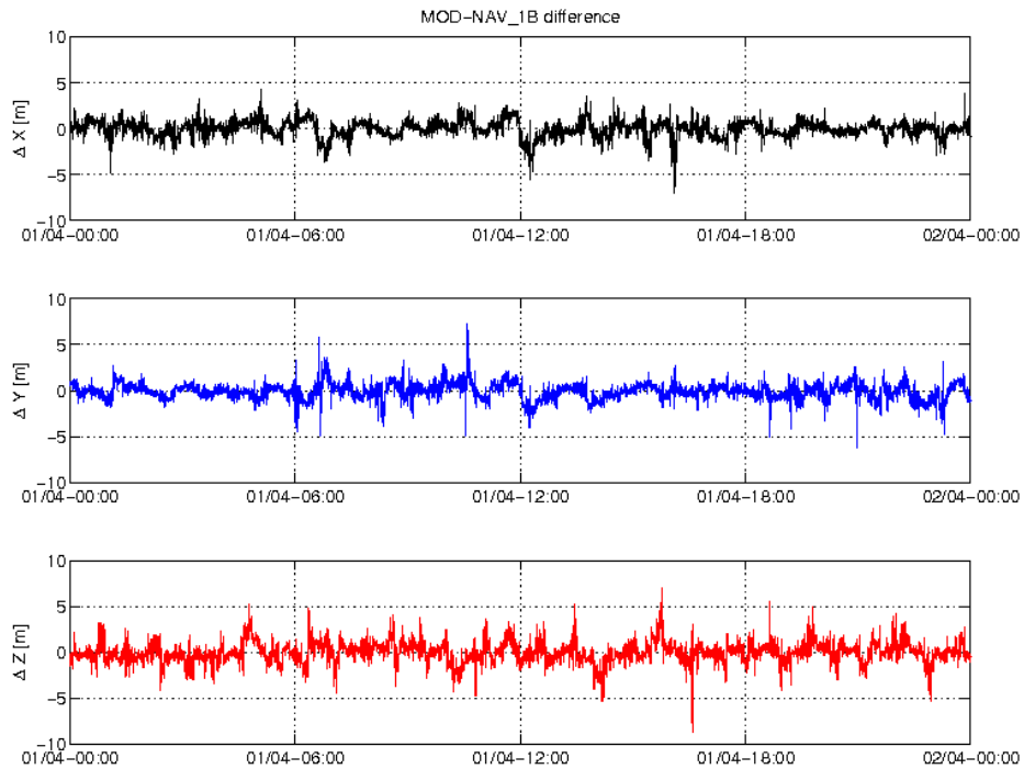
Figure 3-4: Difference MOD-GPSNAV, S/C B, 01.04. From top to bottom: X, Y and Z-axis
