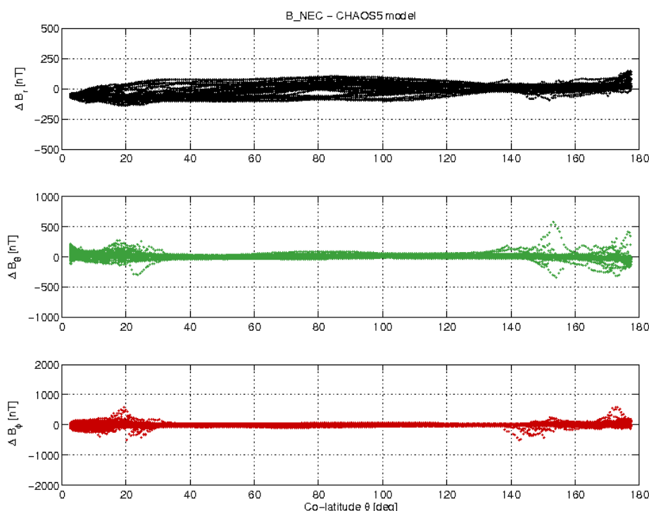
Figure 3-17: S/C A day 01.04 B_{NEC} - B_{Chaos5} vs colatitude.
