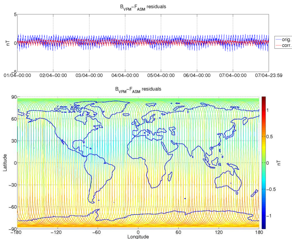
Figure 3-9: ASM-VFM residuals for S/C B, during monitoring period 01/04-07/04. In top figure are plotted: difference between |B VFM | and F ASM (without dB Sun correction) (blue colour), and the residuals with dB Sun corrections (red colour). In bottom figure residuals are presented on the world map.
