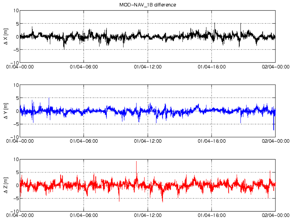
Figure 3-3: Difference MOD-GPSNAV, S/C A, 01.04. From top to bottom: X, Y and Z-axis
