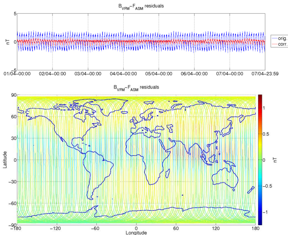
Figure 3-8: ASM-VFM residuals for S/C A, during monitoring period 01/04-07/04. In top figure are plotted: difference between |B_{VFM}| and F_{ASM} (without dB_{Sun} correction) (blue colour), and the residuals with dB_{Sun} corrections (red colour). In bottom figure residuals are presented on the world map.
