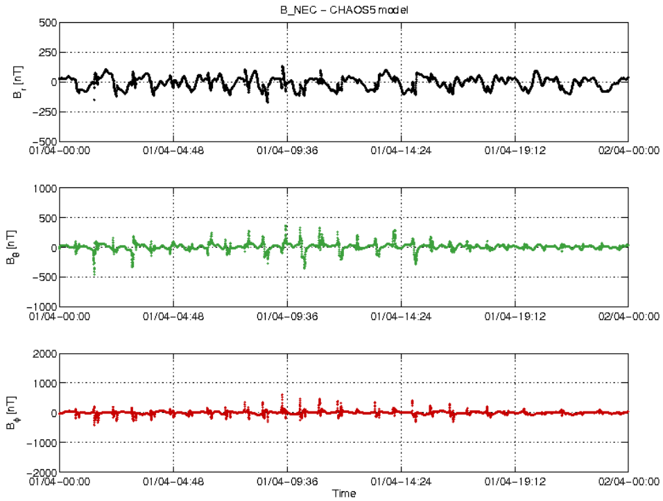
Figure 3-20: S/C B day 01.04 time series of B_{NEC} - B_{Chaos} residuals.
