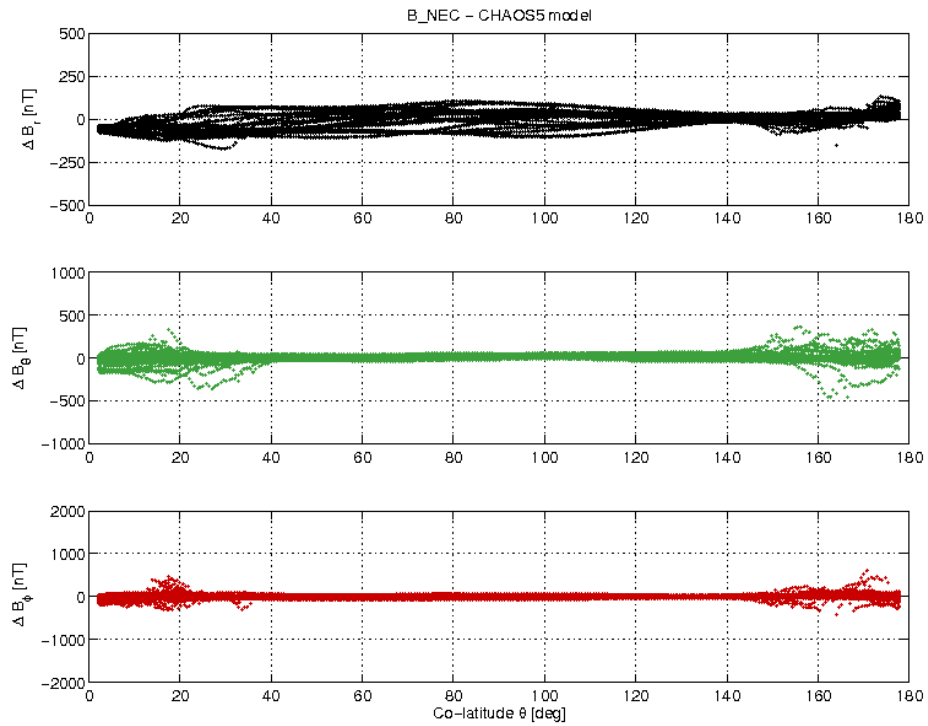
Figure 3-19: S/C B day 01.04 B_{NEC} - B_{Chaos} difference vs colatitude.
