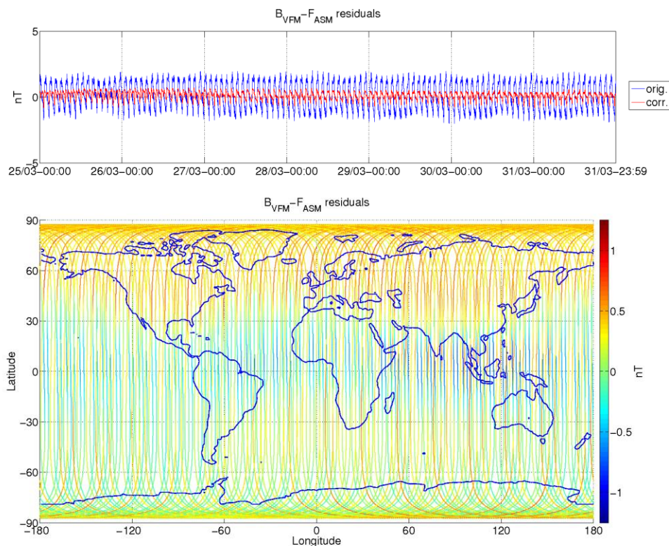
Figure 3-8: ASM-VFM residuals for S/C A, during monitoring period 25/03-31/03. In top figure are plotted: difference between |B_{VFM}| and F_{ASM} (without dB_{Sun} correction) (blue colour), and the residuals with dB_{Sun} corrections (red colour). In bottom figure residuals are presented on the world map.
