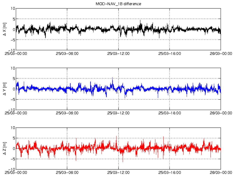
Figure 3-4: Difference MOD-GPSNAV, S/C B, 25.03. From top to bottom: X, Y and Z-axis
