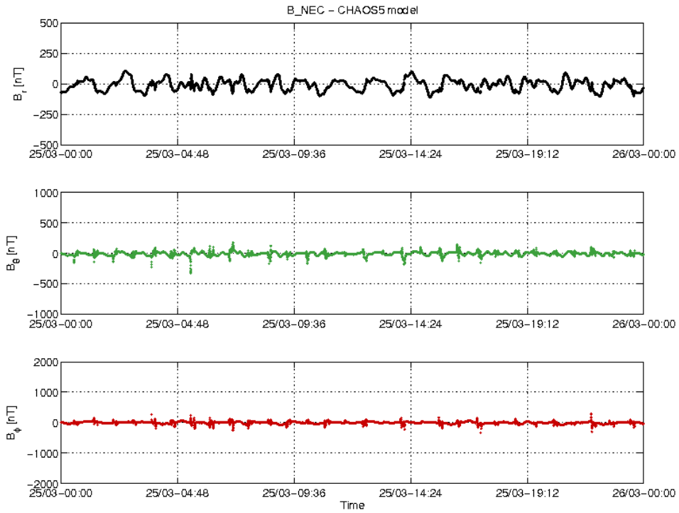
Figure 3-20: S/C B day 25.03 time series of B_{NEC} - B_{Chaos} residuals.
