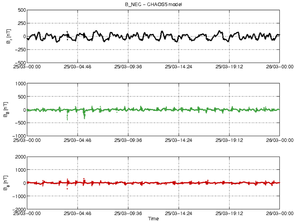
Figure 3-18: S/C A day 25.03: time series of B_{NEC} - B_{Chaos} residuals.
