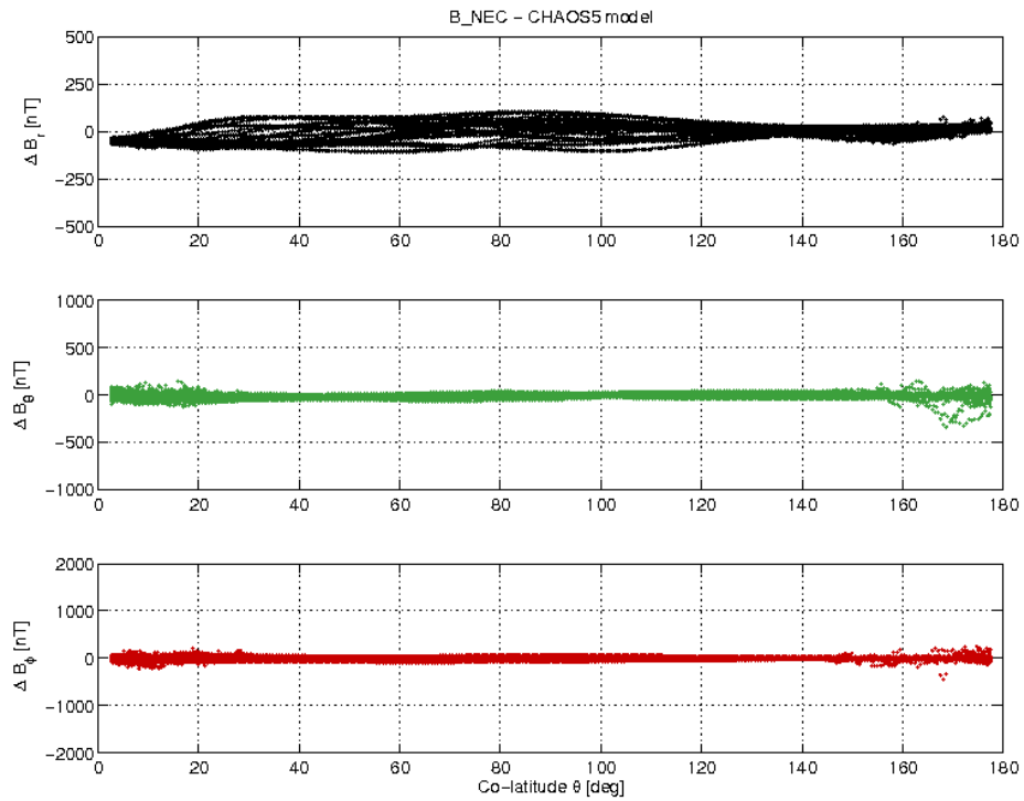
Figure 3-21: S/C C day 25.03 B_{NEC} - B_{Chaos} difference vs colatitude.
