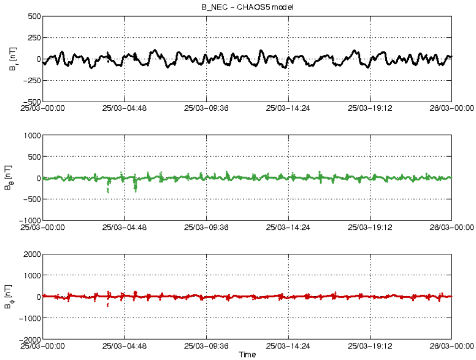
Figure 3-22: S/C C day 25.03 time series of B_{NEC} - B_{Chaos} residuals.
