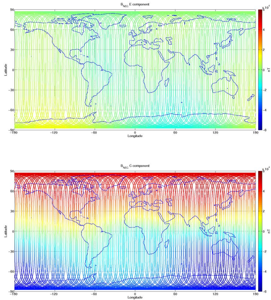
Figure 3-10: S/C A, world map plots of the geomagnetic field and components measured during monitoring period 25/03-31/03. From top to bottom: F-magnetic field from ASM measurement, B_{NEC} components (North, East, and Centre) of magnetic field from VFM measurement.
