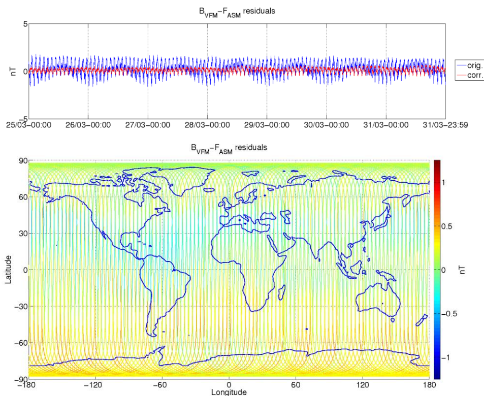
Figure 3-9: ASM-VFM residuals for S/C B, during monitoring period 25/03-31/03. In top figure are plotted: difference between |B\_VFM| and F\_ASM (without dB_Sun correction) (blue colour), and the residuals with dB_Sun corrections (red colour). In bottom figure residuals are presented on the world map.
