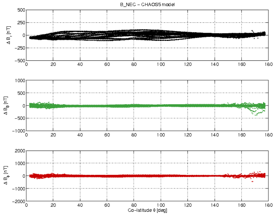
Figure 3-17: S/C A day 25.03 B_{NEC} - B_{Chaos} vs colatitude.
