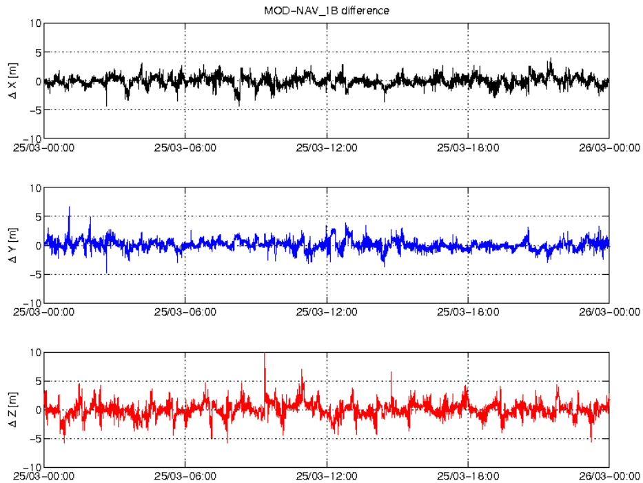
Figure 3-3: Difference MOD-GPSNAV, S/C A, 25.03. From top to bottom: X, Y and Z-axis
