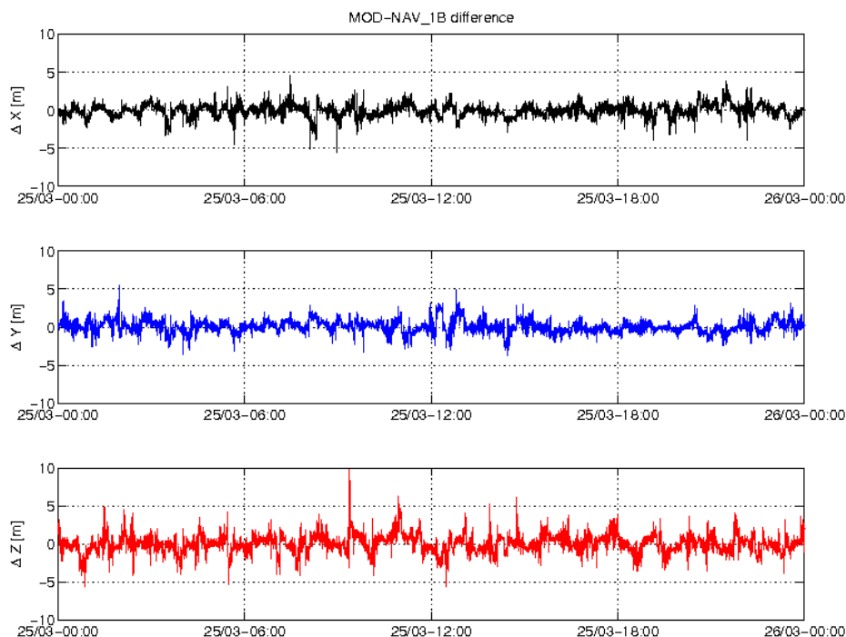
Figure 3-5: Difference MOD-GPSNAV, S/C C, 25.03. From top to bottom: X, Y and Z-axis
