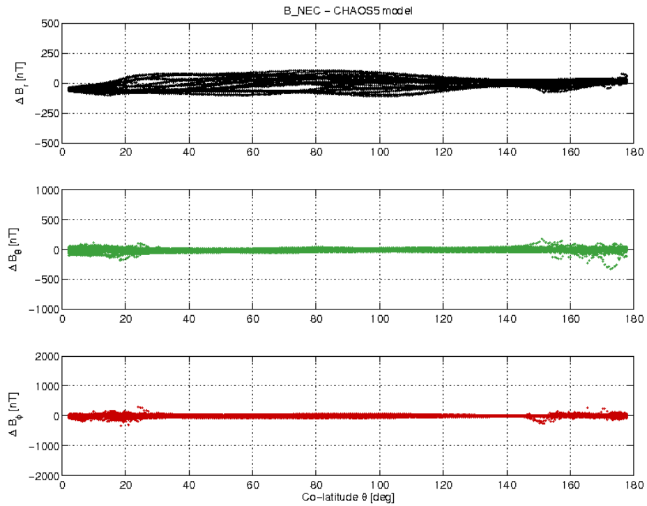
Figure 3-19: S/C B day 25.03 B_{NEC} - B_{Chaos} difference vs colatitude.
