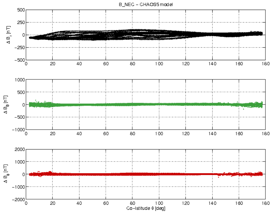
Figure 3-21: S/C C day 18.03 B_{NEC} - B_{Chaos} difference vs colatitude.
