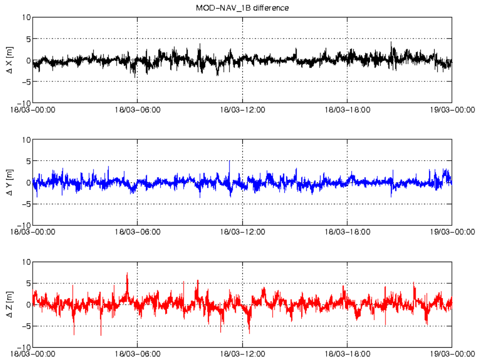
Figure 3-3: Difference MOD-GPSNAV, S/C A, 18.03. From top to bottom: X, Y and Z-axis
