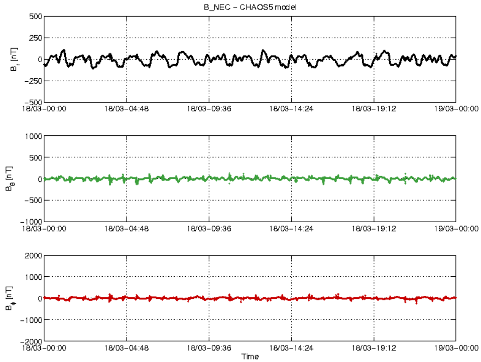
Figure 3-18: S/C A day 18.03: time series of B_{NEC} - B_{Chaos} residuals.
