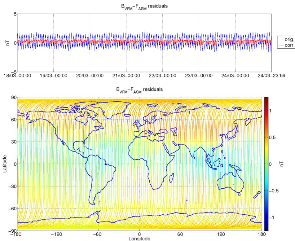
Figure 3-8: ASM-VFM residuals for S/C A, during monitoring period 18/03-24/03. In top figure are plotted: difference between |B_{VFM}| and F_{ASM} (without dB_{Sun} correction) (blue colour), and the residuals with dB_{Sun} corrections (red colour). In bottom figure residuals are presented on the world map.
