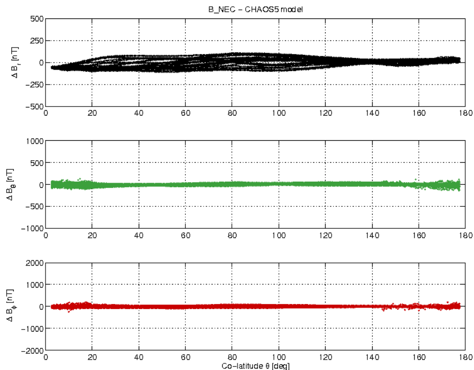
Figure 3-17: S/C A day 18.03 B_{NEC} - B_{Chaos} vs colatitude.
