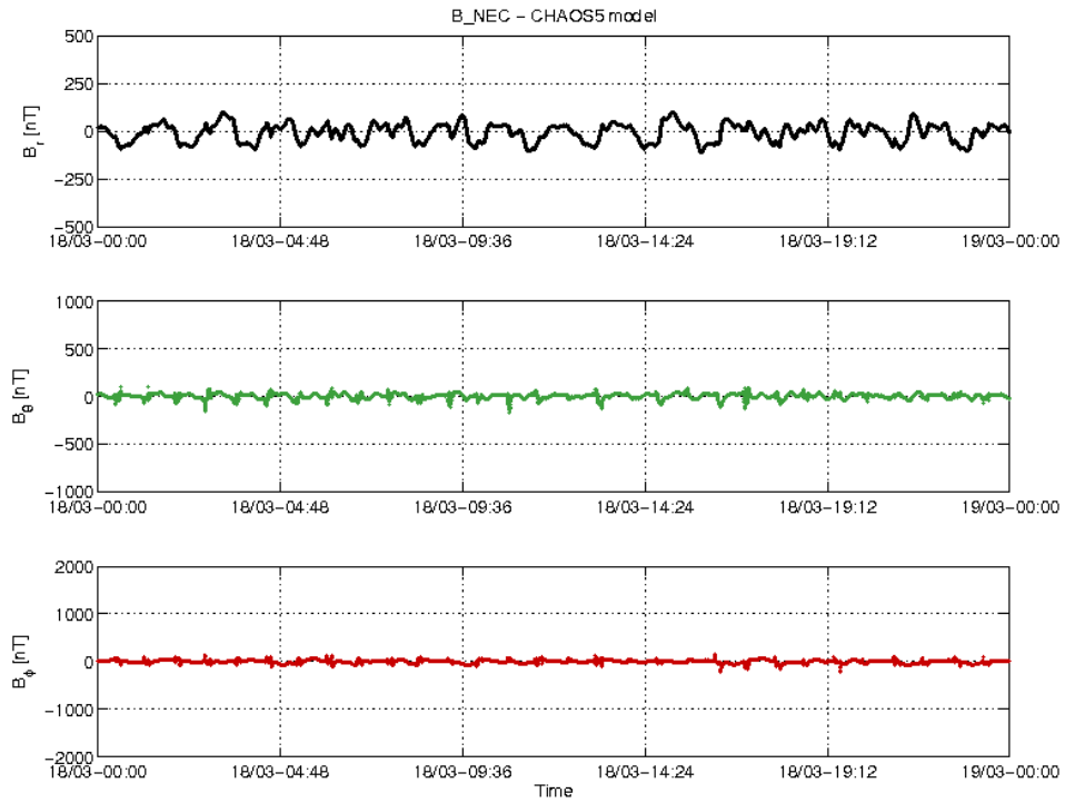
Figure 3-20: S/C B day 18.03 time series of B_{NEC} - B_{Chaos} residuals.
