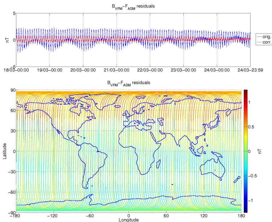
Figure 3-9: ASM-VFM residuals for S/C B, during monitoring period 18/03-24/03. In top figure are plotted: difference between |B_{VFM}| and F_{ASM} (without dB_Sun correction) (blue colour), and the residuals with dB_Sun corrections (red colour). In bottom figure residuals are presented on the world map.
