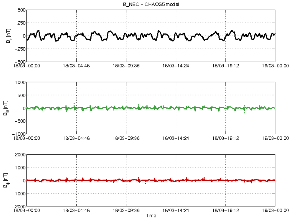
Figure 3-22: S/C C day 18.03 time series of B_{NEC} - B_{Chaos} residuals.
