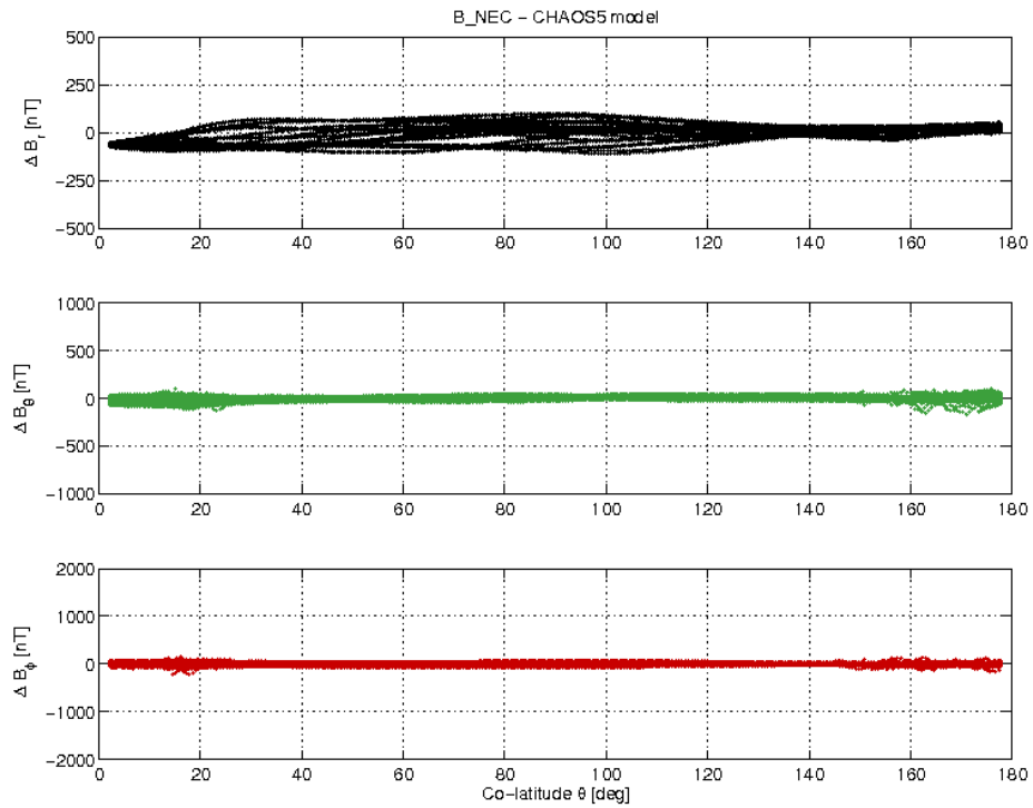
Figure 3-19: S/C B day 18.03 B_{NEC} - B_{Chaos} difference vs colatitude.
