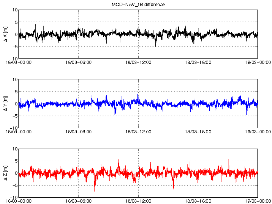
Figure 3-4: Difference MOD-GPSNAV, S/C B, 18.03. From top to bottom: X, Y and Z-axis
