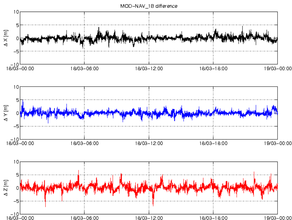
Figure 3-5: Difference MOD-GPSNAV, S/C C, 18.03. From top to bottom: X, Y and Z-axis
