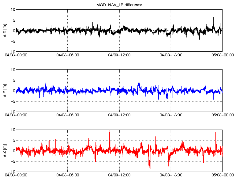
Figure 3-5: Difference MOD-GPSNAV, S/C C, 04.03. From top to bottom: X, Y and Z-axis
