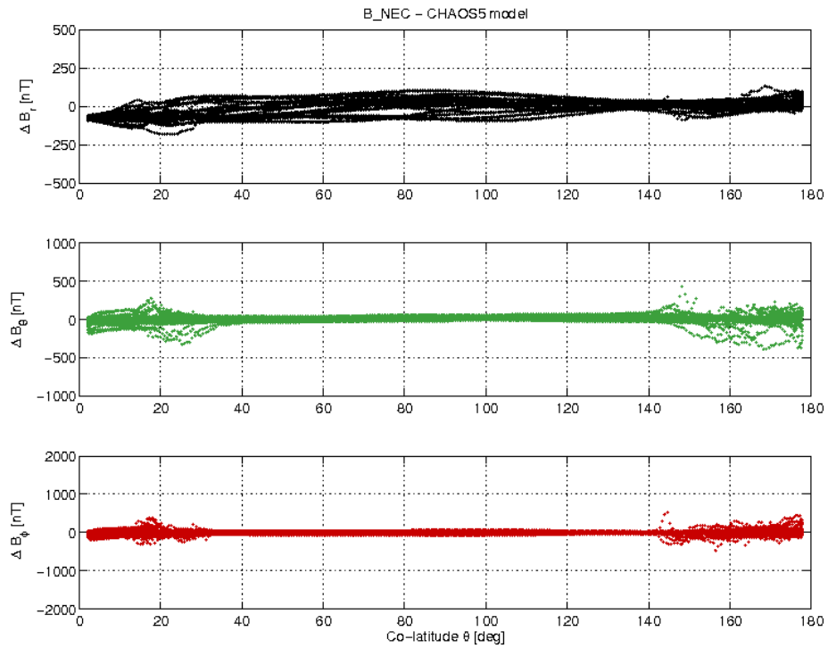
Figure 3-19: S/C B day 04.03 B_{NEC} - B_{Chaos} difference vs colatitude.
