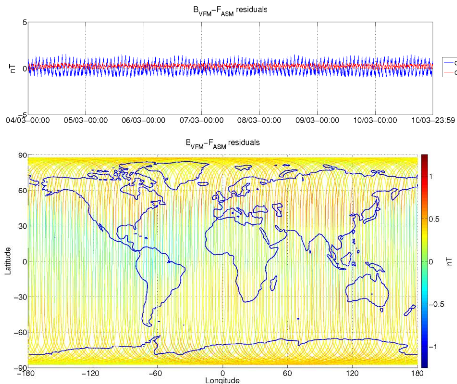
Figure 3-8: ASM-VFM residuals for S/C A, during monitoring period 04/03-10/03. In top figure are plotted: difference between |B_{VFM}| and F_{ASM} (without dB_{Sun} correction) (blue colour), and the residuals with dB_{Sun} corrections (red colour). In bottom figure residuals are presented on the world map.
