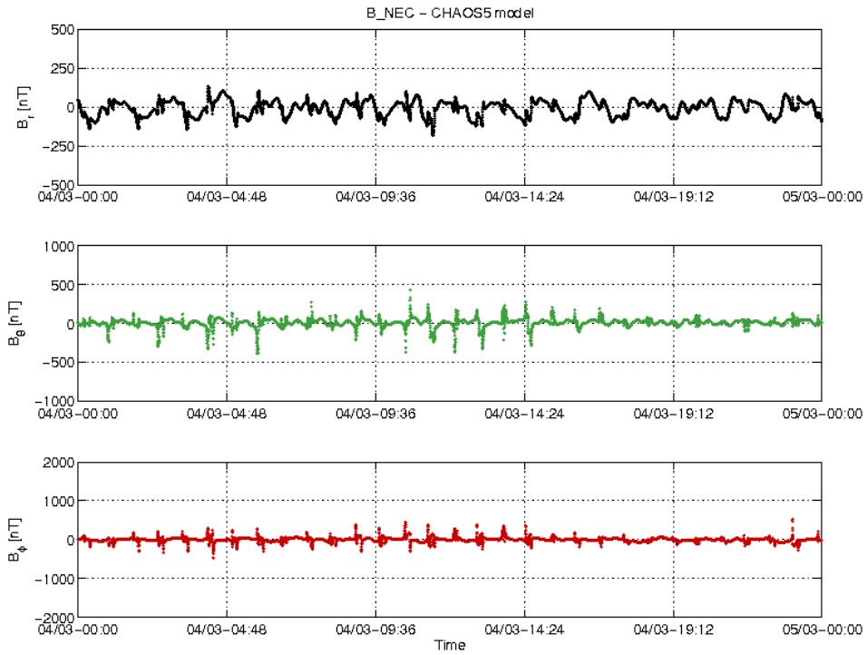
Figure 3-20: S/C B day 04.03 time series of B_{NEC} - B_{Chaos} residuals.
