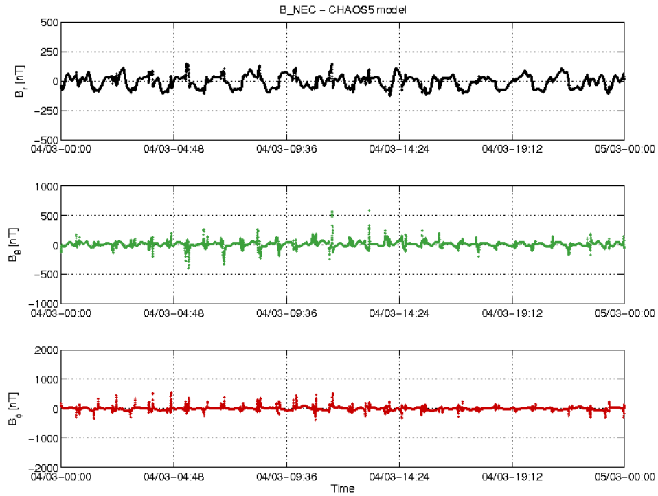
Figure 3-22: S/C C day 04.03 time series of B_{NEC} - B_{Chaos} residuals.
