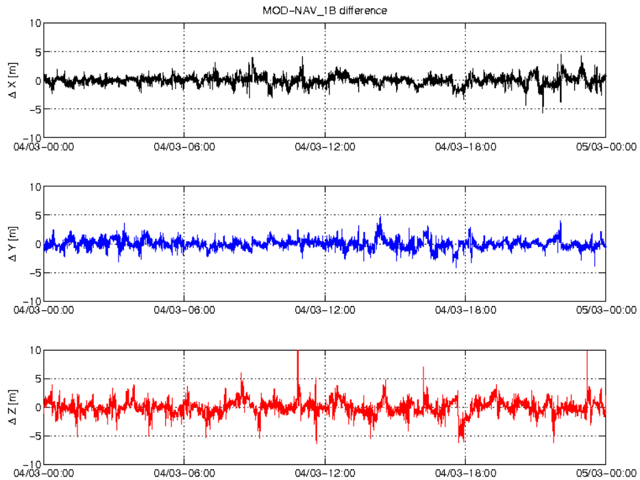
Figure 3-3: Difference MOD-GPSNAV, S/C A, 04.03. From top to bottom: X, Y and Z-axis
