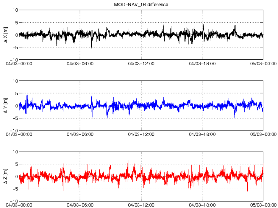
Figure 3-4: Difference MOD-GPSNAV, S/C B, 04.03. From top to bottom: X, Y and Z-axis
