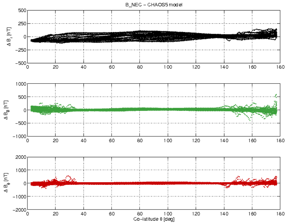
Figure 3-21: S/C C day 04.03 B_{NEC} - B_{Chaos} difference vs colatitude.
