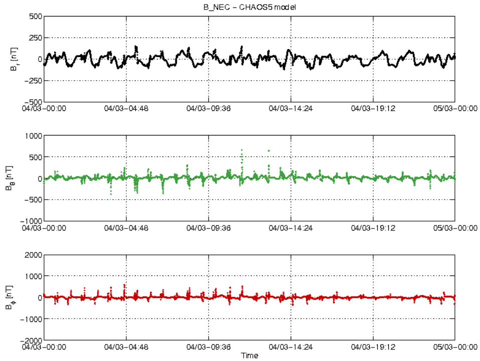
Figure 3-18: S/C A day 04.03: time series of B_{NEC} - B_{Chaos} residuals.
