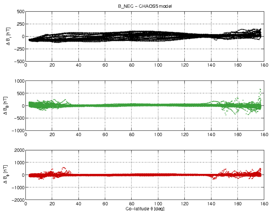
Figure 3-17: S/C A day 04.03 B_{NEC} - B_{Chaos} vs colatitude.
