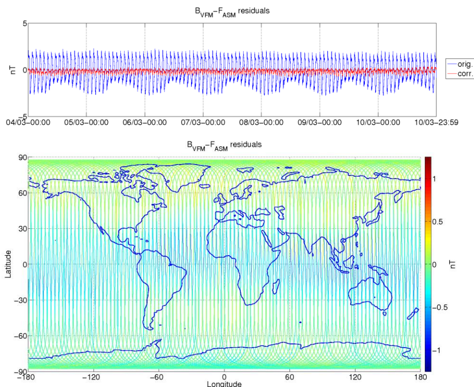
Figure 3-9: ASM-VFM residuals for S/C B, during monitoring period 04/03-10/03. In top figure are plotted: difference between |B_{VFM}| and F_{ASM} (without dB_{Sun} correction) (blue colour), and the residuals with dB_{Sun} corrections (red colour). In bottom figure residuals are presented on the world map.
