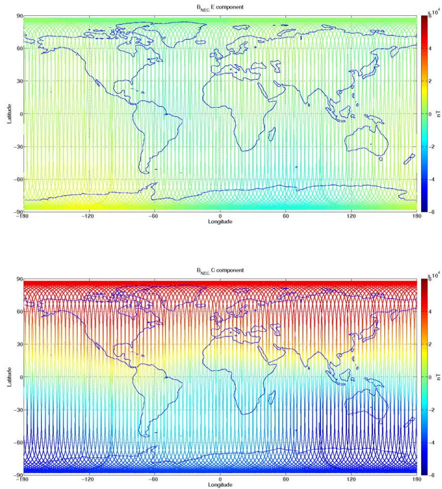
Figure 3-11: S/C B, world map plots of the geomagnetic field and components measured during monitoring period 25/02-03/03. From top to bottom: F-magnetic field from ASM measurement, B_{NEC} components (North, East, and Centre) of magnetic field from VFM measurement.
