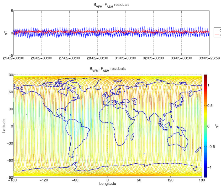
Figure 3-8: ASM-VFM residuals for S/C A, during monitoring period 25/02-03/03. In top figure are plotted: difference between |B_{VFM}| and F_{ASM} (without dB_{Sun} correction) (blue colour), and the residuals with dB_{Sun} corrections (red colour). In bottom figure residuals are presented on the world map.
