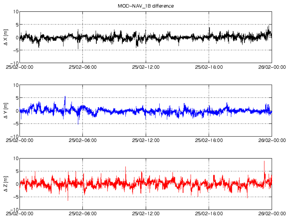
Figure 3-5: Difference MOD-GPSNAV, S/C C, 25.02. From top to bottom: X, Y and Z-axis
