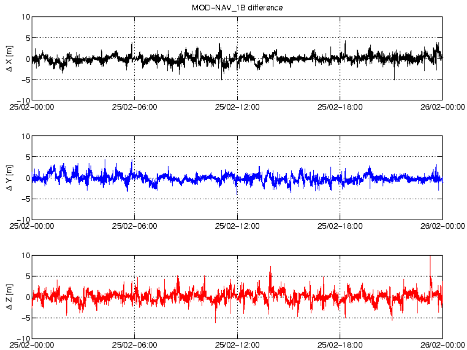
Figure 3-3: Difference MOD-GPSNAV, S/C A, 25.02. From top to bottom: X, Y and Z-axis
