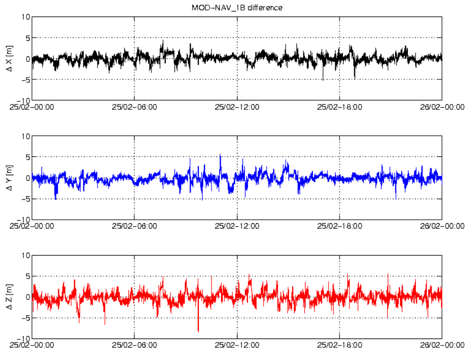
Figure 3-4: Difference MOD-GPSNAV, S/C B, 25.02. From top to bottom: X, Y and Z-axis
