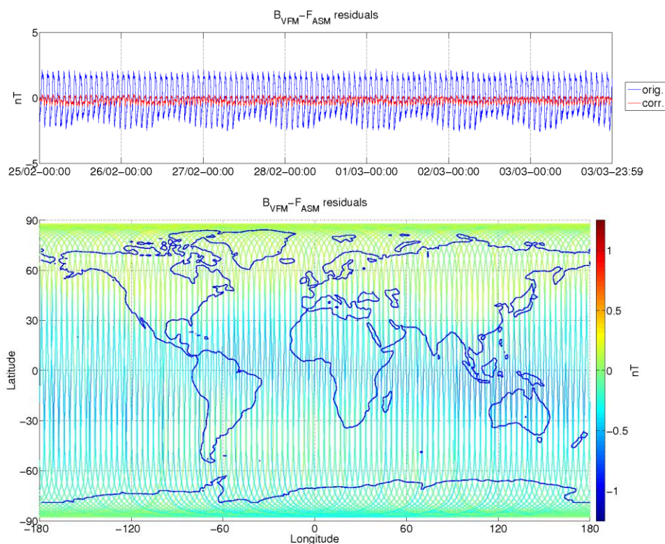
Figure 3-9: ASM-VFM residuals for S/C B, during monitoring period 25/02-03/03. In top figure are plotted: difference between |B\_VFM| and F\_ASM (without dB\_Sun correction) (blue colour), and the residuals with dB\_Sun corrections (red colour). In bottom figure residuals are presented on the world map.
