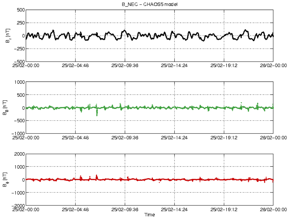
Figure 3-22: S/C C day 25.02 time series of B_{NEC} - B_{Chaos} residuals.
