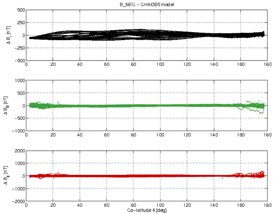
Figure 3-21: S/C C day 25.02 B_{NEC} - B_{Chaos} difference vs colatitude.
