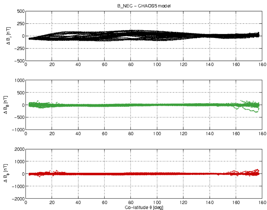
Figure 3-17: S/C A day 25.02 B_{NEC} - B_{Chaos5} vs colatitude.
