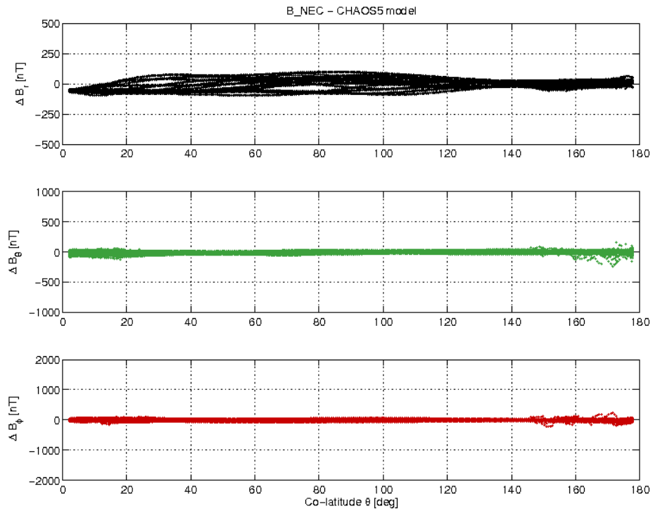
Figure 3-19: S/C B day 25.02 B_{NEC} - B_{Chaos} difference vs colatitude.
