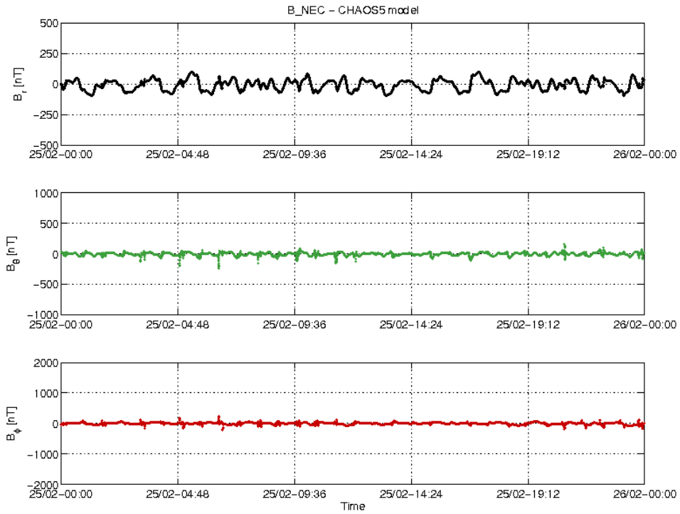
Figure 3-20: S/C B day 25.02 time series of B_{NEC} - B_{Chaos} residuals.
