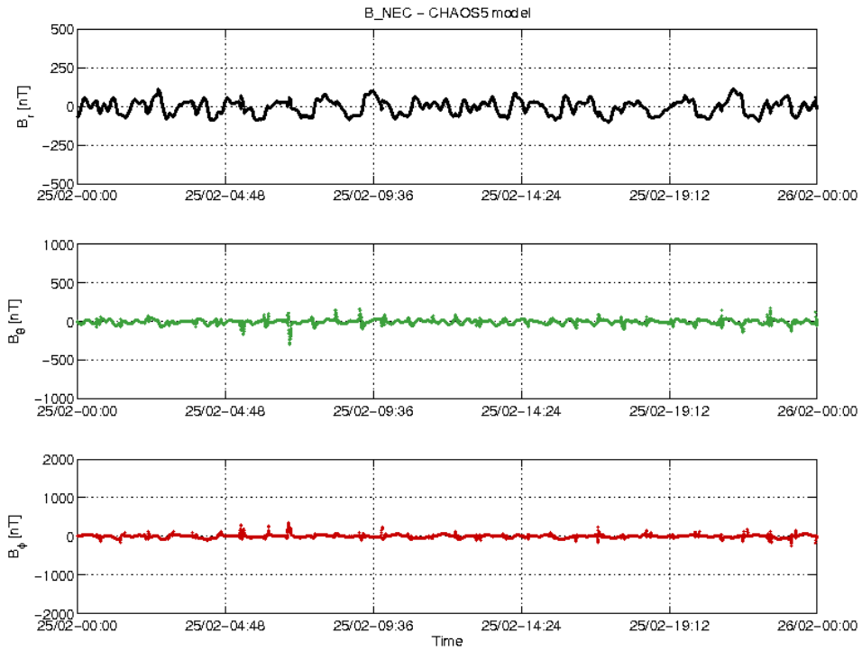
Figure 3-18: S/C A day 25.02: time series of B_{NEC} - B_{Chaos} residuals.
