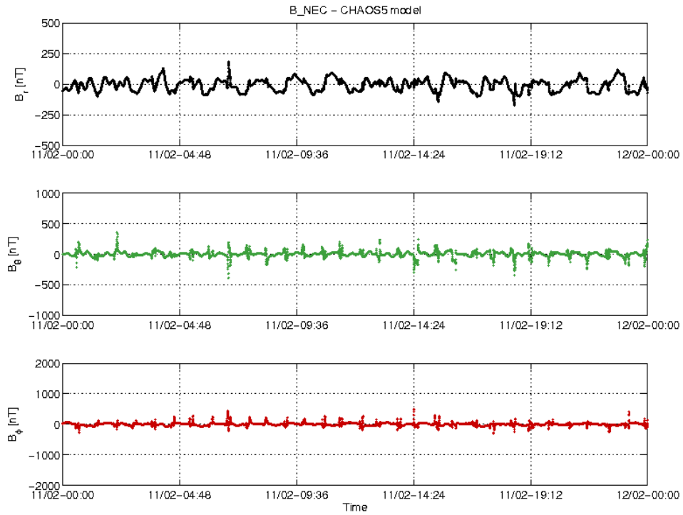
Figure 3-18: S/C A day 11.02: time series of B_{NEC} - B_{Chaos} residuals.
