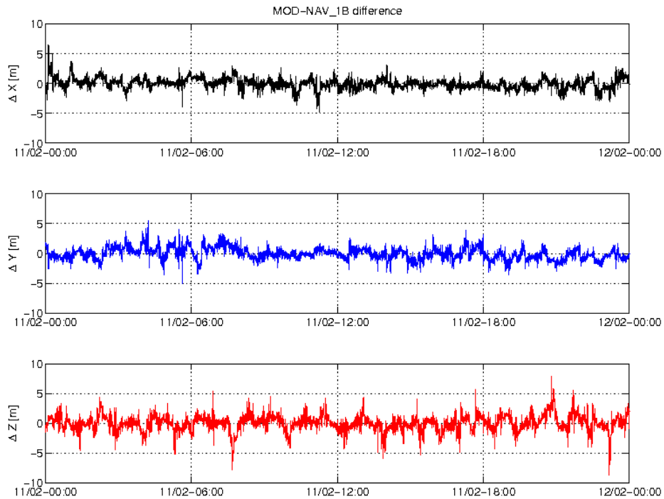
Figure 3-3: Difference MOD-GPSNAV, S/C A, 11.02. From top to bottom: X, Y and Z-axis
