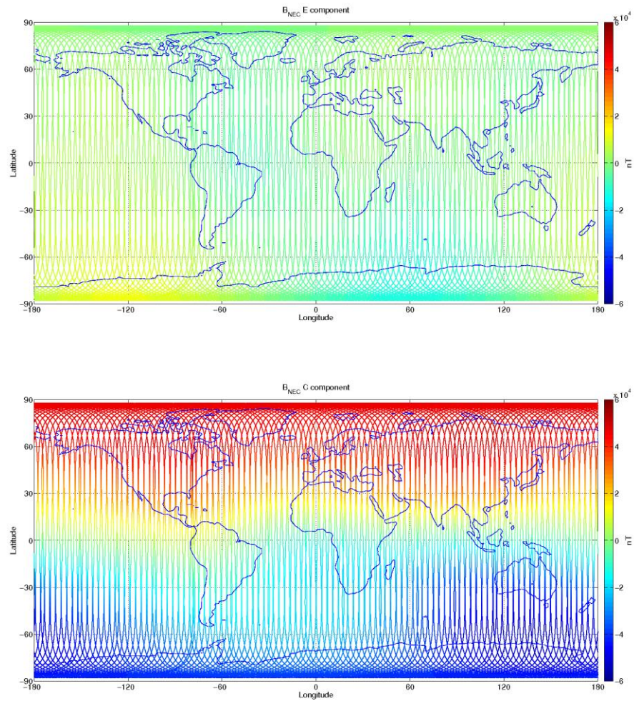
Figure 3-11: S/C B, world map plots of the geomagnetic field and components measured during monitoring period 11/02-17/02. From top to bottom: F-magnetic field from ASM measurement, B_{NEC} components (North, East, and Centre) of magnetic field from VFM measurement.
