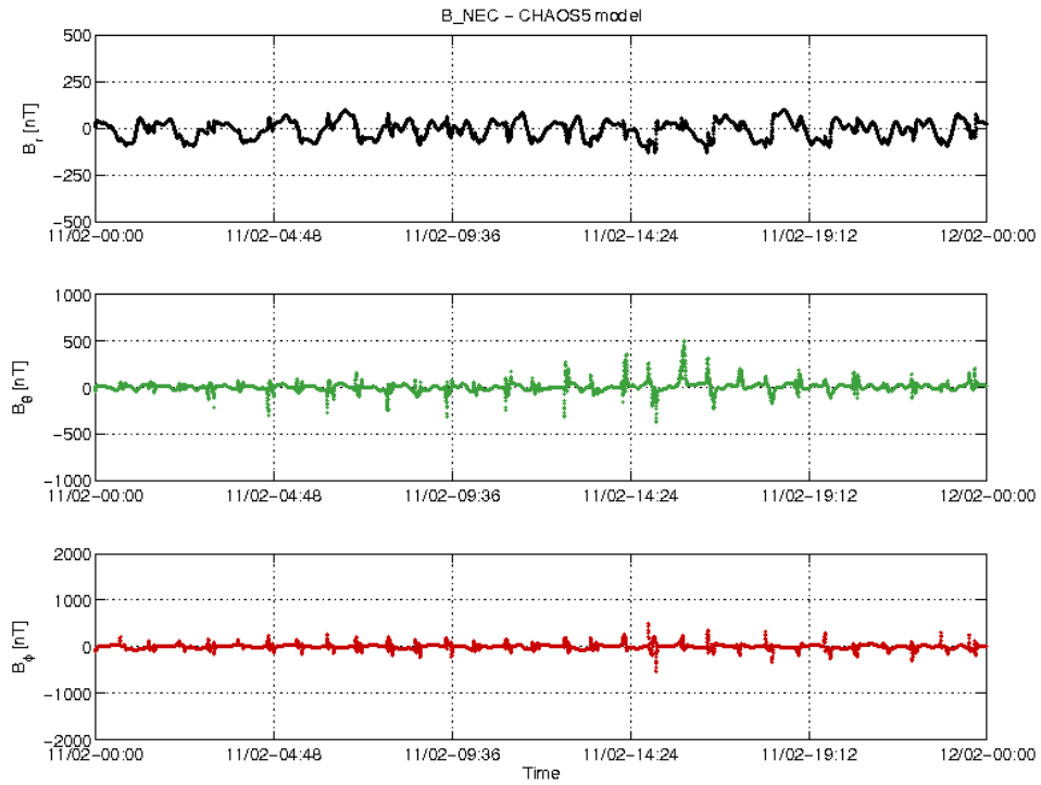
Figure 3-20: S/C B day 11.02 time series of B_{NEC} - B_{Chaos} residuals.
