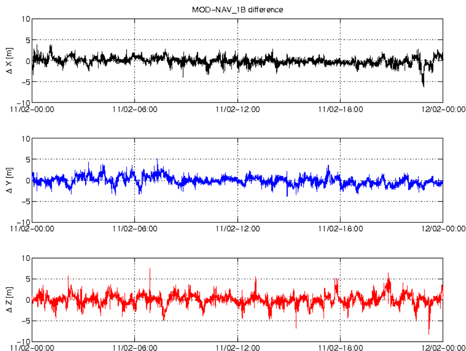
Figure 3-5: Difference MOD-GPSNAV, S/C C, 11.02. From top to bottom: X, Y and Z-axis
