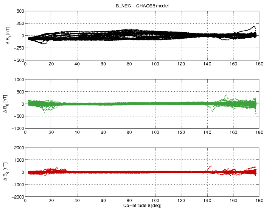
Figure 3-17: S/C A day 11.02 B_{NEC} - B_{Chaos} vs colatitude.
