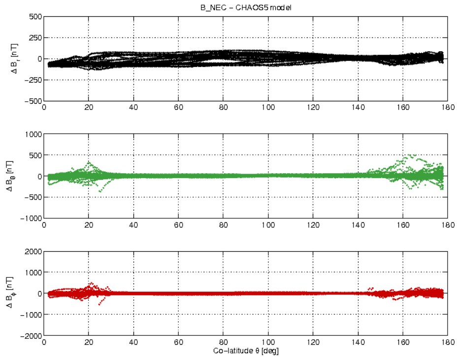
Figure 3-19: S/C B day 11.02 B_{NEC} - B_{Chaos} difference vs colatitude.
