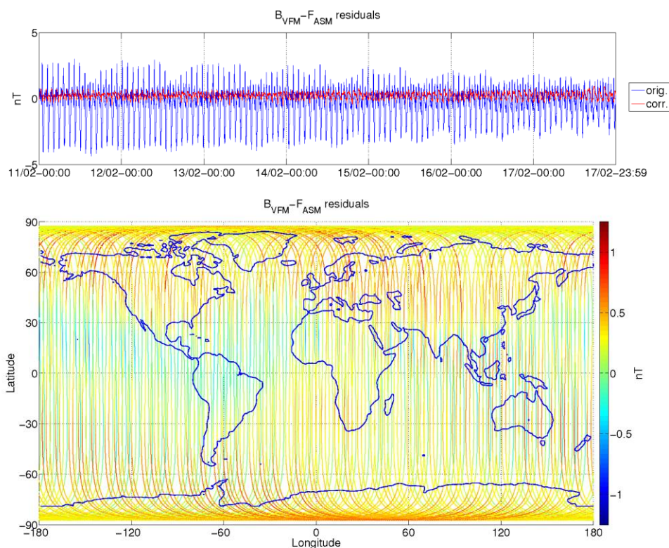
Figure 3-8: ASM-VFM residuals for S/C A, during monitoring period 11/02-17/02. In top figure are plotted: difference between |B_{VFM}| and F_{ASM} (without dB_{Sun} correction) (blue colour), and the residuals with dB_{Sun} corrections (red colour). In bottom figure residuals are presented on the world map.
