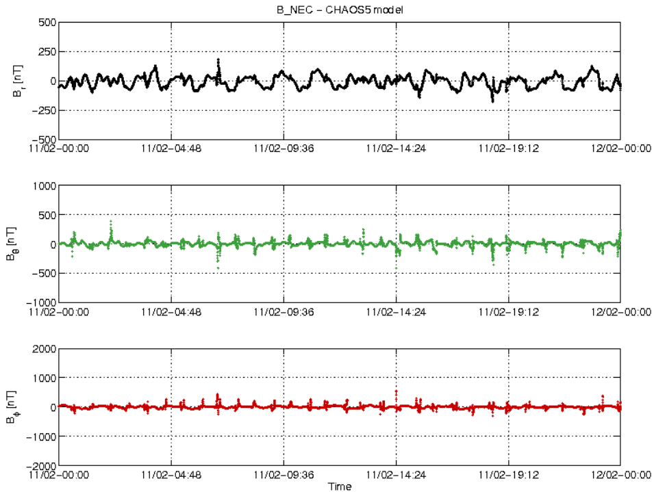
Figure 3-22: S/C C day 11.02 time series of B_{NEC} - B_{Chaos} residuals.
