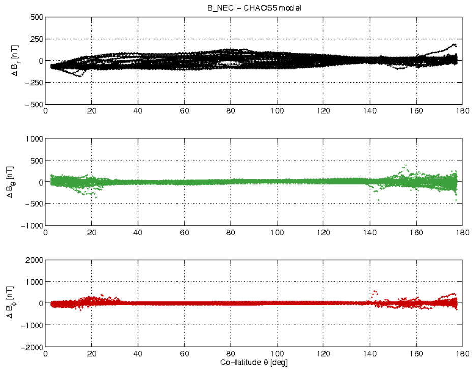
Figure 3-21: S/C C day 11.02 B_{NEC} - B_{Chaos} difference vs colatitude.
