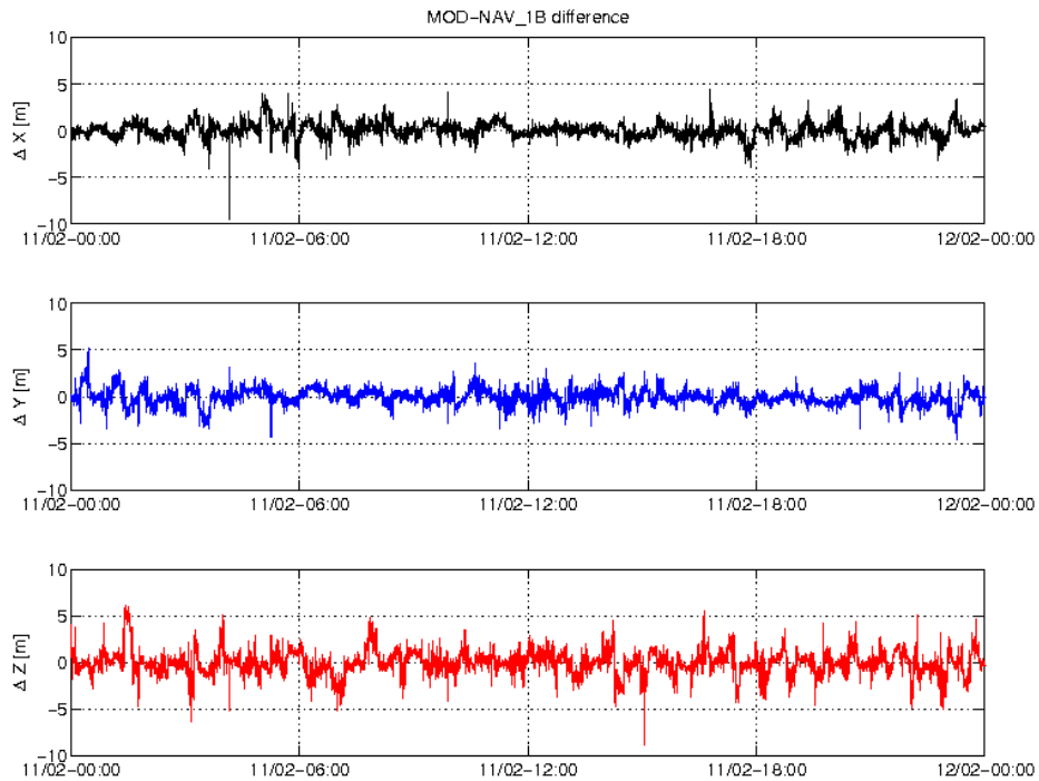
Figure 3-4: Difference MOD-GPSNAV, S/C B, 11.02. From top to bottom: X, Y and Z-axis
