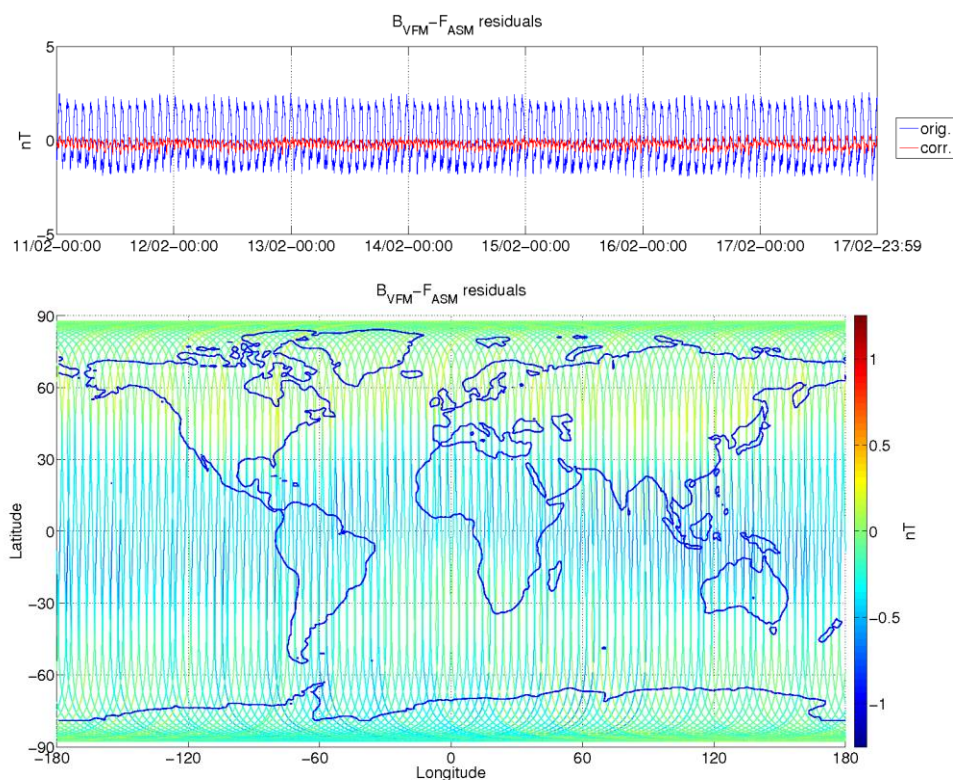
Figure 3-9: ASM-VFM residuals for S/C B, during monitoring period 11/02-17/02. In top figure are plotted: difference between |B_{VFM}| and F_{ASM} (without dB_{Sun} correction) (blue colour), and the residuals with dB_{Sun} corrections (red colour). In bottom figure residuals are presented on the world map.
