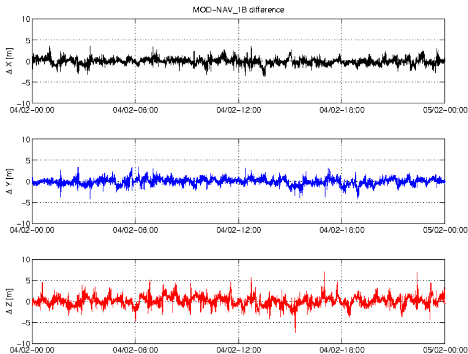
Figure 3-5: Difference MOD-GPSNAV, S/C C, 04.02. From top to bottom: X, Y and Z-axis
