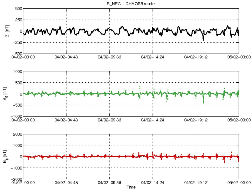
Figure 3-18: S/C A day 04.02: time series of B_{NEC} - B_{Chaos} residuals.
