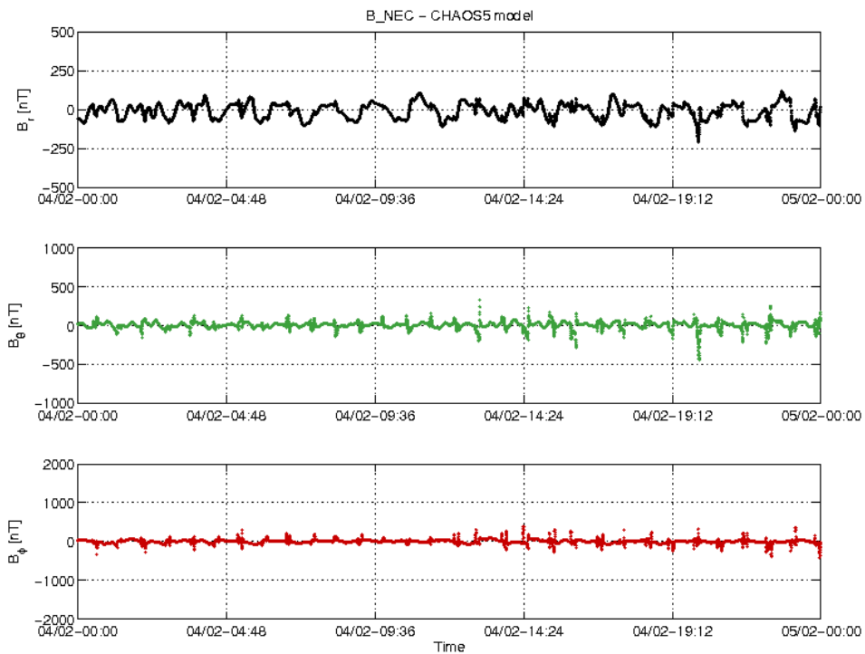
Figure 3-22: S/C C day 04.02 time series of B_{NEC} - B_{Chaos} residuals.
