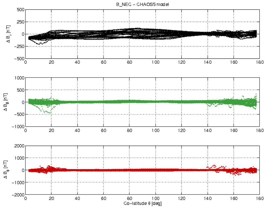
Figure 3-21: S/C C day 04.02 B_{NEC} - B_{Chaos} difference vs colatitude.
