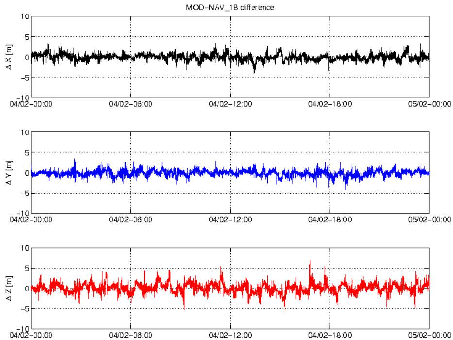
Figure 3-3: Difference MOD-GPSNAV, S/C A, 04.02. From top to bottom: X, Y and Z-axis
