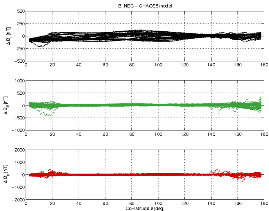
Figure 3-17: S/C A day 04.02 B_{NEC} - B_{Chaos} vs colatitude.
