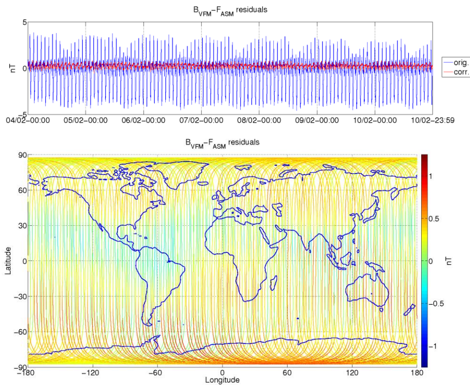
Figure 3-8: ASM-VFM residuals for S/C A, during monitoring period 04/02-10/02. In top figure are plotted: difference between |B_{VFM}| and F_{ASM} (without dB_{Sun} correction) (blue colour), and the residuals with dB_{Sun} corrections (red colour). In bottom figure residuals are presented on the world map.
