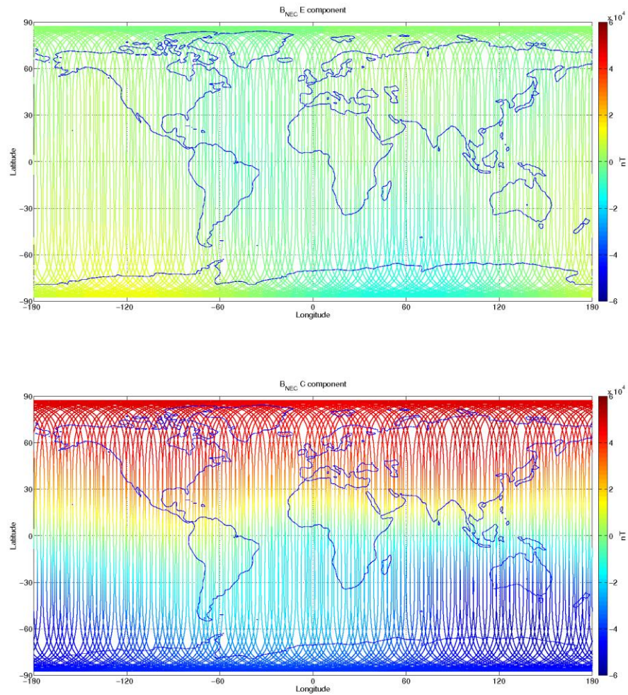
Figure 3-10: S/C A, world map plots of the geomagnetic field and components measured during monitoring period 04/02-10/02. From top to bottom: F-magnetic field from ASM measurement, B NEC components (North, East, and Centre) of magnetic field from VFM measurement.
