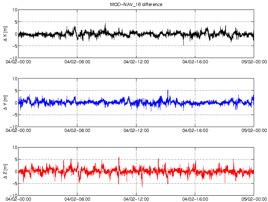
Figure 3-4: Difference MOD-GPSNAV, S/C B, 04.02. From top to bottom: X, Y and Z-axis
