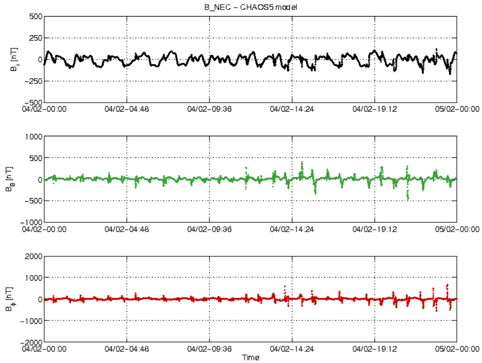
Figure 3-20: S/C B day 04.02 time series of B_{NEC} - B_{Chaos} residuals.
