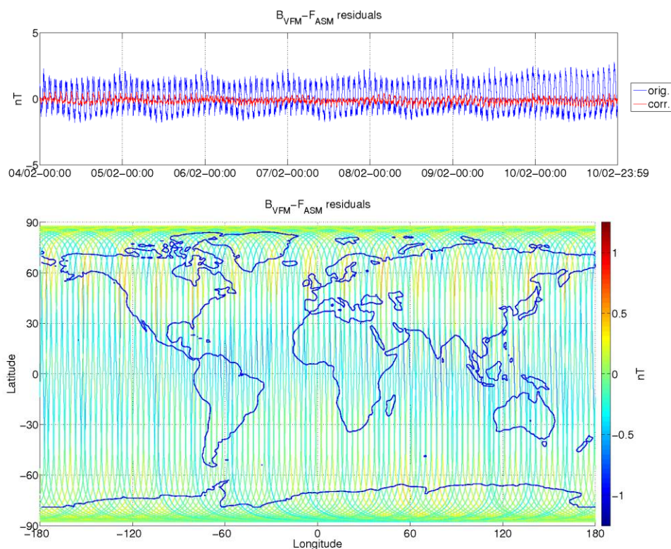
Figure 3-9: ASM-VFM residuals for S/C B, during monitoring period 04/02-10/02. In top figure are plotted: difference between |B_{VFM}| and F_{ASM} (without dB_{Sun} correction) (blue colour), and the residuals with dB_{Sun} corrections (red colour). In bottom figure residuals are presented on the world map.
