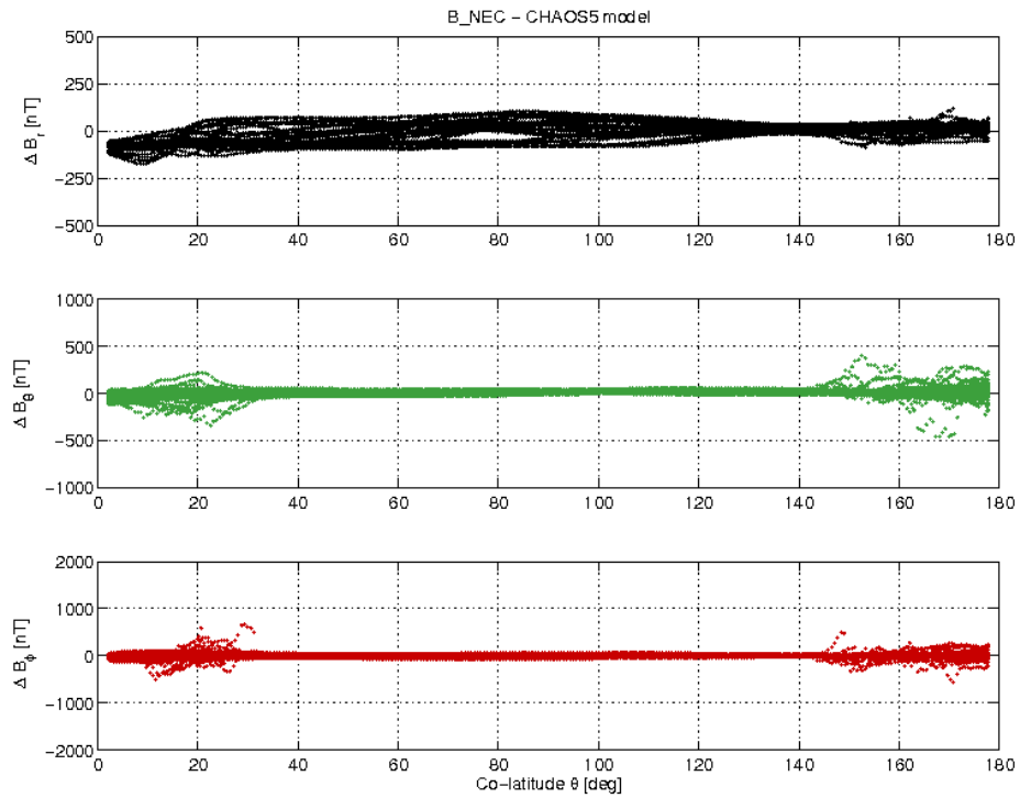
Figure 3-19: S/C B day 04.02 B_{NEC} - B_{Chaos} difference vs colatitude.
