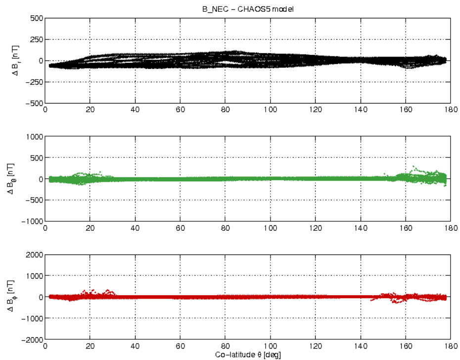
Figure 3-19: S/C B day 21.01 B_{\text{NEC}} - B_{\text{Chaos}} difference vs colatitude.
