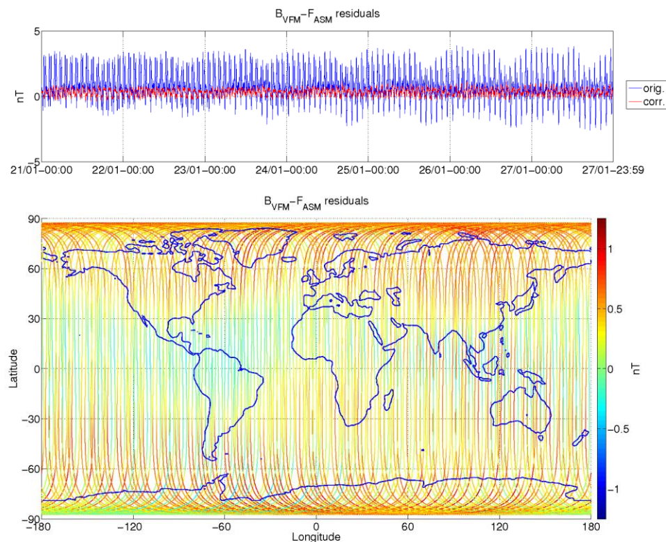
Figure 3-8: ASM-VFM residuals for S/C A, during monitoring period 21/01-27/01. In top figure are plotted: difference between |B_{VFM}| and F_{ASM} (without dB_Sun correction) (blue colour), and the residuals with dB_Sun corrections (red colour). In bottom figure residuals are presented on the world map.
