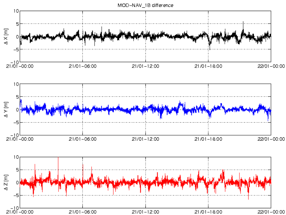
Figure 3-4: Difference MOD-GPSNAV, S/C B, 21.01. From top to bottom: X, Y and Z-axis
