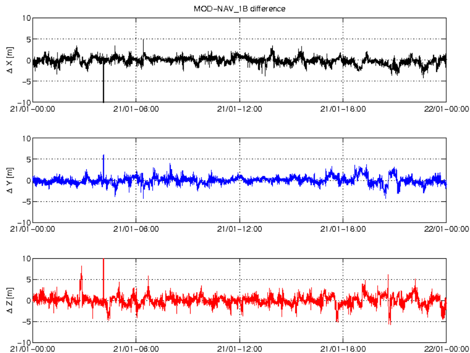
Figure 3-5: Difference MOD-GPSNAV, S/C C, 21.01. From top to bottom: X, Y and Z-axis
