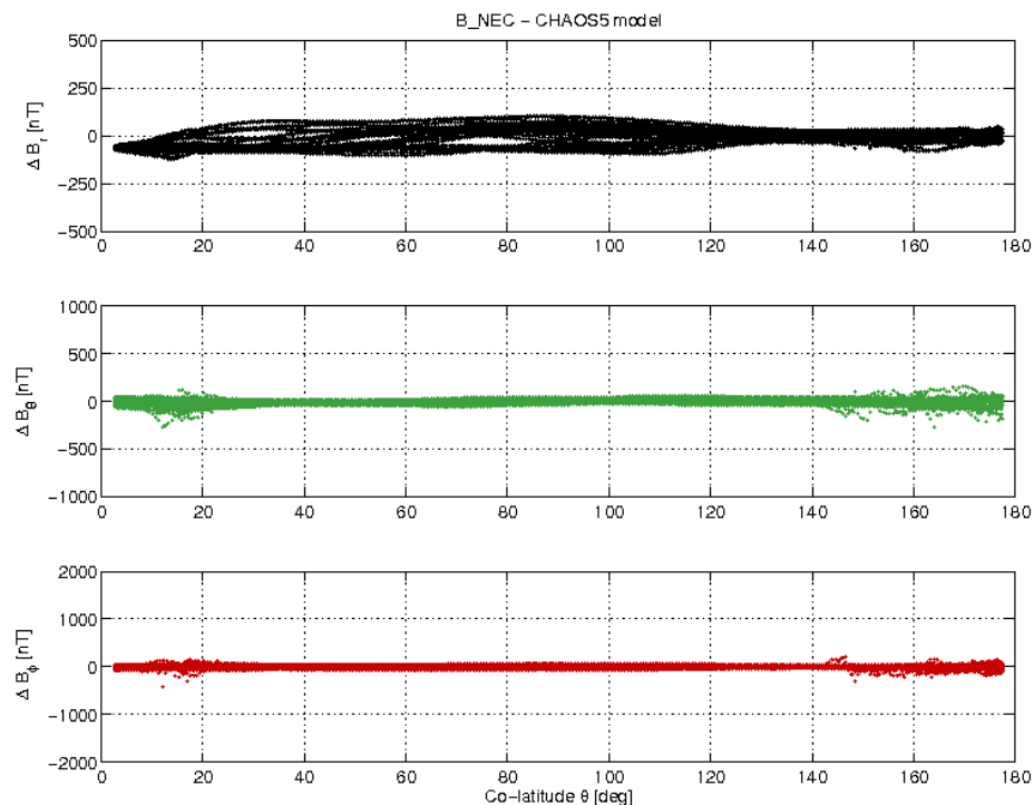
Figure 3-17: S/C A day 21.01 B_{NEC} - B_{Chaos} vs colatitude.
