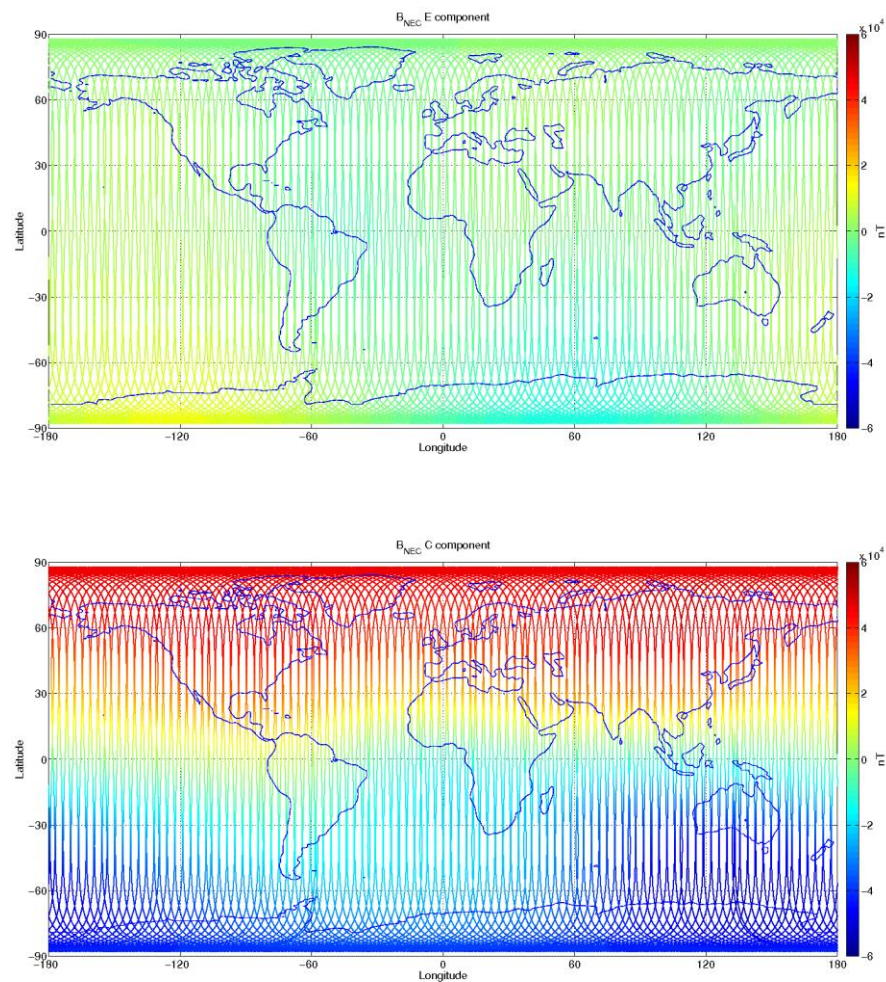
Figure 3-11: S/C B, world map plots of the geomagnetic field and components measured during monitoring period 21/01-27/01. From top to bottom: F-magnetic field from ASM measurement, B_{NEC} components (North, East, and Centre) of magnetic field from VFM measurement.
