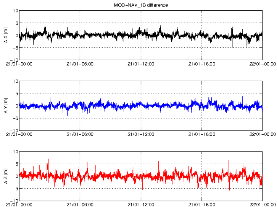
Figure 3-3: Difference MOD-GPSNAV, S/C A, 21.01. From top to bottom: X, Y and Z-axis
