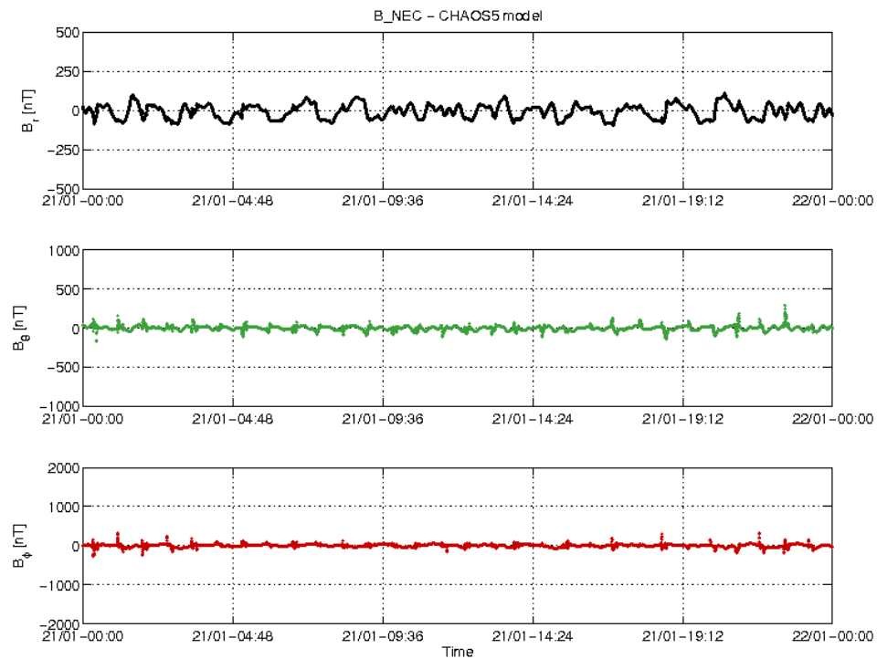
Figure 3-20: S/C B day 21.01 time series of B_{NEC} - B_{Chaos} residuals.
