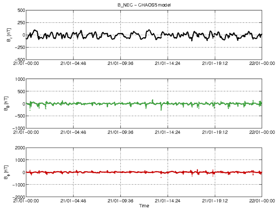
Figure 3-18: S/C A day 21.01: time series of B_{NEC} - B_{Chaos} residuals.
