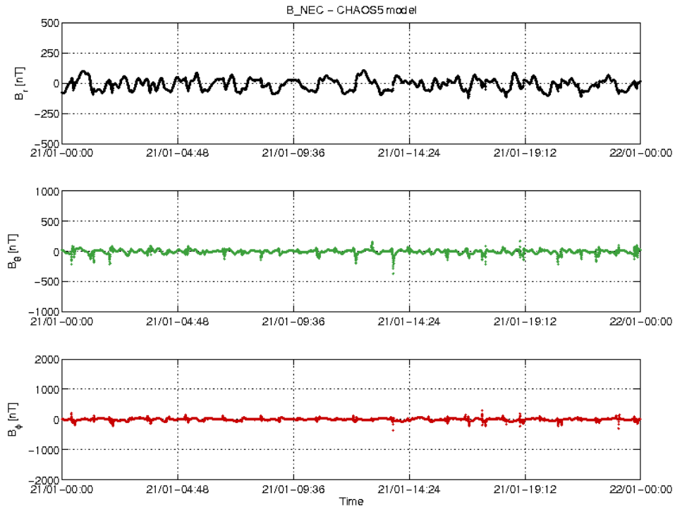
Figure 3-22: S/C C day 21.01 time series of B_{NEC} - B_{\text{Chaos}} residuals.
