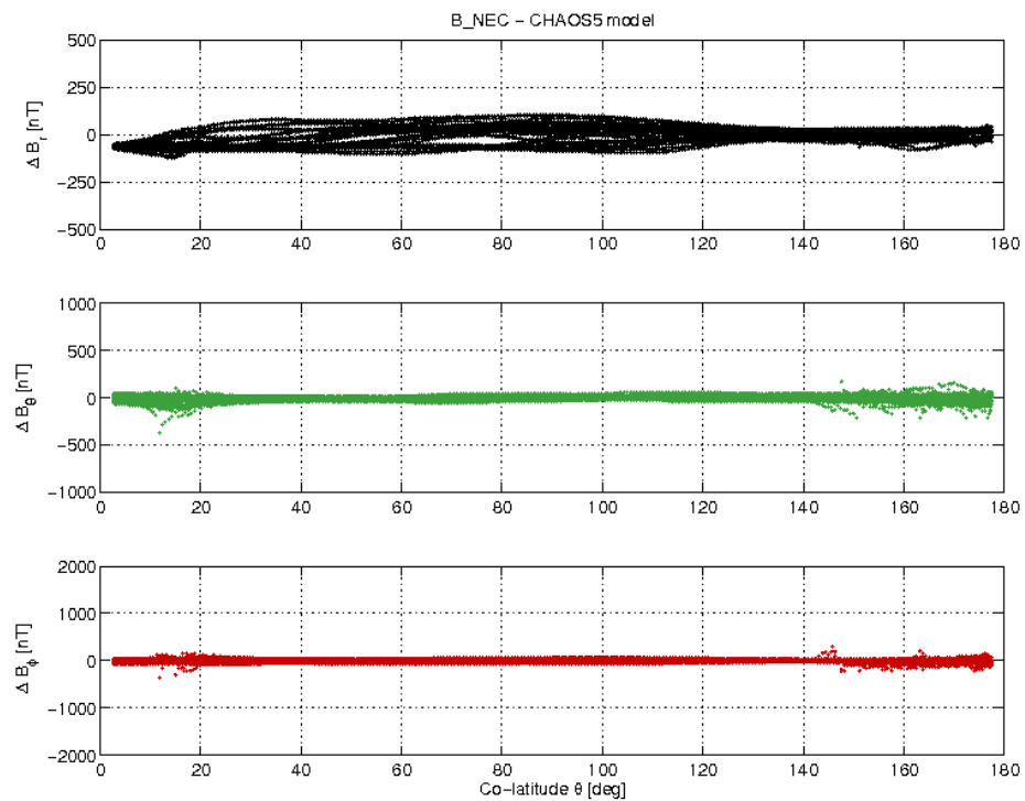
Figure 3-21: S/C C day 21.01 B_{NEC} - B_{Chaos} difference vs colatitude.
