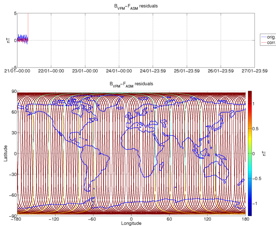
Figure 3-9: ASM-VFM residuals for S/C B, during monitoring period 21/01-27/01. In top figure are plotted: difference between |B_{VFM}| and F_{ASM} (without dB_Sun correction) (blue colour), and the residuals with dB_Sun corrections (red colour). In bottom figure residuals are presented on the world map.
