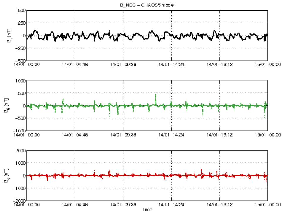
Figure 3-18: S/C A day 14.01: time series of B_{NEC} - B_{Chaos} residuals.
