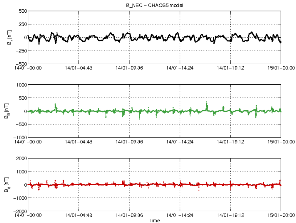
Figure 3-20: S/C B day 14.01 time series of B_{NEC} - B_{Chaos} residuals.
