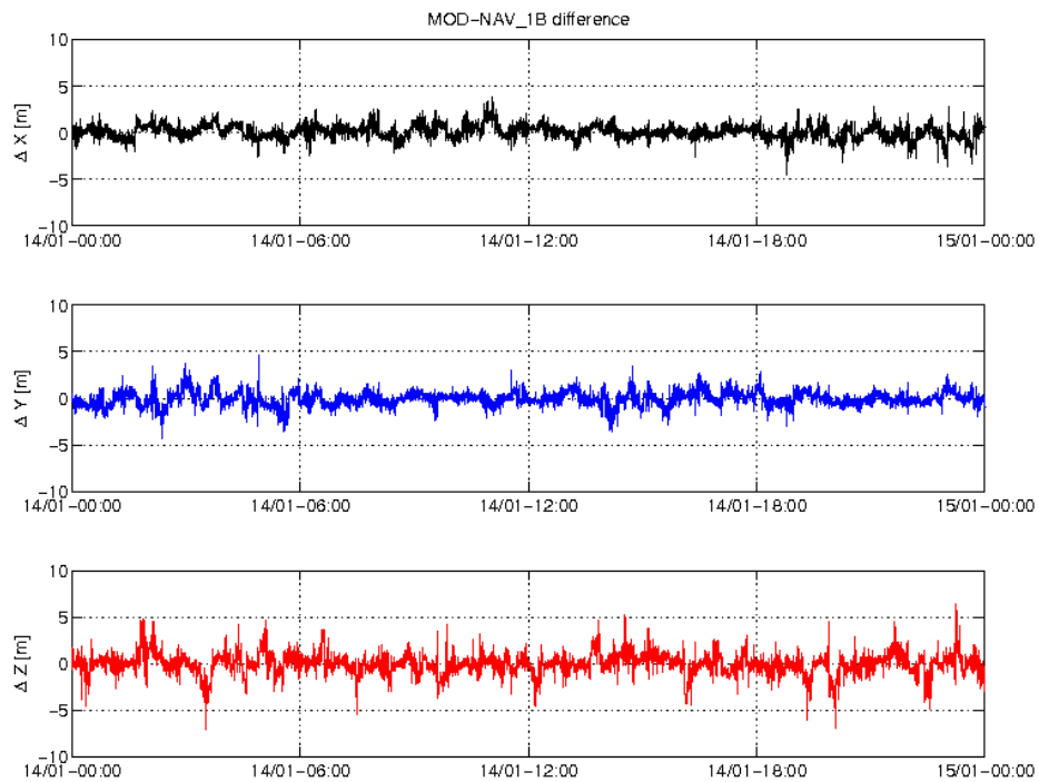
Figure 3-4: Difference MOD-GPSNAV, S/C B, 14.01. From top to bottom: X, Y and Z-axis
