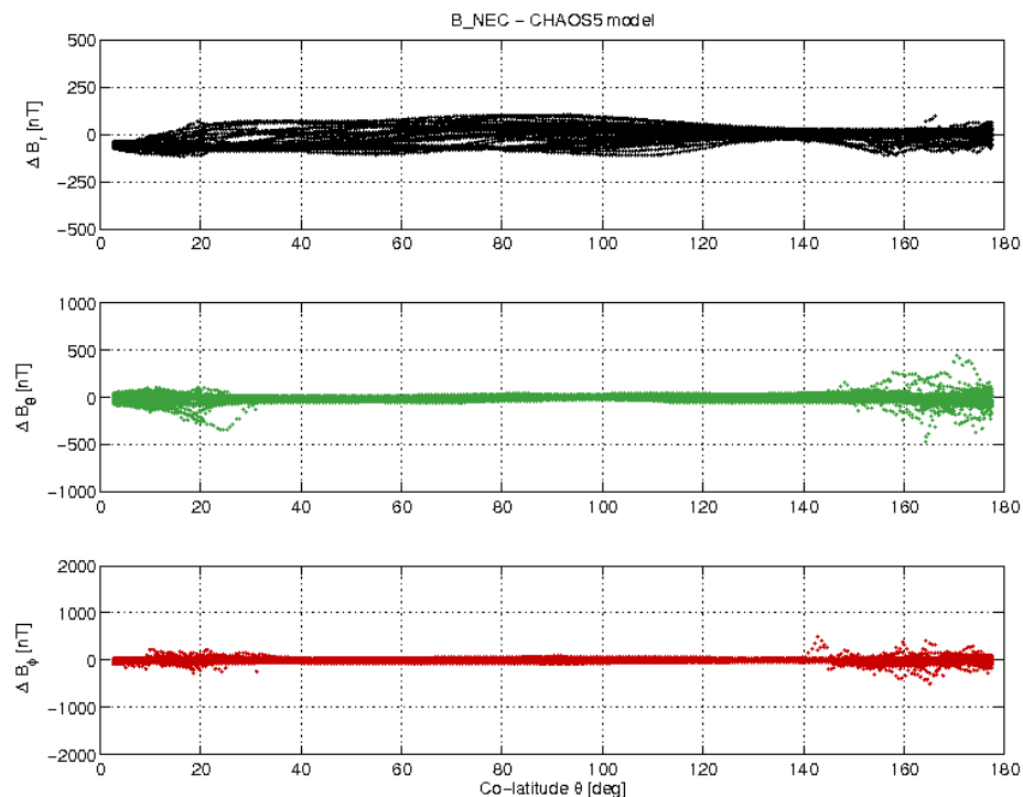
Figure 3-17: S/C A day 14.01 B_{NEC} - B_{Chaos} vs colatitude.
