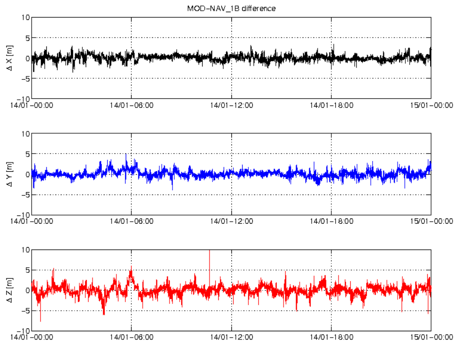
Figure 3-3: Difference MOD-GPSNAV, S/C A, 14.01. From top to bottom: X, Y and Z-axis
