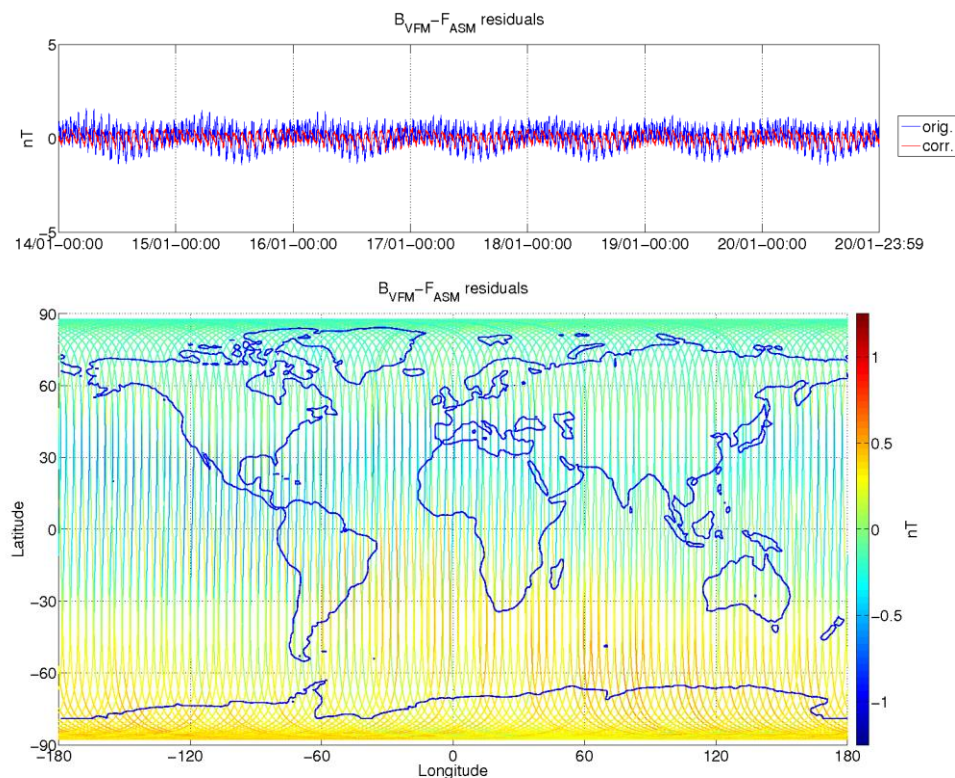
Figure 3-9: ASM-VFM residuals for S/C B, during monitoring period 14/01-20/01. In top figure are plotted: difference between |B_{VFM}| and F_{ASM} (without dB_Sun correction) (blue colour), and the residuals with dB_Sun corrections (red colour). In bottom figure residuals are presented on the world map.
