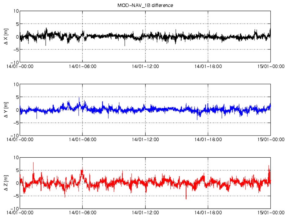
Figure 3-5: Difference MOD-GPSNAV, S/C C, 14.01. From top to bottom: X, Y and Z-axis
