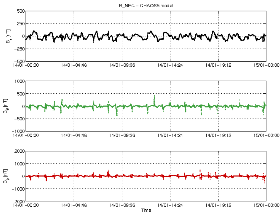
Figure 3-22: S/C C day 14.01 time series of B_{\text{NEC}} - B_{\text{Chaos}} residuals.
