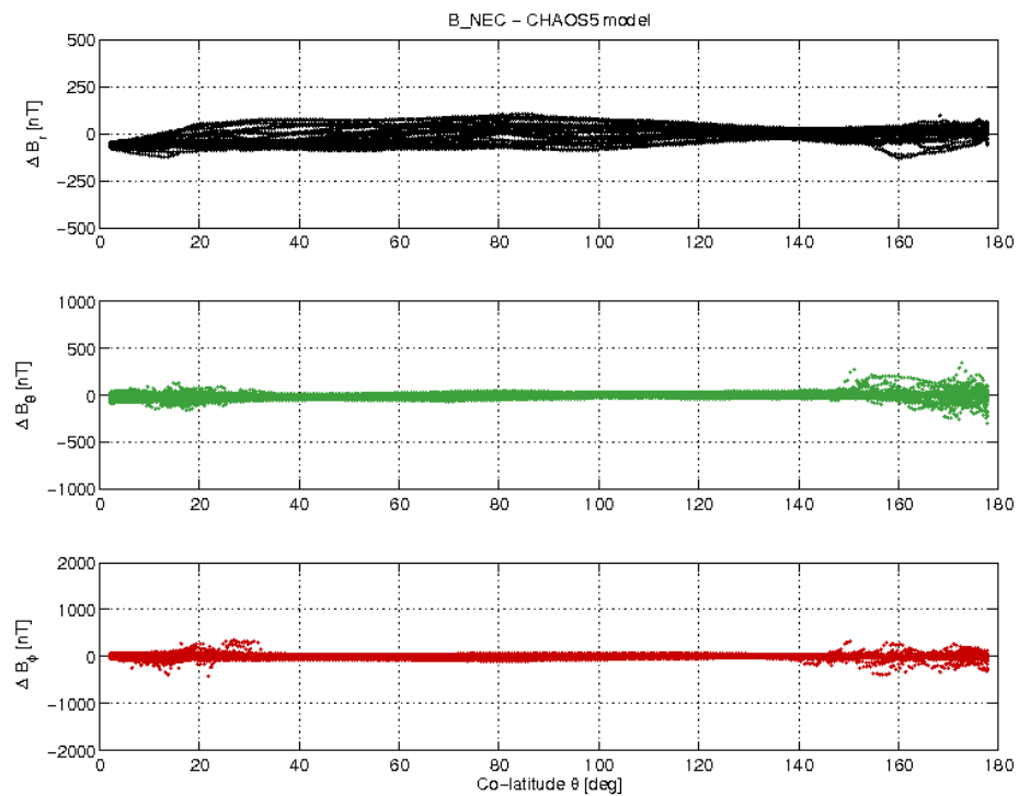
Figure 3-19: S/C B day 14.01 B_{\text{NEC}} - B_{\text{Chaos}} difference vs colatitude.
