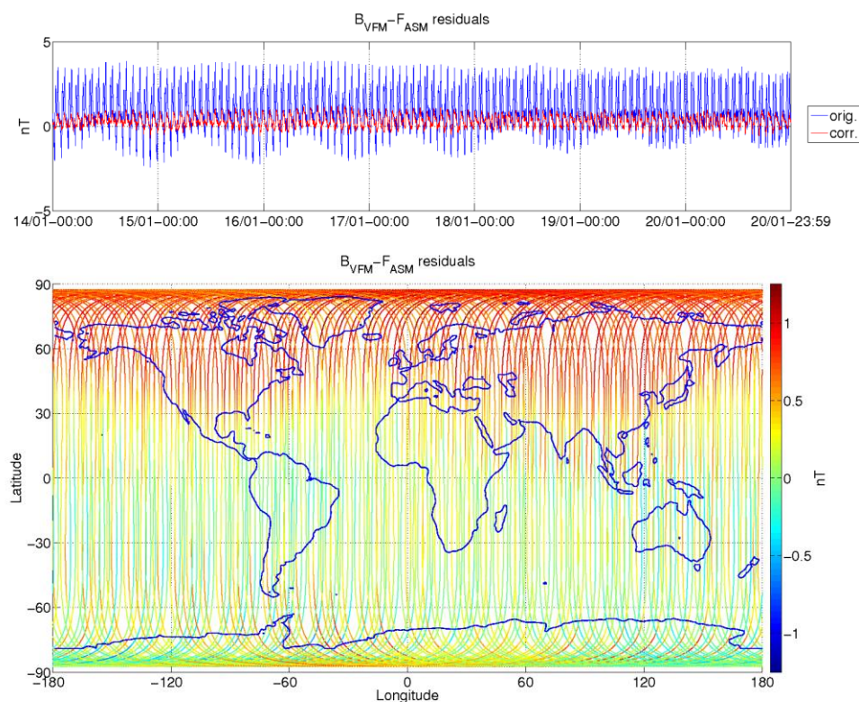
Figure 3-8: ASM-VFM residuals for S/C A, during monitoring period 14/01-20/01. In top figure are plotted: difference between |B_{VFM}| and F_{ASM} (without dB_{Sun} correction) (blue colour), and the residuals with dB_{Sun} corrections (red colour). In bottom figure residuals are presented on the world map.
