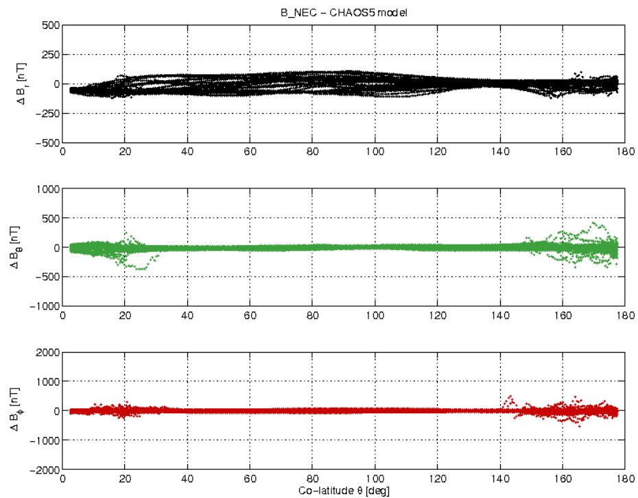
Figure 3-21: S/C C day 14.01 B_{NEC} - B_{Chaos} difference vs colatitude.
