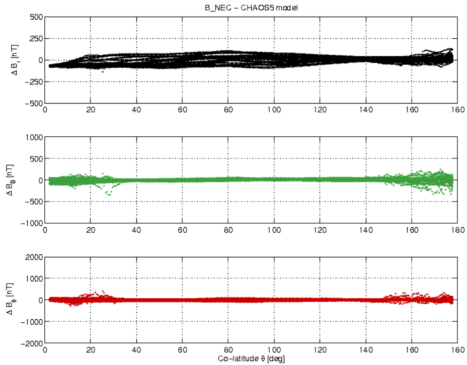
Figure 3-19: S/C B day 07.01 B_{NEC} - B_{Chaos} difference vs colatitude.
