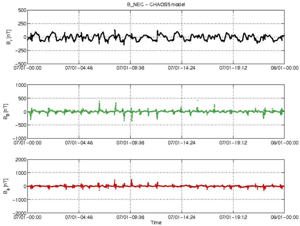
Figure 3-18: S/C A day 07.01: time series of B_{NEC} - B_{Chaos} residuals.
