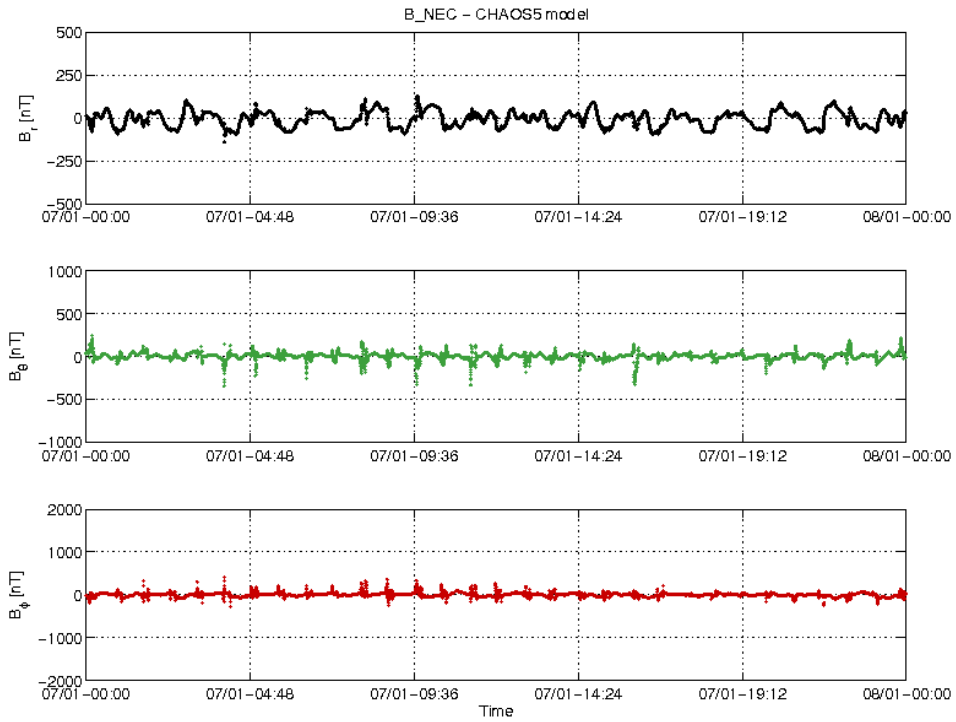
Figure 3-20: S/C B day 07.01 time series of B_{NEC} - B_{Chaos} residuals.
