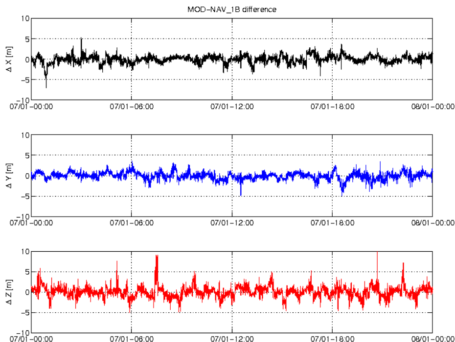
Figure 3-5: Difference MOD-GPSNAV, S/C C, 07.01. From top to bottom: X, Y and Z-axis
