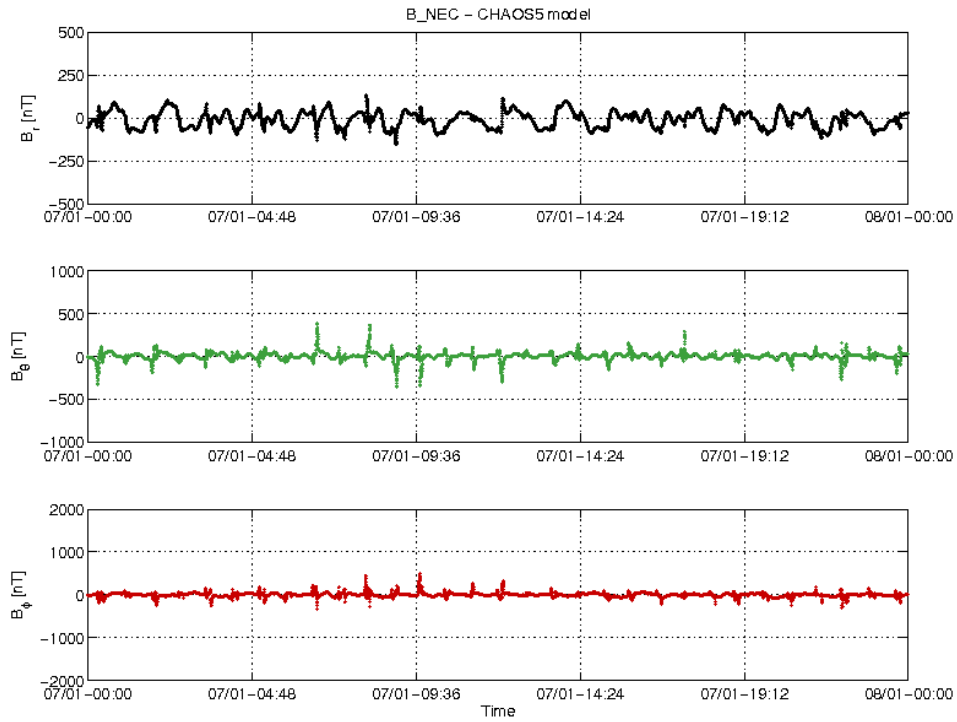
Figure 3-22: S/C C day 07.01 time series of B_{NEC} - B_{Chaos} residuals.
