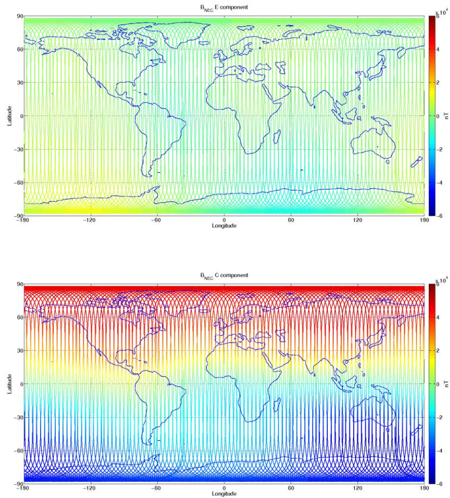
Figure 3-11: S/C B, world map plots of the geomagnetic field and components measured during monitoring period 07/01-13/01. From top to bottom: F-magnetic field from ASM measurement, B_{NEC} components (North, East, and Centre) of magnetic field from VFM measurement.
