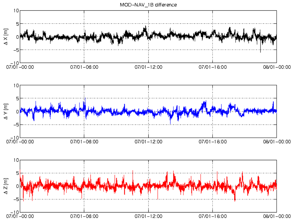
Figure 3-4: Difference MOD-GPSNAV, S/C B, 07.01. From top to bottom: X, Y and Z-axis
