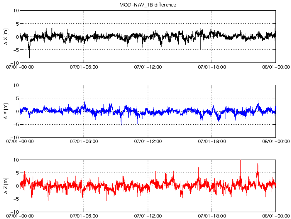
Figure 3-3: Difference MOD-GPSNAV, S/C A, 07.01. From top to bottom: X, Y and Z-axis
