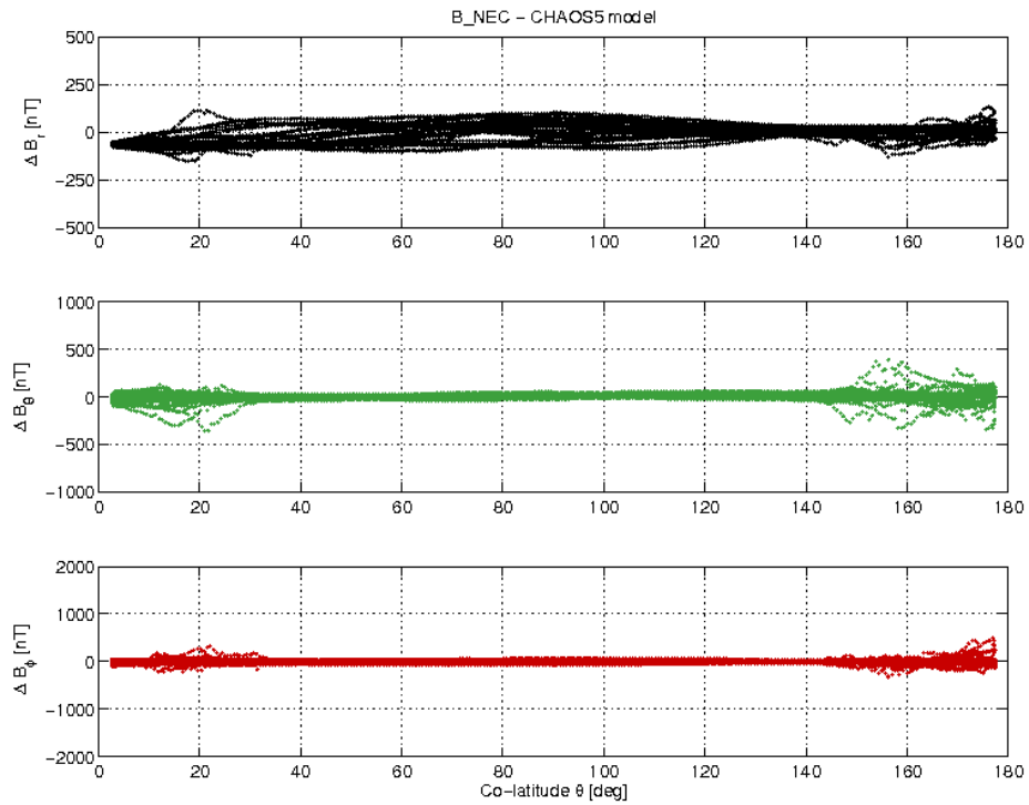
Figure 3-21: S/C C day 07.01 B_{NEC} - B_{Chaos} difference vs colatitude.
