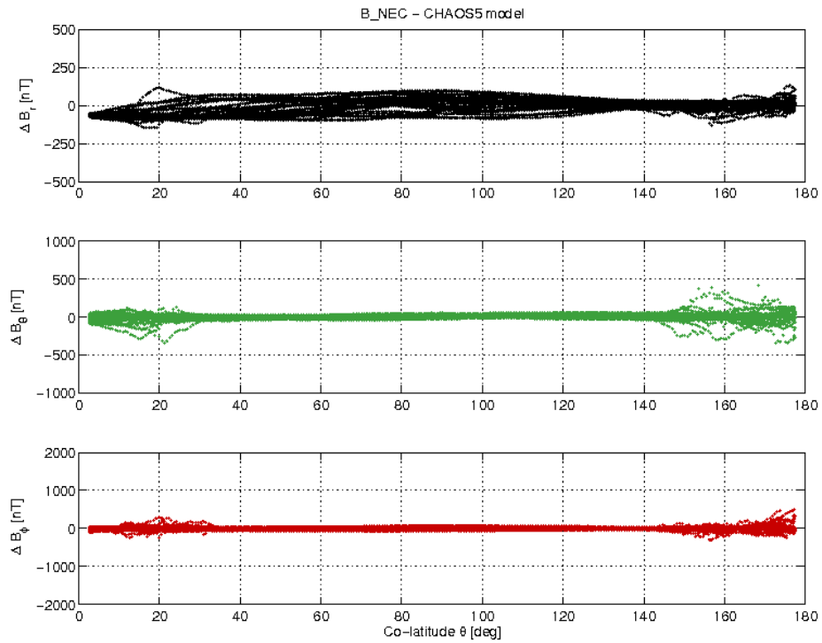
Figure 3-17: S/C A day 07.01 B_{NEC} - B_{Chaos} vs colatitude.
