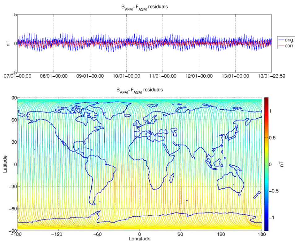
Figure 3-9: ASM-VFM residuals for S/C B, during monitoring period 07/01-13/01. In top figure are plotted: difference between |B_{VFM}| and F_{ASM} (without dB_Sun correction) (blue colour), and the residuals with dB_Sun corrections (red colour). In bottom figure residuals are presented on the world map.
