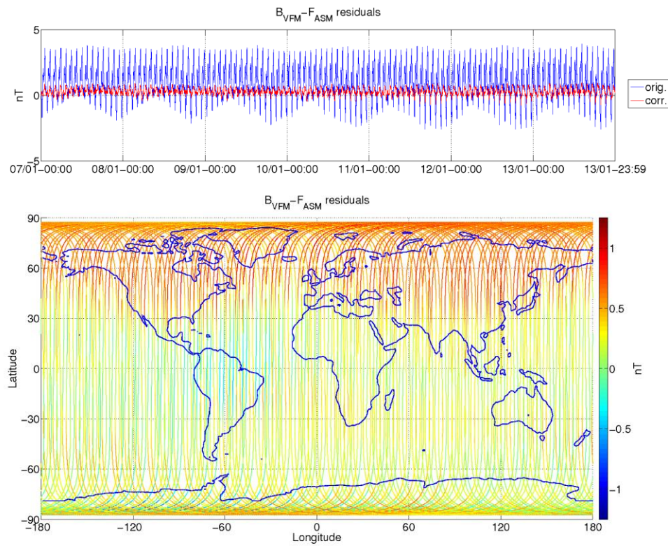
Figure 3-8: ASM-VFM residuals for S/C A, during monitoring period 07/01-13/01. In top figure are plotted: difference between |B VFM | and F ASM (without dB_Sun correction) (blue colour), and the residuals with dB_Sun corrections (red colour). In bottom figure residuals are presented on the world map.
