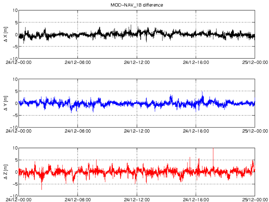
Figure 3-4: Difference MOD-GPSNAV, S/C B, 24.12. From top to bottom: X, Y and Z-axis
