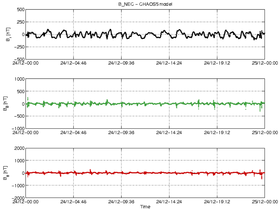
Figure 3-22: S/C C day 24.12 time series of B_{NEC} - B_{\text{Chaos}} residuals.
