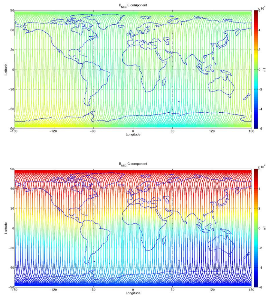
Figure 3-11: S/C B, world map plots of the geomagnetic field and components measured during monitoring period 24/12-30/12. From top to bottom: F-magnetic field from ASM measurement, B_{NEC} components (North, East, and Centre) of magnetic field from VFM measurement.
