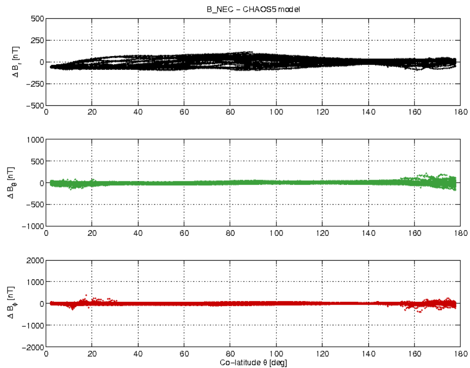
Figure 3-19: S/C B day 24.12 B_{NEC} - B_{CHAOS5} difference vs colatitude.
