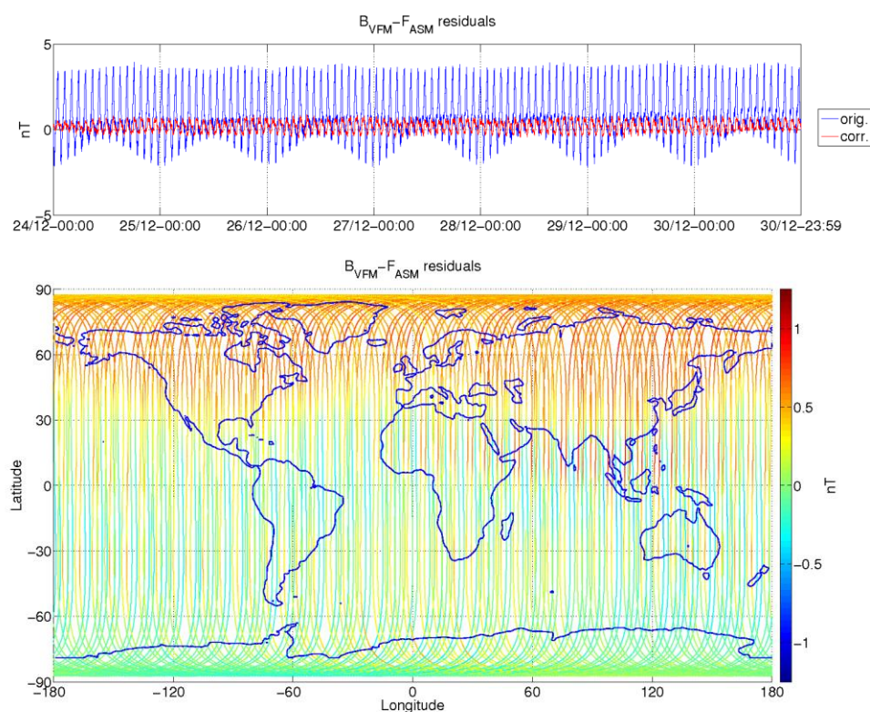
Figure 3-8: ASM-VFM residuals for S/C A, during monitoring period 24/12-30/12. In top figure are plotted: difference between |B_{VFM}| and F_{ASM} (without dB_{Sun} correction) (blue colour), and the residuals with dB_{Sun} corrections (red colour). In bottom figure residuals are presented on the world map.
