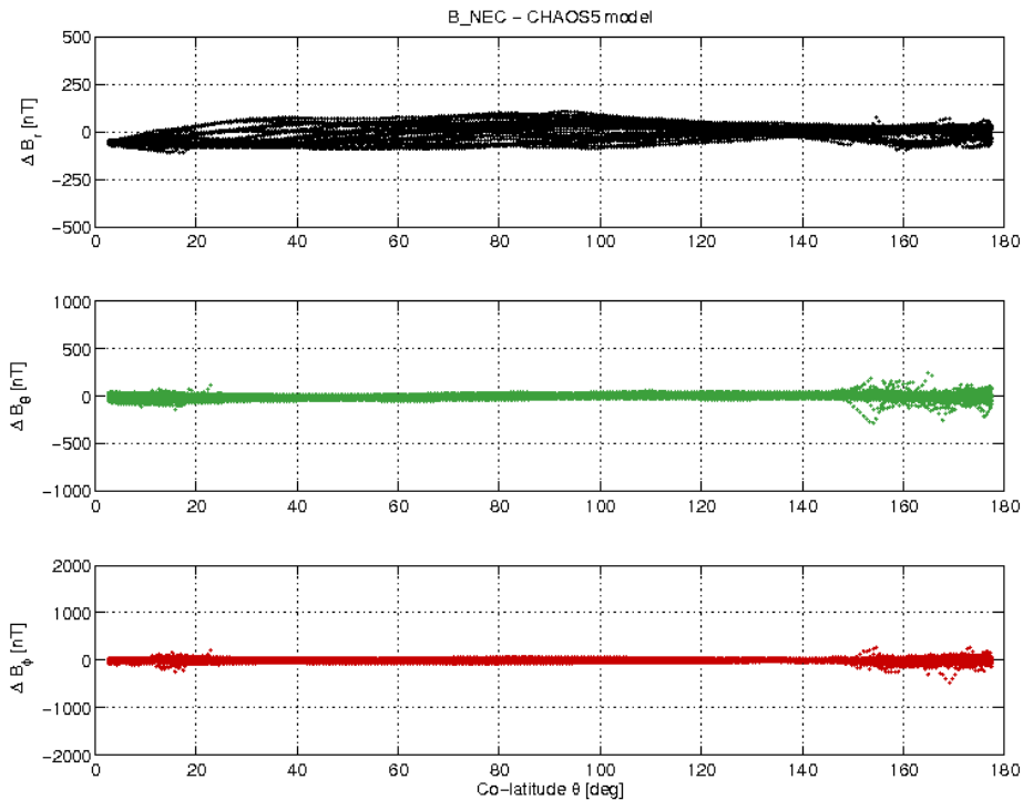
Figure 3-17: S/C A day 24.12 B_{NEC} - B_{Chaos5} vs colatitude.
