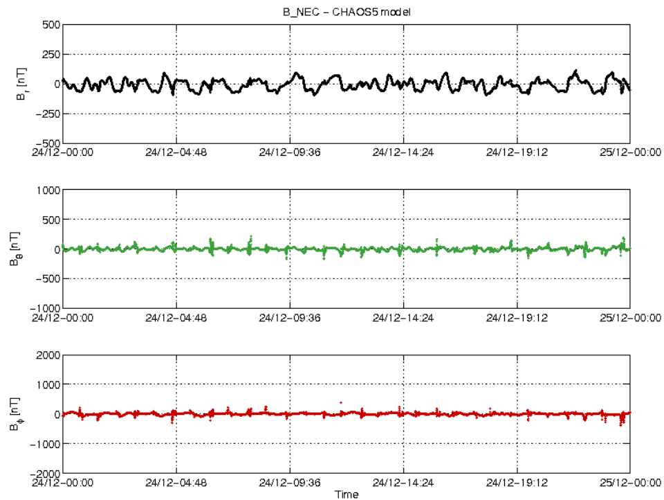
Figure 3-20: S/C B day 24.12 time series of B_{NEC} - B_{Chaos} residuals.
