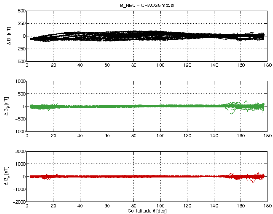
Figure 3-21: S/C C day 24.12 B_{\text{NEC}} - B_{\text{Chaos}} difference vs colatitude.
