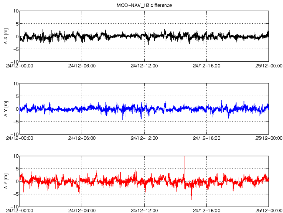
Figure 3-5: Difference MOD-GPSNAV, S/C C, 24.12. From top to bottom: X, Y and Z-axis
