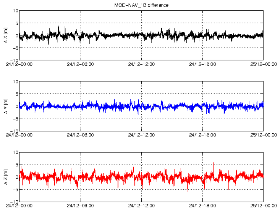
Figure 3-3: Difference MOD-GPSNAV, S/C A, 24.12. From top to bottom: X, Y and Z-axis
