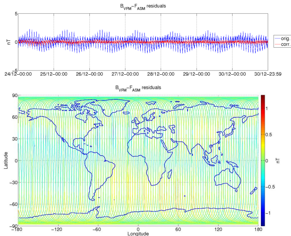
Figure 3-9: ASM-VFM residuals for S/C B, during monitoring period 24/12-30/12. In top figure are plotted: difference between |B_{VFM}| and F_{ASM} (without dB_Sun correction) (blue colour), and the residuals with dB_Sun corrections (red colour). In bottom figure residuals are presented on the world map.
