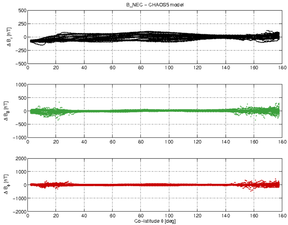
Figure 3-19: S/C B day 10.12 B_{NEC} - B_{Chaos} difference vs colatitude.
