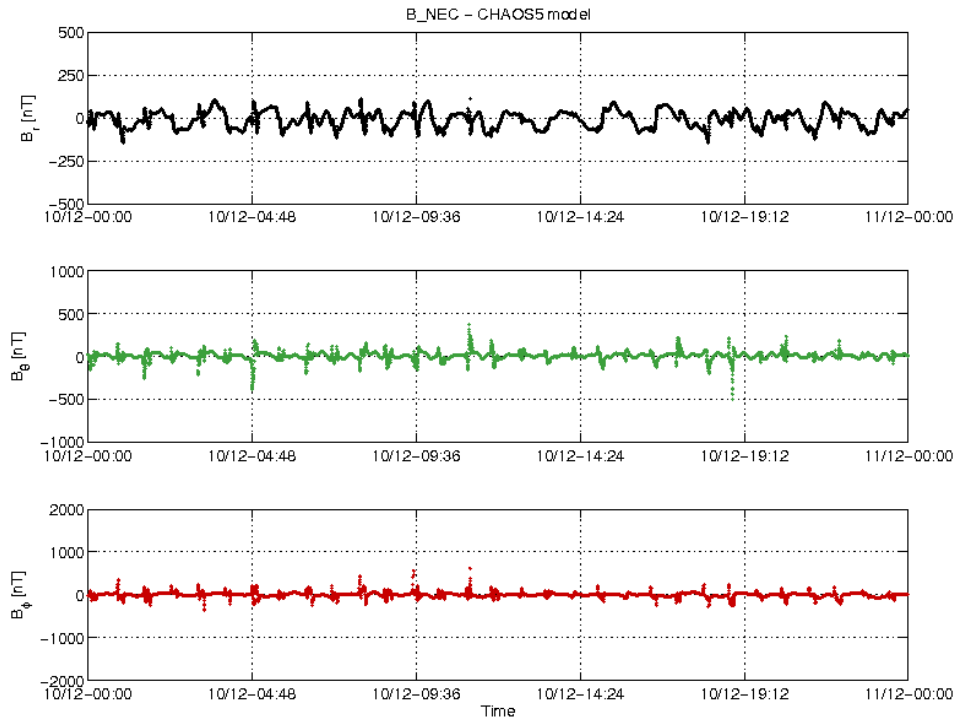
Figure 3-18: S/C A day 10.12: time series of B_{NEC} - B_{Chaos} residuals.
