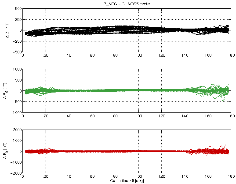
Figure 3-21: S/C C day 10.12 B_{NEC} - B_{Chaos} difference vs colatitude.
