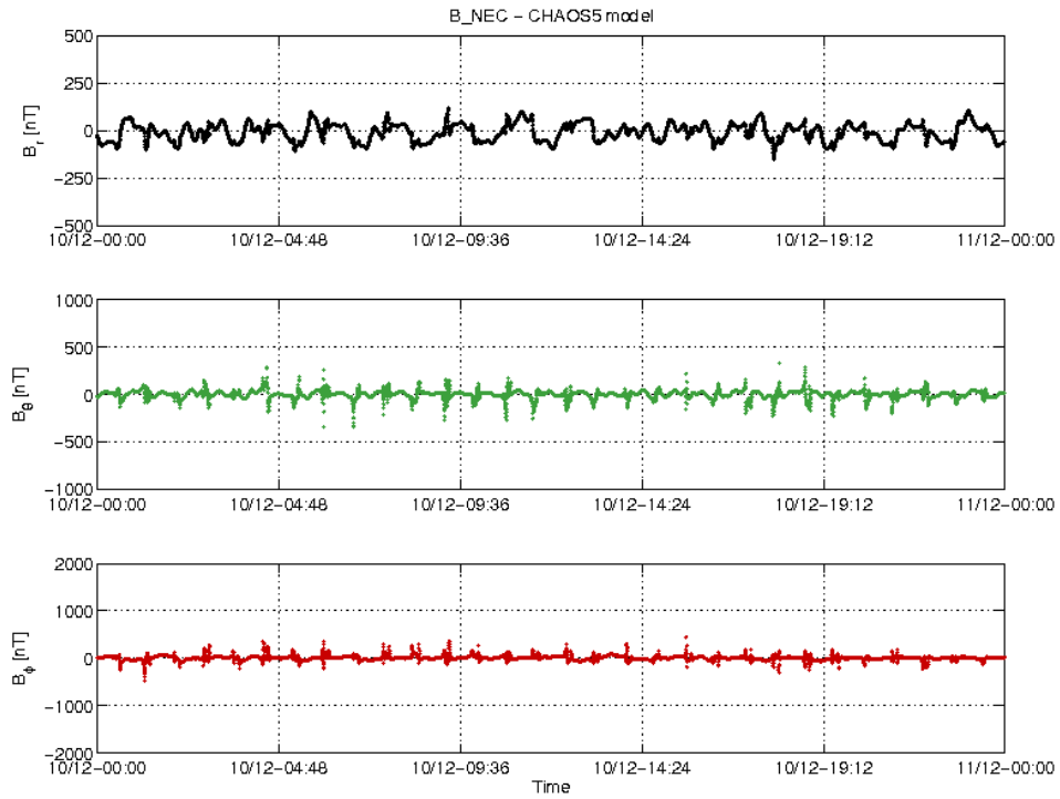
Figure 3-20: S/C B day 10.12 time series of B_{NEC} - B_{Chaos} residuals.
