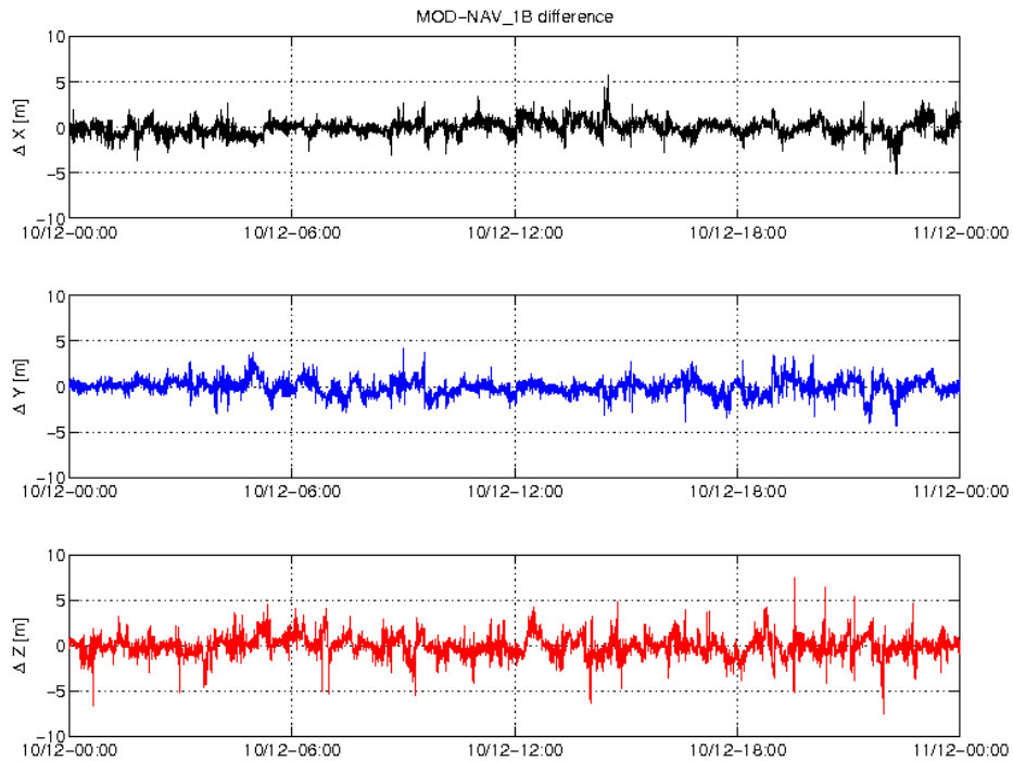
Figure 3-4: Difference MOD-GPSNAV, S/C B, 10.12. From top to bottom: X, Y and Z-axis
