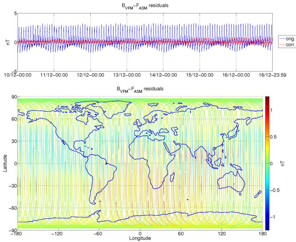
Figure 3-8: ASM-VFM residuals for S/C A, during monitoring period 10/12-16/12. In top figure are plotted: difference between |B VFM | and F ASM (without dB Sun correction) (blue colour), and the residuals with dB Sun corrections (red colour). In bottom figure residuals are presented on the world map.
