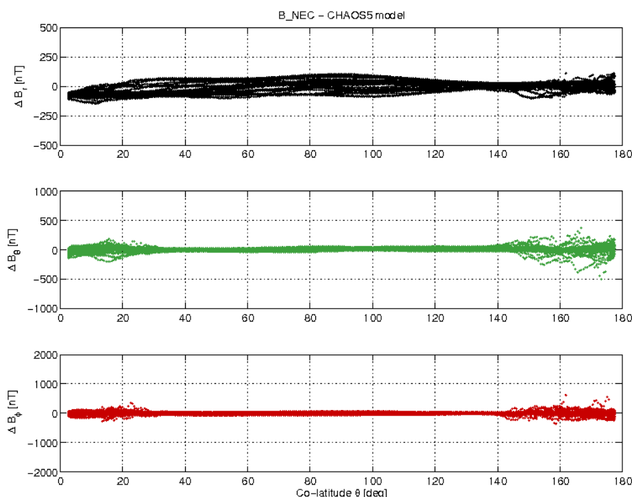
Figure 3-17: S/C A day 10.12 B_{NEC} - B_{Chaos} vs colatitude.
