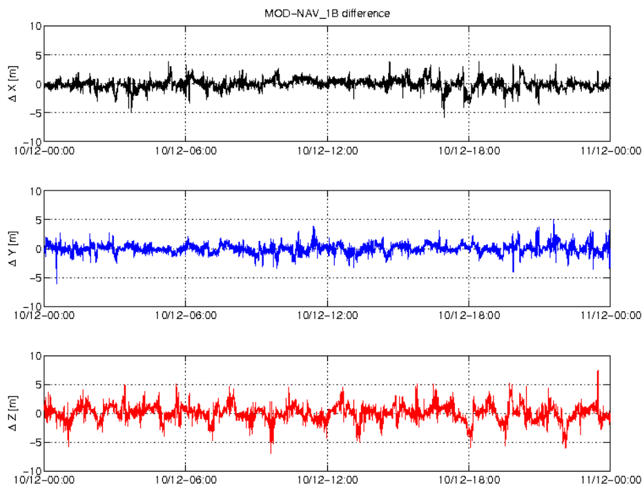
Figure 3-5: Difference MOD-GPSNAV, S/C C, 10.12. From top to bottom: X, Y and Z-axis
