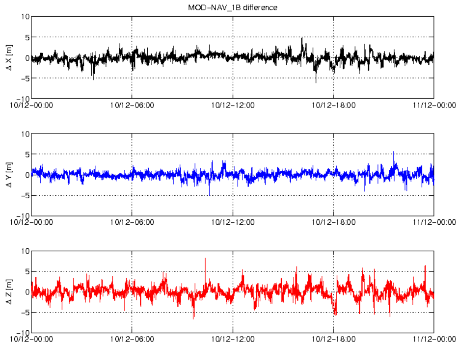
Figure 3-3: Difference MOD-GPSNAV, S/C A, 10.12. From top to bottom: X, Y and Z-axis
