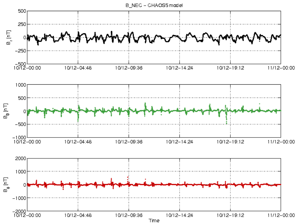
Figure 3-22: S/C C day 10.12 time series of B_{NEC} - B_{Chaos} residuals.
