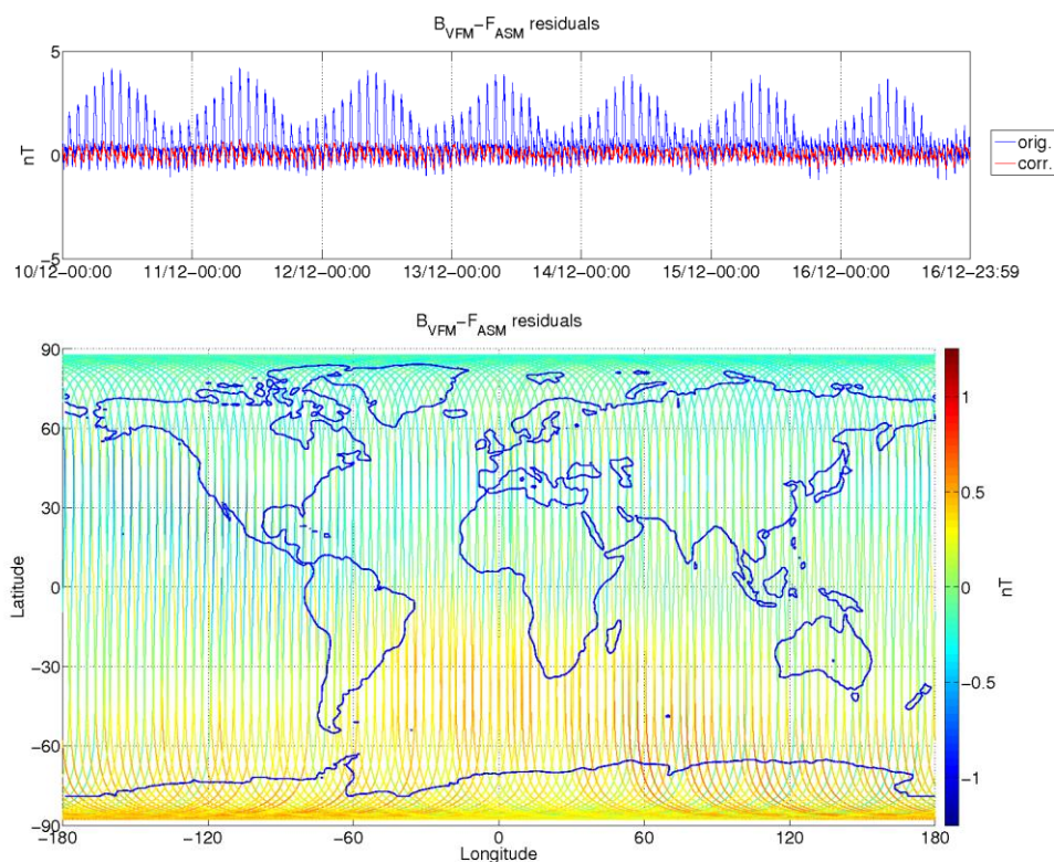
Figure 3-9: ASM-VFM residuals for S/C B, during monitoring period 10/12-16/12. In top figure are plotted: difference between |B_{VFM}| and F_{ASM} (without dB_{Sun} correction) (blue colour), and the residuals with dB_{Sun} corrections (red colour). In bottom figure residuals are presented on the world map.
