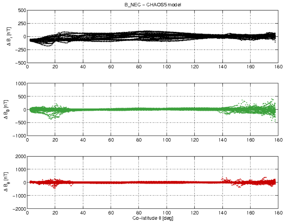
Figure 3-19: S/C B day 03.12 B_{NEC} - B_{Chaos} difference vs colatitude.
