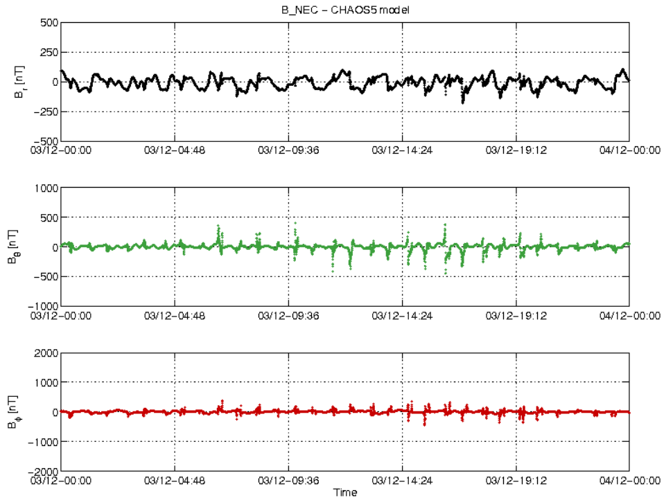
Figure 3-20: S/C B day 03.12 time series of B_{NEC} - B_{Chaos} residuals.
