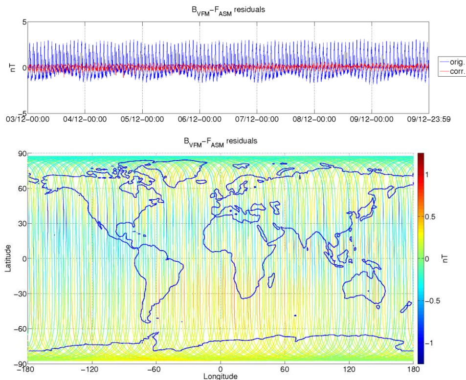
Figure 3-8: ASM-VFM residuals for S/C A, during monitoring period 03/12-09/12. In top figure are plotted: difference between |B_{VFM}| and F_{ASM} (without dB_Sun correction) (blue colour), and the residuals with dB_Sun corrections (red colour). In bottom figure residuals are presented on the world map.
