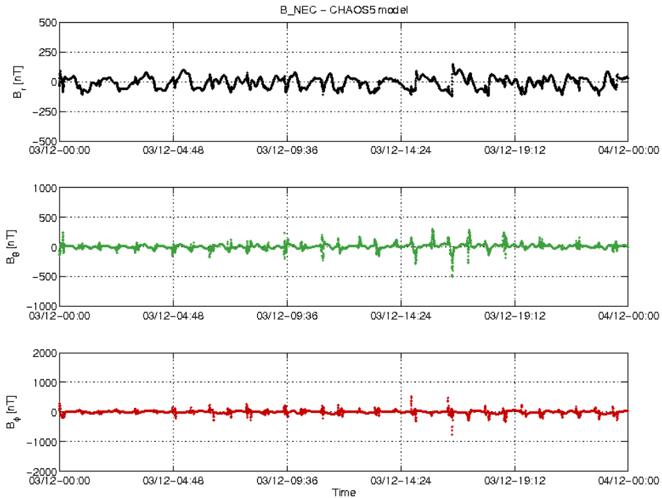
Figure 3-22: S/C C day 03.12 time series of B_{NEC} - B_{Chaos} residuals.
