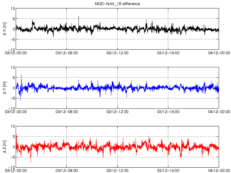
Figure 3-3: Difference MOD-GPSNAV, S/C A, 03.12. From top to bottom: X, Y and Z-axis
