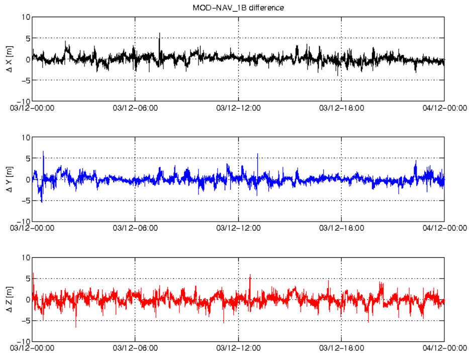
Figure 3-5: Difference MOD-GPSNAV, S/C C, 03.12. From top to bottom: X, Y and Z-axis
