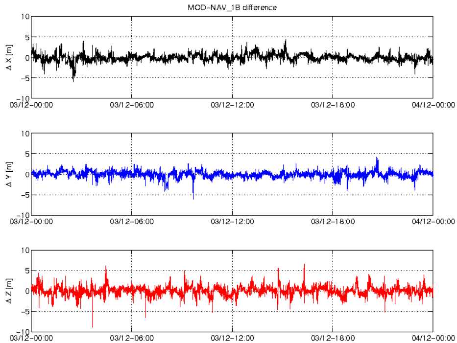
Figure 3-4: Difference MOD-GPSNAV, S/C B, 03.12. From top to bottom: X, Y and Z-axis
