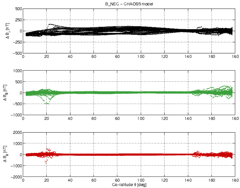
Figure 3-21: S/C C day 03.12 B_{NEC} - B_{Chaos} difference vs colatitude.
