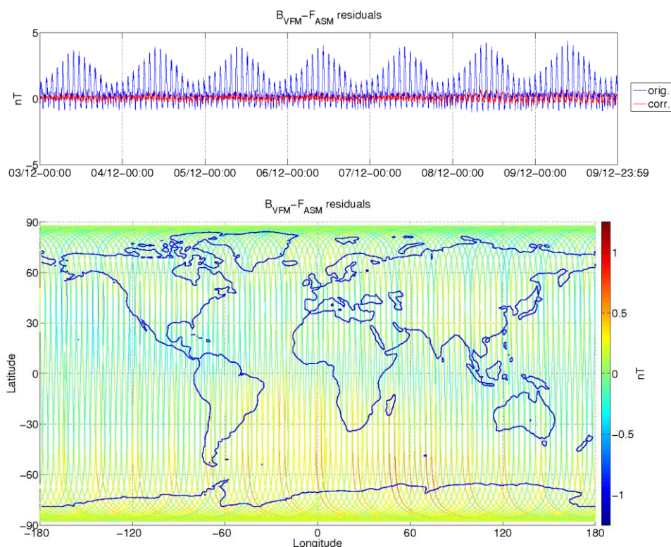
Figure 3-9: ASM-VFM residuals for S/C B, during monitoring period 03/12-09/12. In top figure are plotted: difference between |B_{VFM}| and F_{ASM} (without dB Sun correction) (blue colour), and the residuals with dB Sun corrections (red colour). In bottom figure residuals are presented on the world map.
