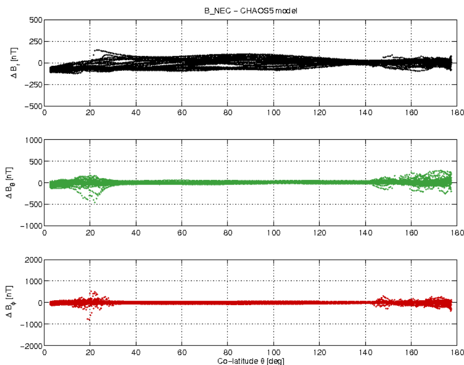
Figure 3-17: S/C A day 03.12 B_{NEC} - B_{Chaos} vs colatitude.
