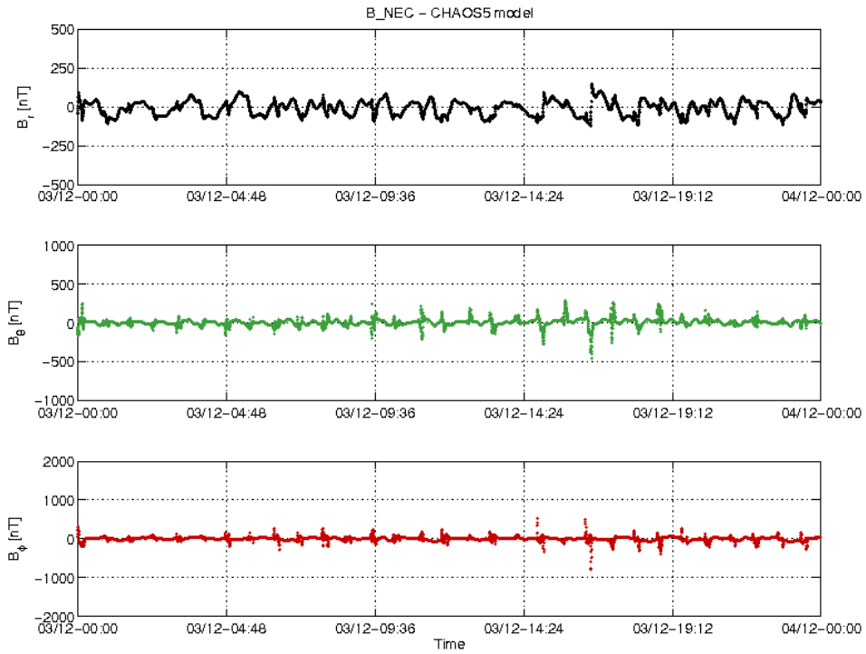
Figure 3-18: S/C A day 03.12: time series of B_{NEC} - B_{Chaos} residuals.
