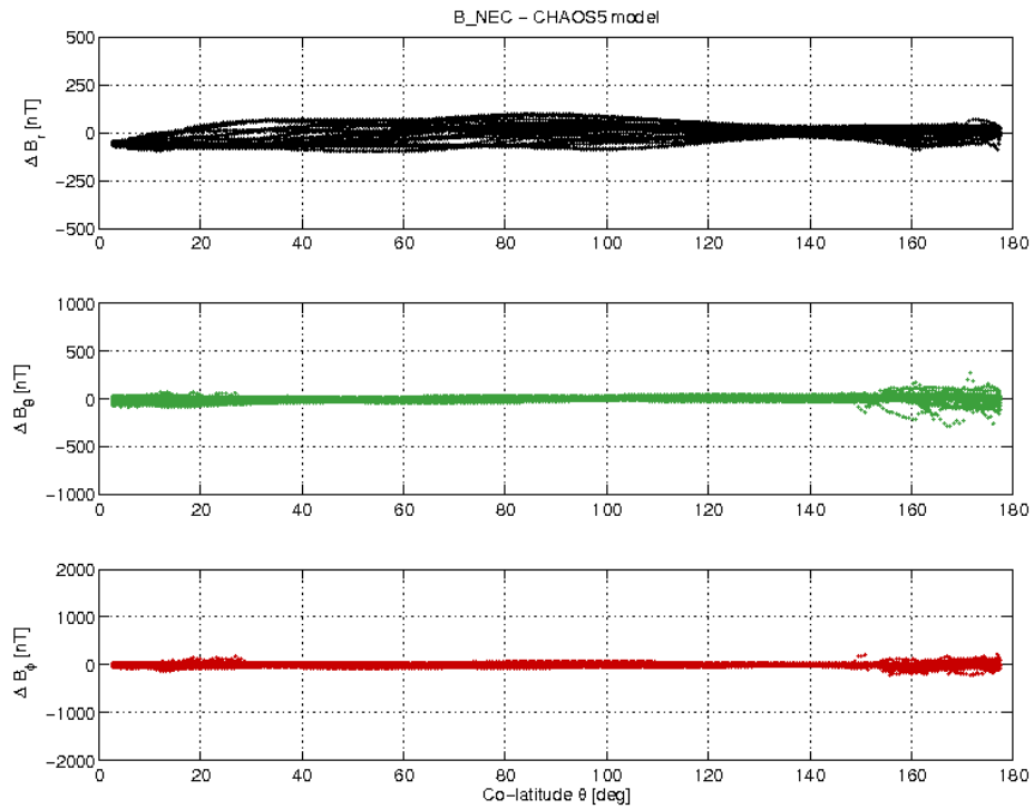
Figure 3-21: S/C C day 26.11 B_{NEC} - B_{Chaos} difference vs colatitude.
