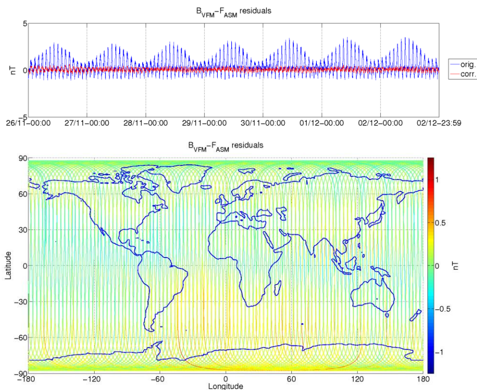
Figure 3-9: ASM-VFM residuals for S/C B, during monitoring period 26/11-02/12. In top figure are plotted: difference between |B_{VFM}| and F_{ASM} (without dB Sun correction) (blue colour), and the residuals with dB Sun corrections (red colour). In bottom figure residuals are presented on the world map.
