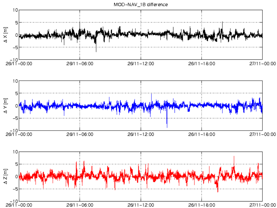
Figure 3-3: Difference MOD-GPSNAV, S/C A, 26.11. From top to bottom: X, Y and Z-axis
