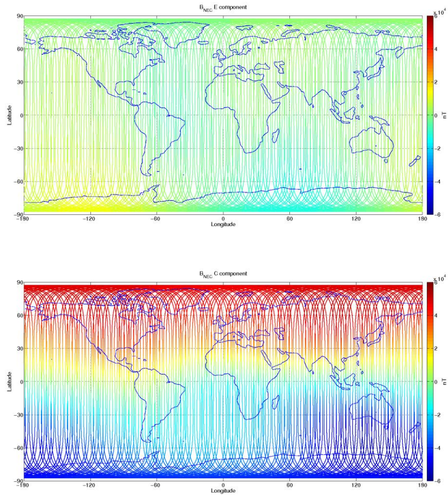
Figure 3-10: S/C A, world map plots of the geomagnetic field and components measured during monitoring period 26/11-02/12. From top to bottom: F-magnetic field from ASM measurement, B_{NEC} components (North, East, and Centre) of magnetic field from VFM measurement.
