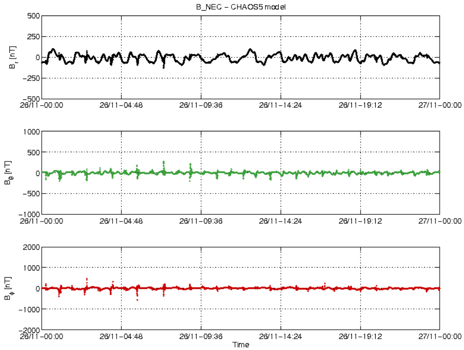
Figure 3-20: S/C B day 26.11 time series of B_{NEC} - B_{Chaos} residuals.
