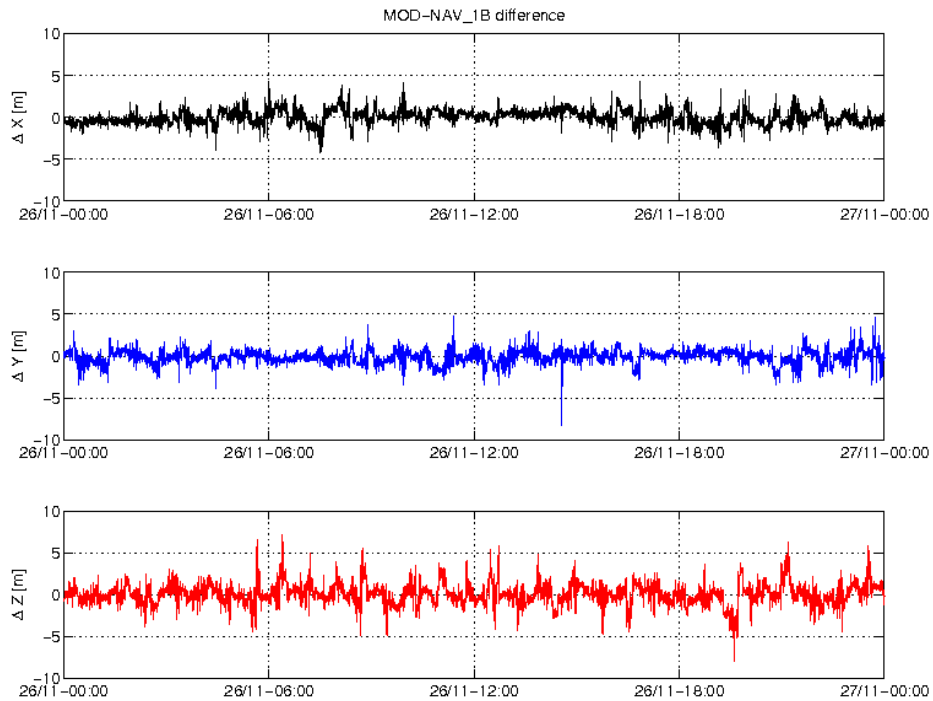
Figure 3-5: Difference MOD-GPSNAV, S/C C, 26.11. From top to bottom: X, Y and Z-axis
