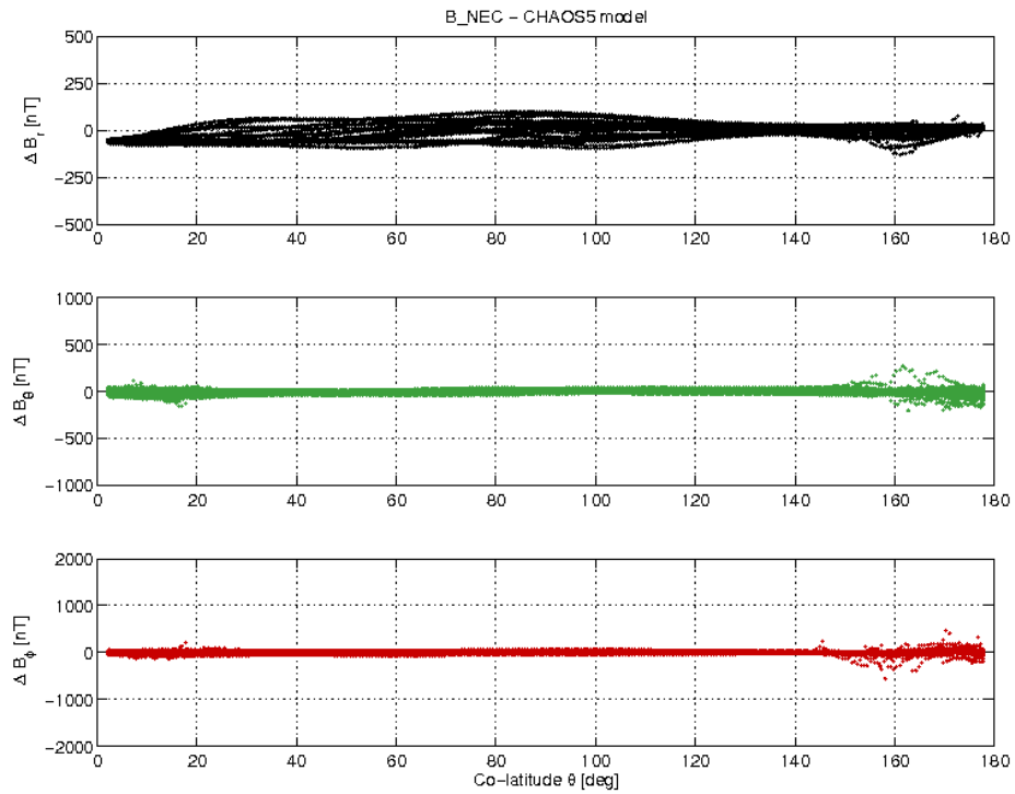
Figure 3-19: S/C B day 26.11 B_{NEC} - B_{Chaos} difference vs colatitude.
