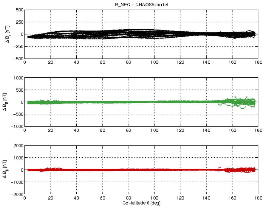
Figure 3-17: S/C A day 26.11 B_{NEC} - B_{Chaos} vs colatitude.
