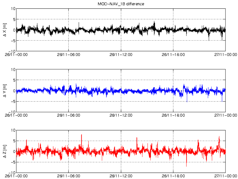
Figure 3-4: Difference MOD-GPSNAV, S/C B, 26.11. From top to bottom: X, Y and Z-axis
