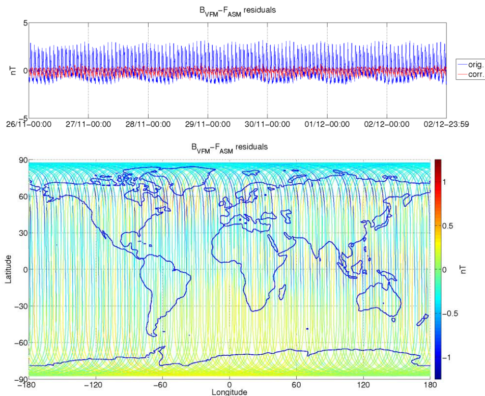
Figure 3-8: ASM-VFM residuals for S/C A, during monitoring period 26/11-02/12. In top figure are plotted: difference between |B_{VFM}| and F_{ASM} (without dB_{Sun} correction) (blue colour), and the residuals with dB_{Sun} corrections (red colour). In bottom figure residuals are presented on the world map.
