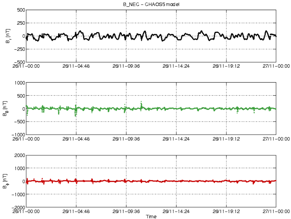
Figure 3-22: S/C C day 26.11 time series of B_{NEC} - B_{Chaos} residuals.
