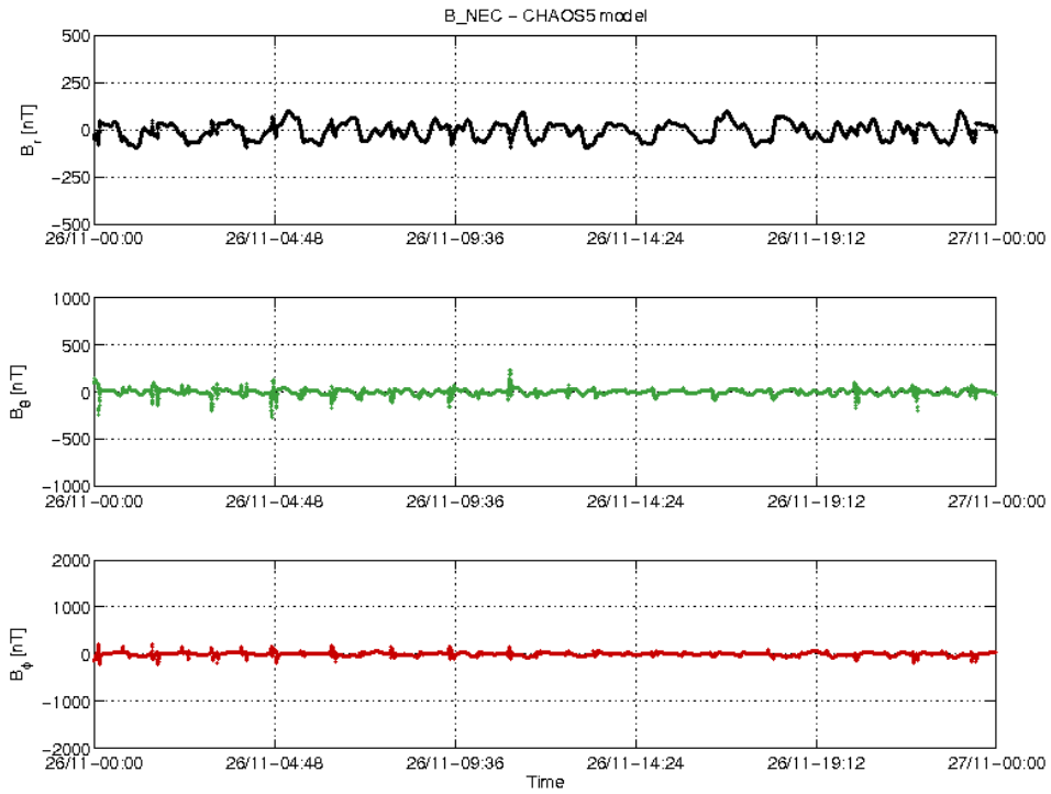
Figure 3-18: S/C A day 26.11: time series of B_{NEC} - B_{Chaos} residuals.
