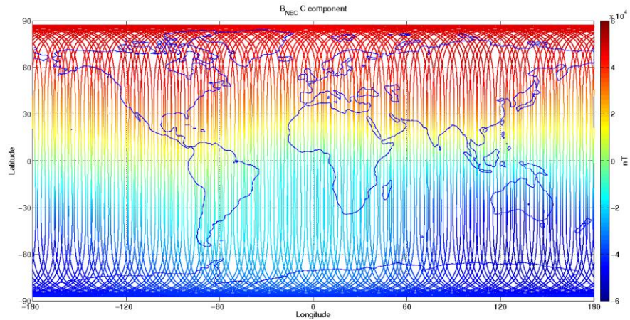
Figure 3-12: S/C C, world map plots of the geomagnetic field and components measured during monitoring period 12/11-18/11. From top to bottom: B_{NEC} components (North, East, and Centre) of magnetic field from VFM measurement.
