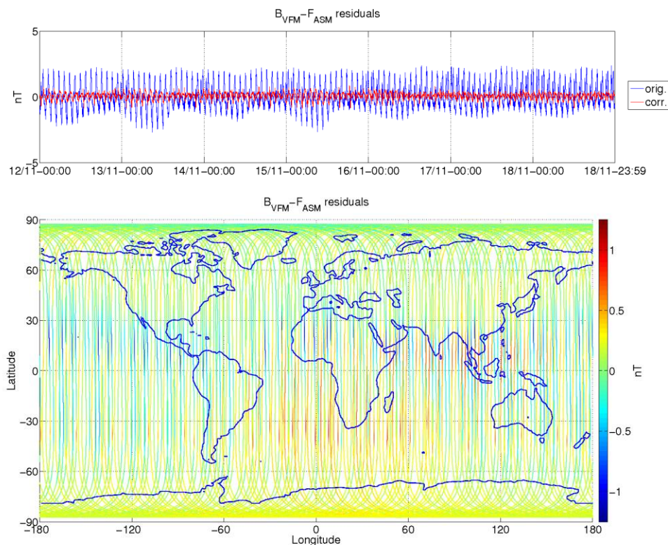
Figure 3-8: ASM-VFM residuals for S/C A, during monitoring period 12/11-18/11. In top figure are plotted: difference between |B_{VFM}| and F_{ASM} (without dB_Sun correction) (blue colour), and the
