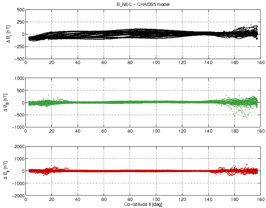
Figure 3-21: S/C C day 12.11 B_{NEC} - B_{Chaos} difference vs colatitude.
