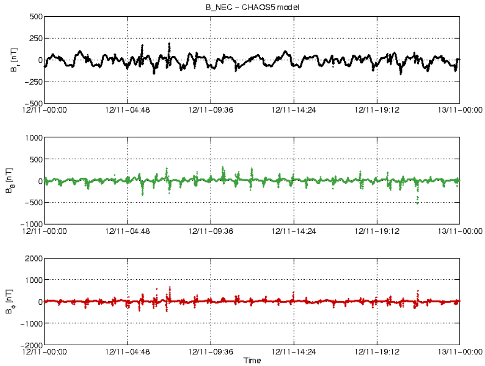
Figure 3-20: S/C B day 12.11 time series of B_{NEC} - B_{Chaos} residuals.
