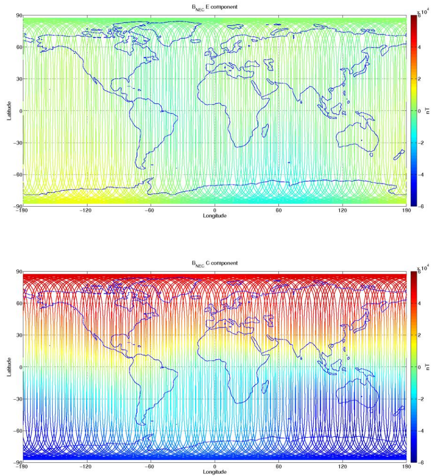
Figure 3-10: S/C A, world map plots of the geomagnetic field and components measured during monitoring period 12/11-18/11. From top to bottom: F-magnetic field from ASM measurement, B NEC components (North, East, and Centre) of magnetic field from VFM measurement.
