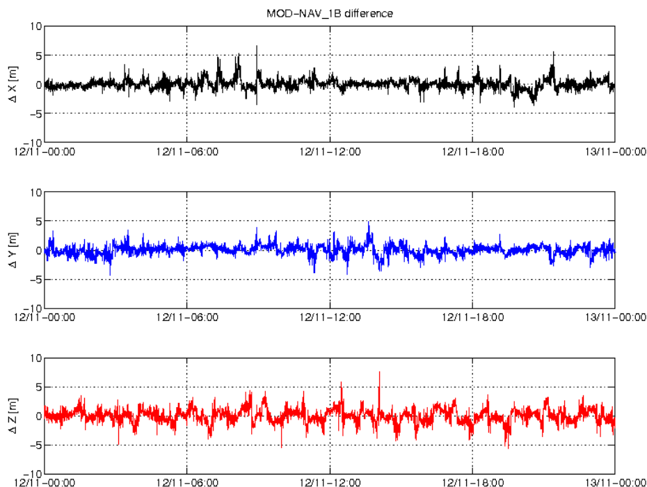
Figure 3-5: Difference MOD-GPSNAV, S/C C, 12.11. From top to bottom: X, Y and Z-axis
