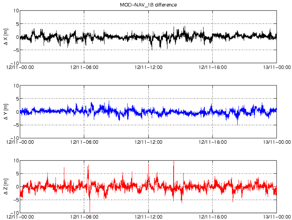
Figure 3-4: Difference MOD-GPSNAV, S/C B, 12.11. From top to bottom: X, Y and Z-axis
