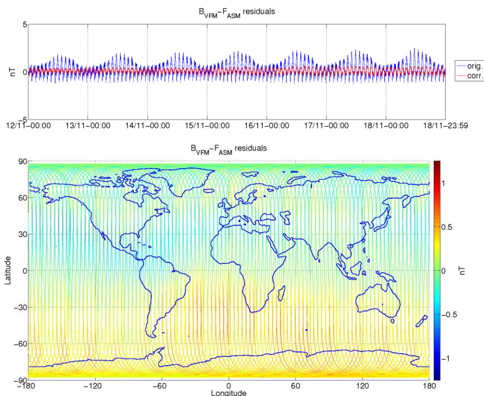
Figure 3-9: ASM-VFM residuals for S/C B, during monitoring period 12/11-18/11. In top figure are plotted: difference between |B_{VFM}| and F_{ASM} (without dB_Sun correction) (blue colour), and the residuals with dB_Sun corrections (red colour). In bottom figure residuals are presented on the world map.
