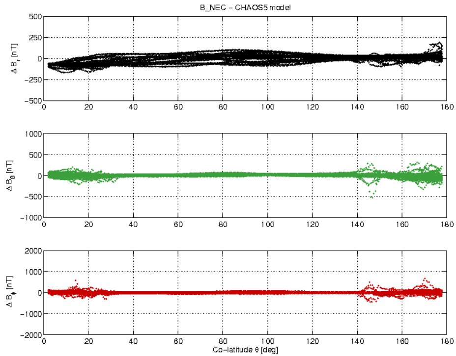
Figure 3-19: S/C B day 12.11 B_{NEC} - B_{Chaos} difference vs colatitude.
