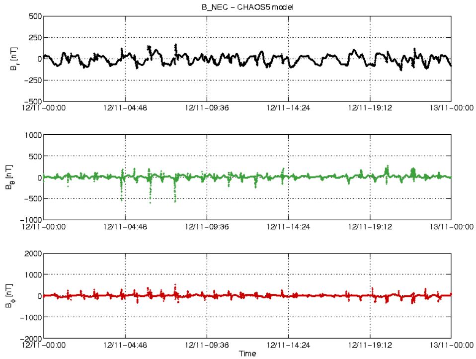
Figure 3-18: S/C A day 12.11: time series of B_{NEC} - B_{Chaos} residuals.
