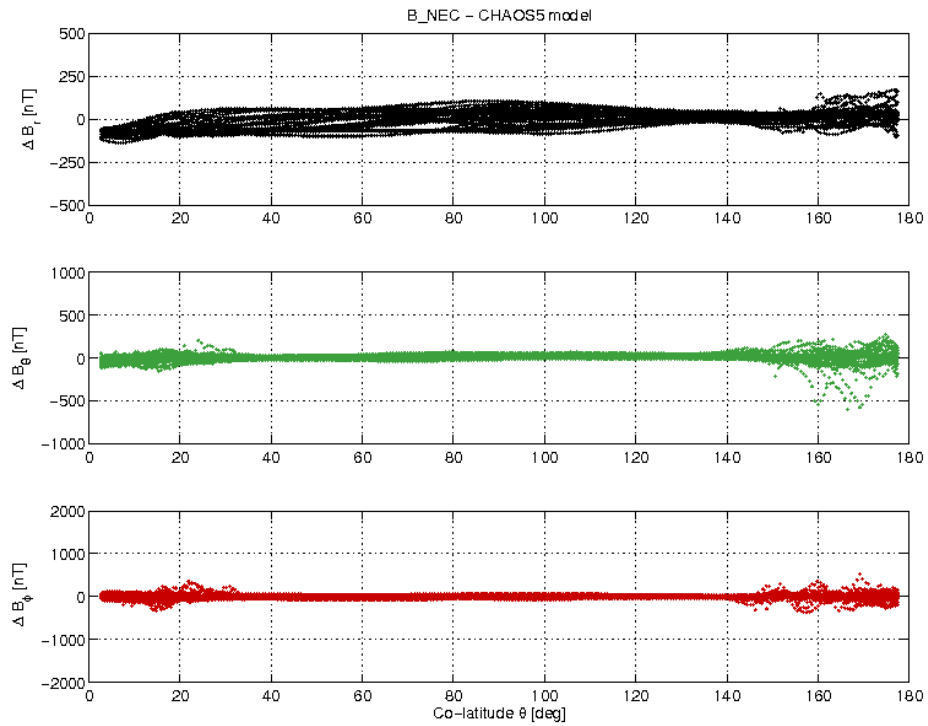
Figure 3-17: S/C A day 12.11 B_{NEC} - B_{Chaos} vs colatitude.
