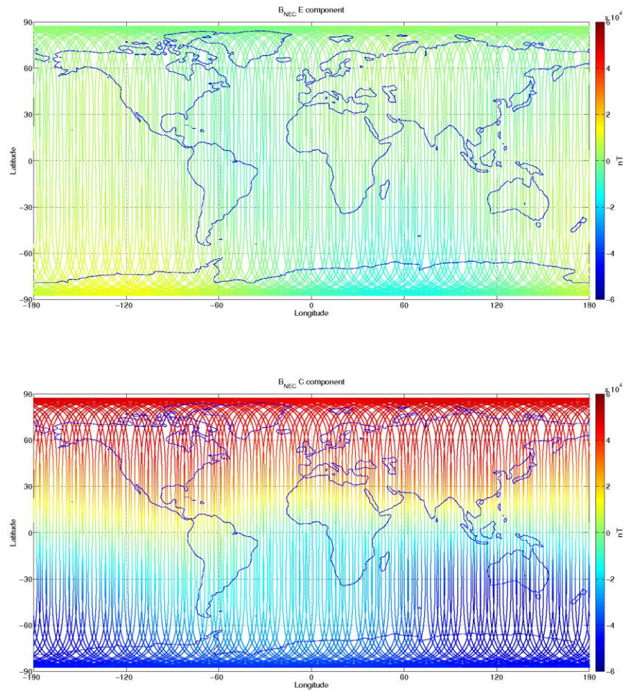
Figure 3-10: S/C A, world map plots of the geomagnetic field and components measured during monitoring period 05/11-11/11. From top to bottom: F-magnetic field from ASM measurement, B_{NEC} components (North, East, and Centre) of magnetic field from VFM measurement.
