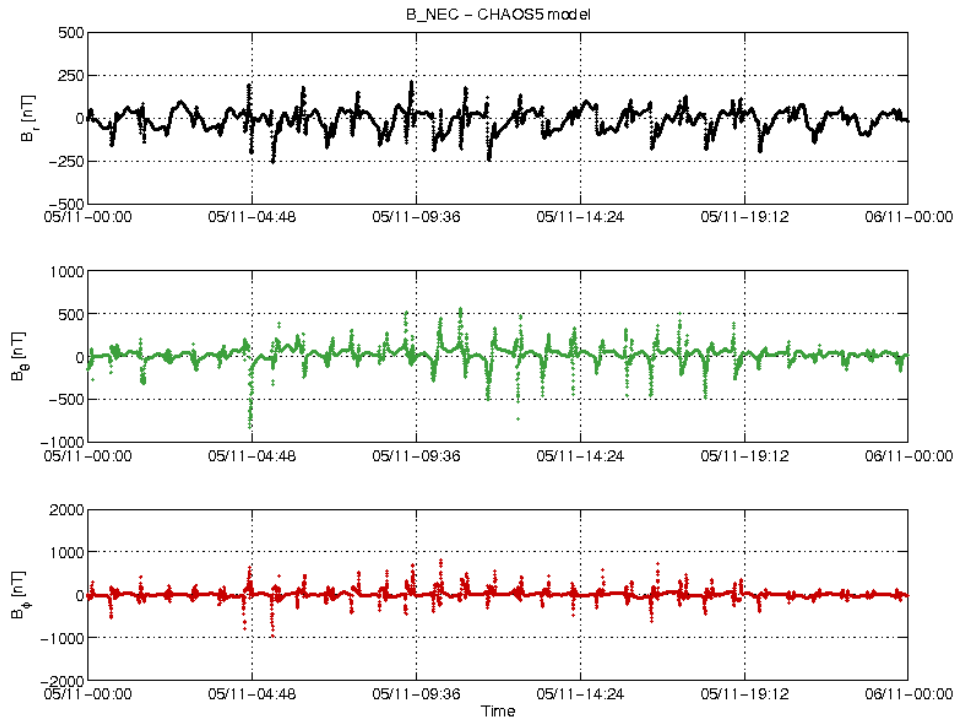
Figure 3-20: S/C B day 05.11 time series of B_{NEC} - B_{Chaos} residuals.
