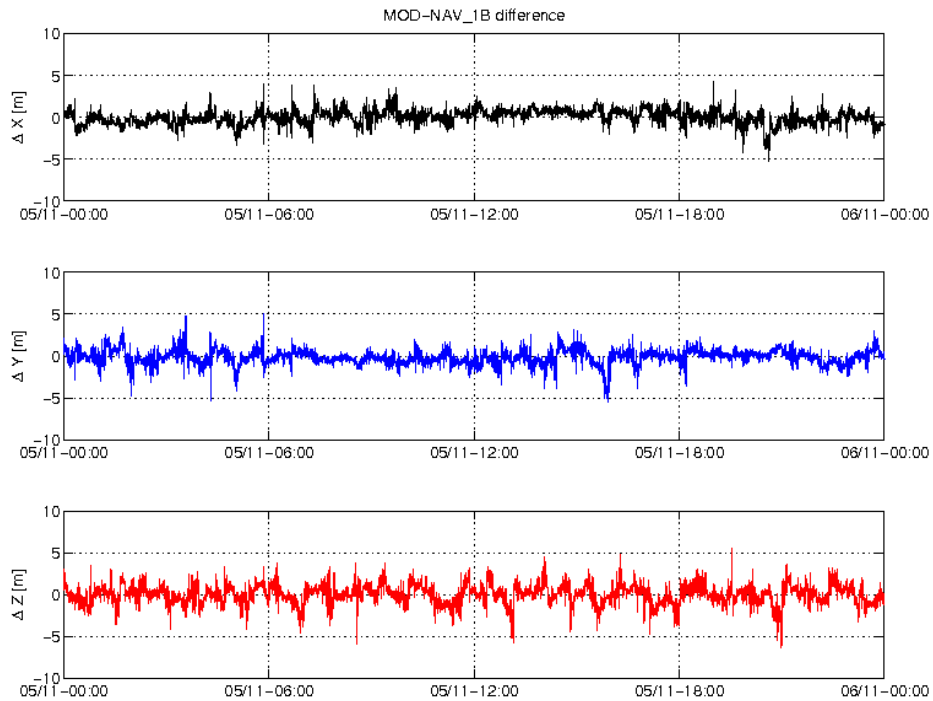
Figure 3-5: Difference MOD-GPSNAV, S/C C, 05.11. From top to bottom: X, Y and Z-axis
