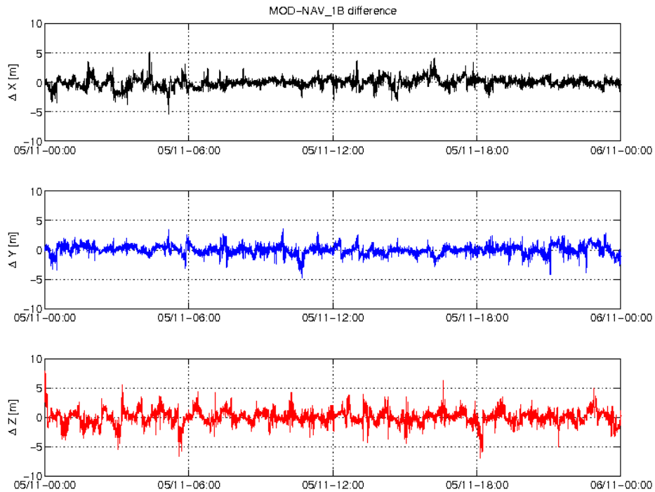
Figure 3-4: Difference MOD-GPSNAV, S/C B, 05.11. From top to bottom: X, Y and Z-axis
