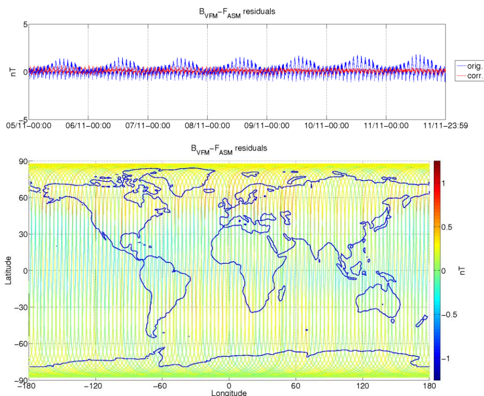
Figure 3-9: ASM-VFM residuals for S/C B, during monitoring period 05/11-11/11. In top figure are plotted: difference between |B_{VFM}| and F_{ASM} (without dB_Sun correction) (blue colour), and the residuals with dB_Sun corrections (red colour). In bottom figure residuals are presented on the world map.
