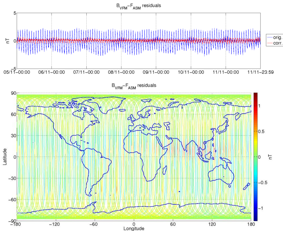
Figure 3-8: ASM-VFM residuals for S/C A, during monitoring period 05/11-11/11. In top figure are plotted: difference between |B_{VFM}| and F_{ASM} (without dB_Sun correction) (blue colour), and the
