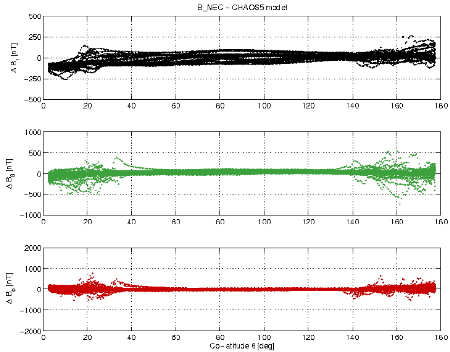
Figure 3-17: S/C A day 05.11 B_{NEC} - B_{Chaos} vs colatitude.
