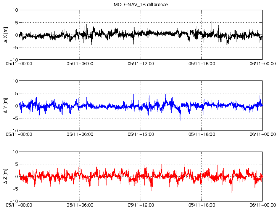
Figure 3-3: Difference MOD-GPSNAV, S/C A, 05.11. From top to bottom: X, Y and Z-axis
