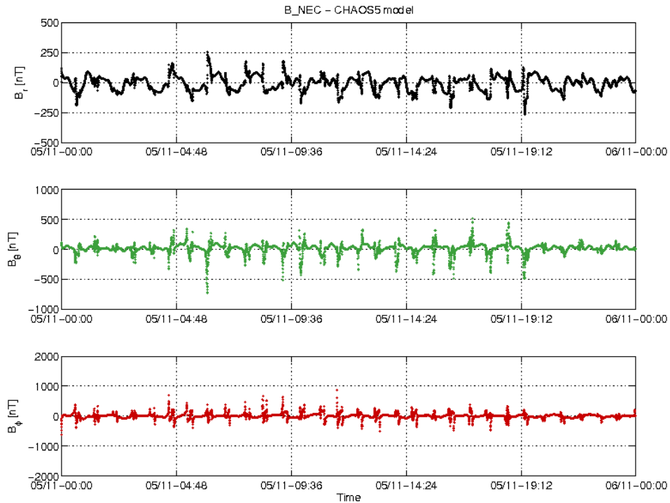
Figure 3-22: S/C C day 05.11 time series of B_{NEC} - B_{Chaos} residuals.
