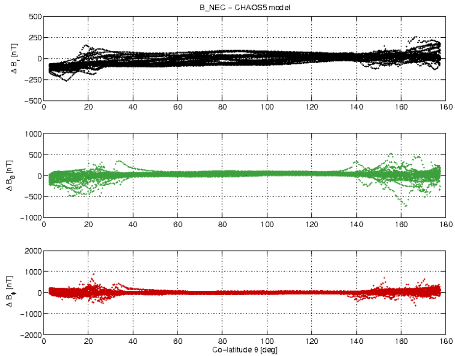
Figure 3-21: S/C C day 05.11 B_{NEC} - B_{Chaos} difference vs colatitude.
