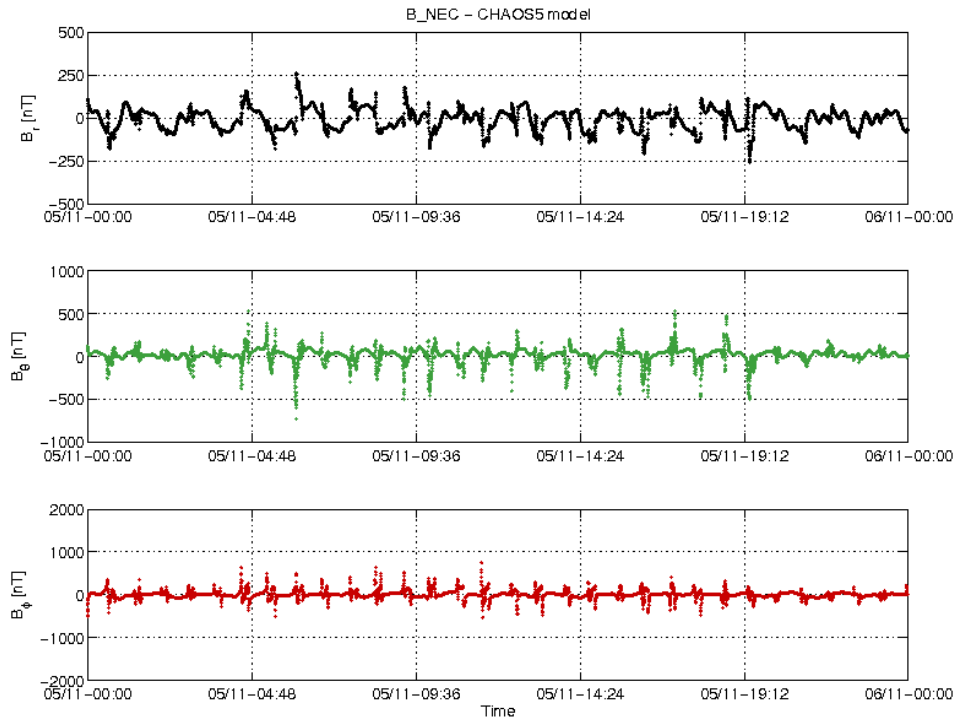
Figure 3-18: S/C A day 05.11: time series of B_{NEC} - B_{Chaos} residuals.
