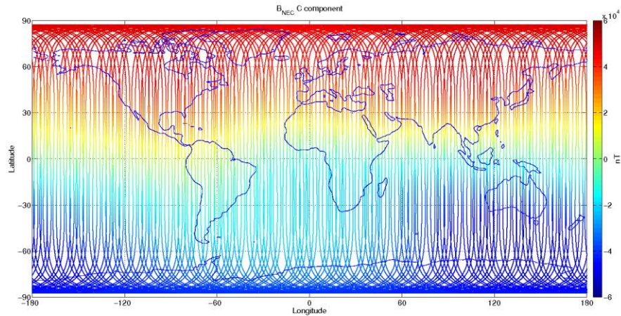
Figure 3-12: S/C C, world map plots of the geomagnetic field and components measured during monitoring period 05/11-11/11. From top to bottom: B_{NEC} components (North, East, and Centre) of magnetic field from VFM measurement.
