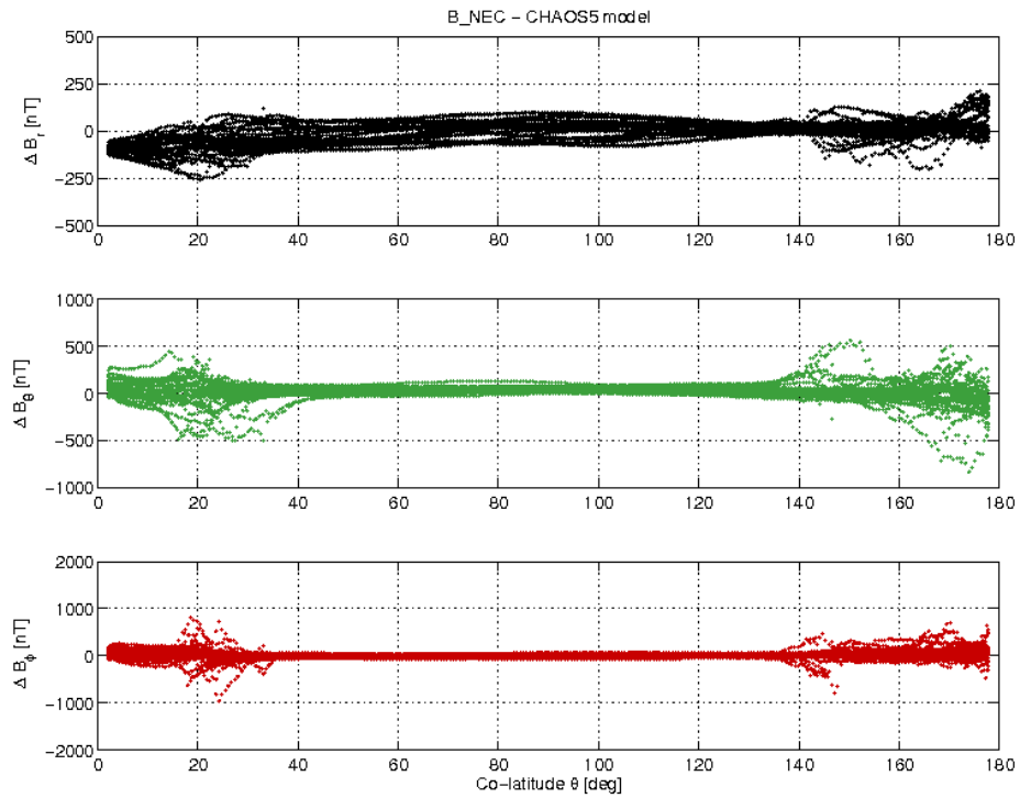
Figure 3-19: S/C B day 05.11 B_{NEC} - B_{Chaos} difference vs colatitude.
